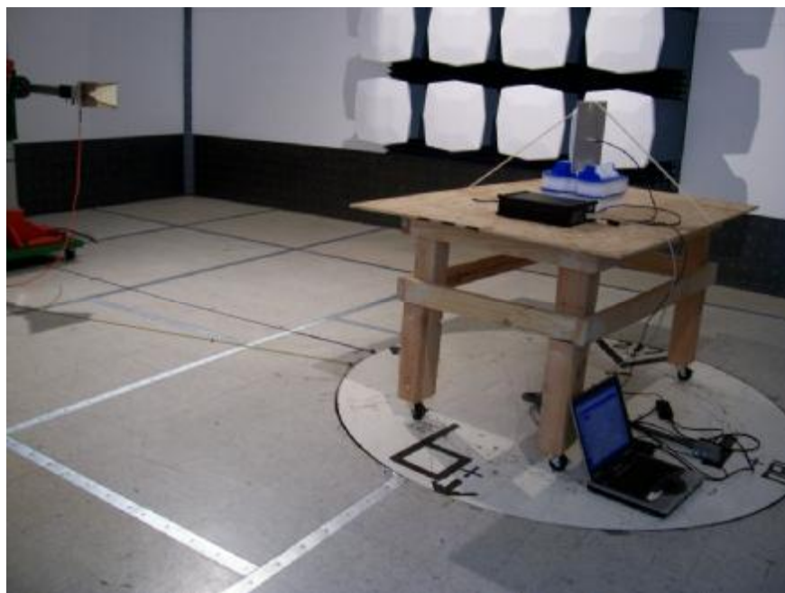
Radiated Emission setup > 1 GHz
