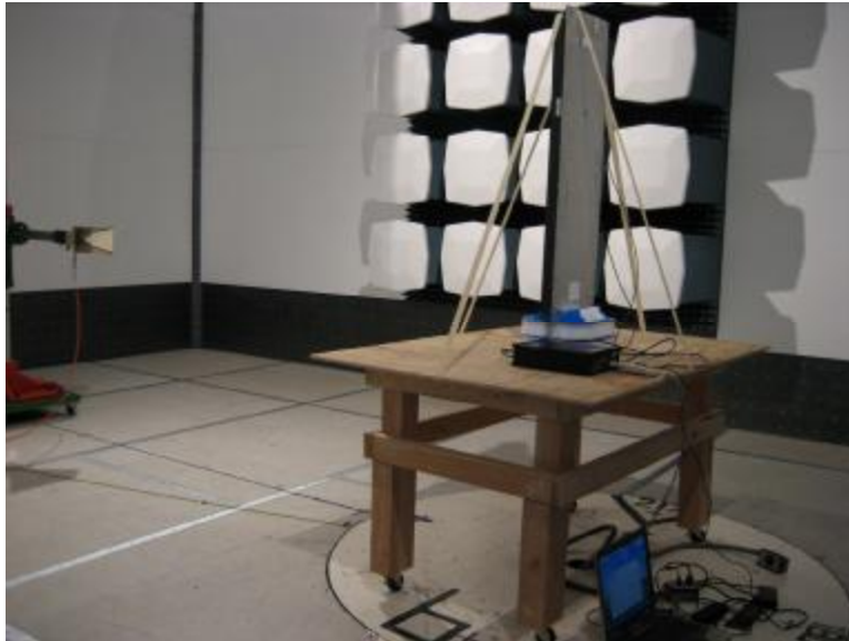
Radiated Emission setup > 1 GHz
