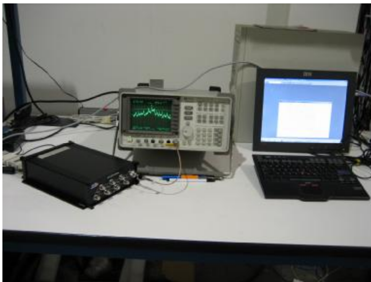
Conducted Measurement setup
