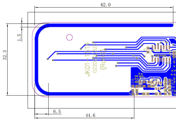
UU2022-15T4 Schematic diagram of antenna position
