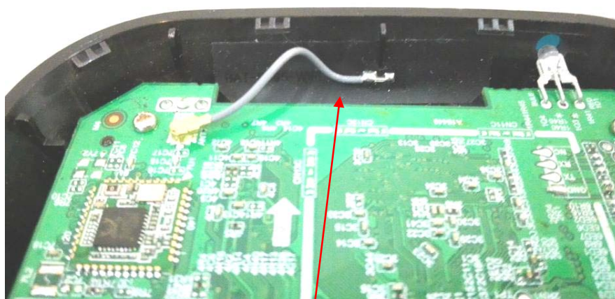
WiFi Antenna
