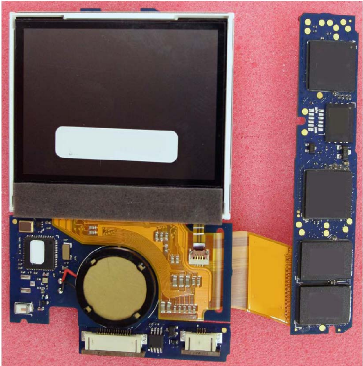
Minimed 620G PCBA Stack Opened: Top View
