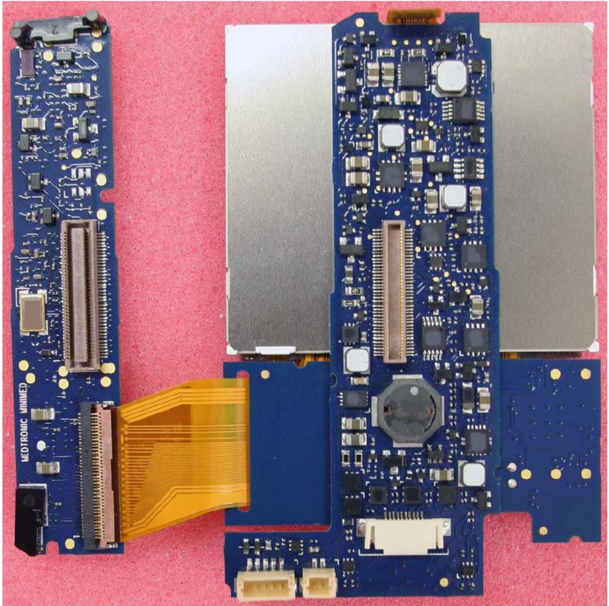
Minimed 620G PCBA Stack Opened: Bottom View
