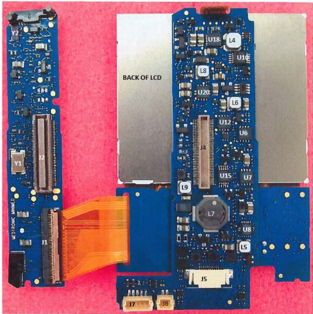
Minimed 620G Stack Opened: Bottom View
