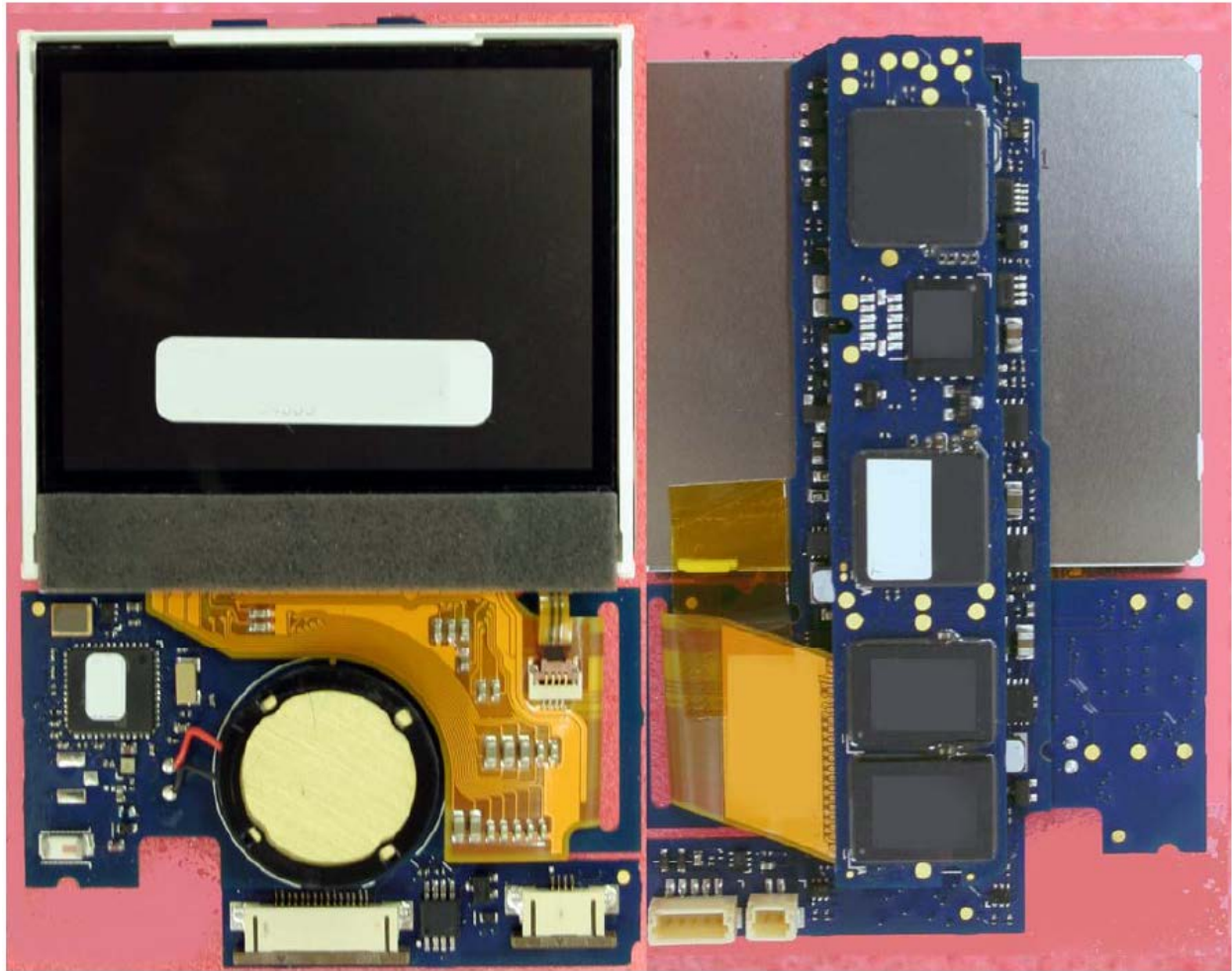
Minimed 620G PCBA Stack: Top and Bottom Views
