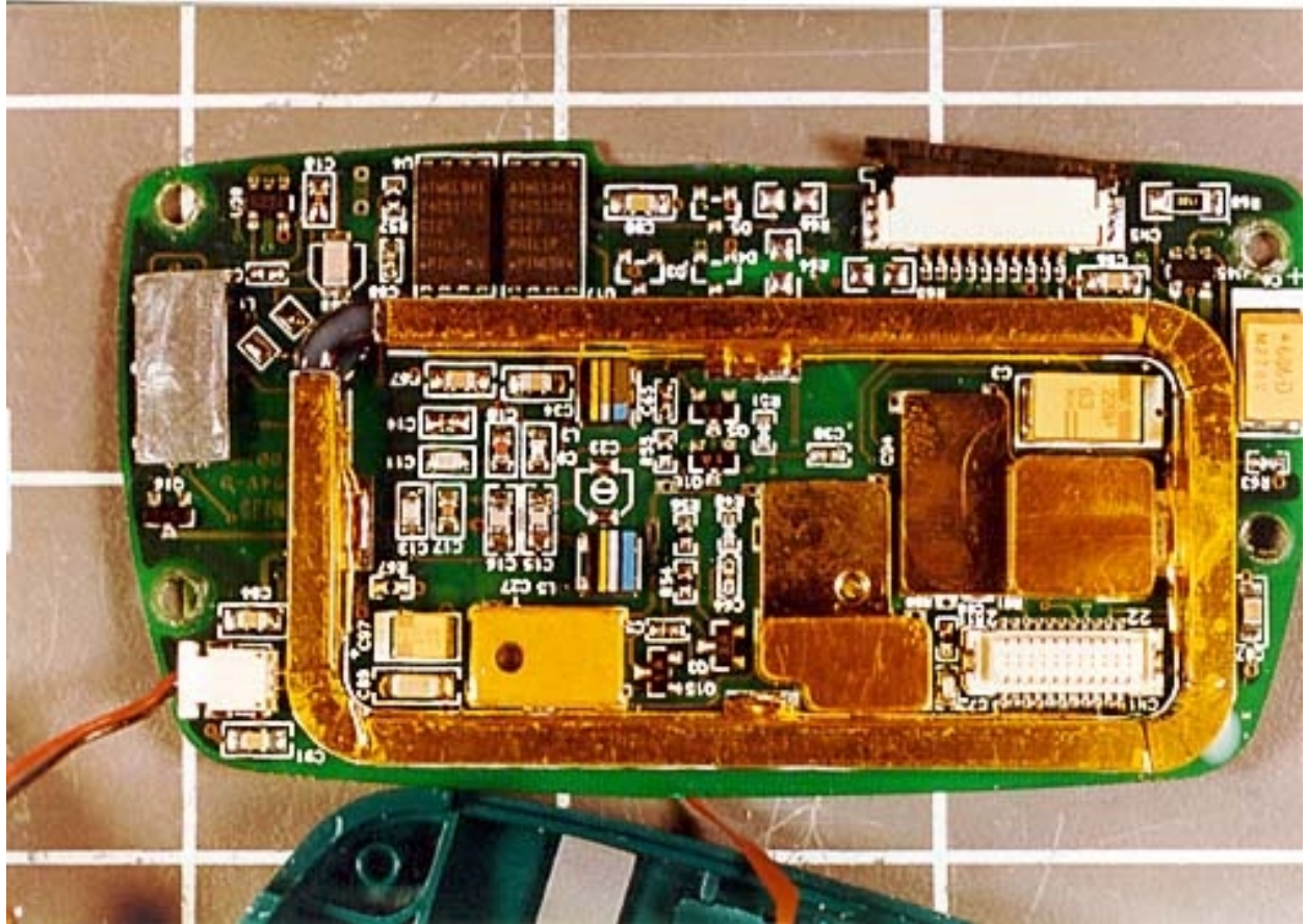
Bottom PPC RF Digital Board
