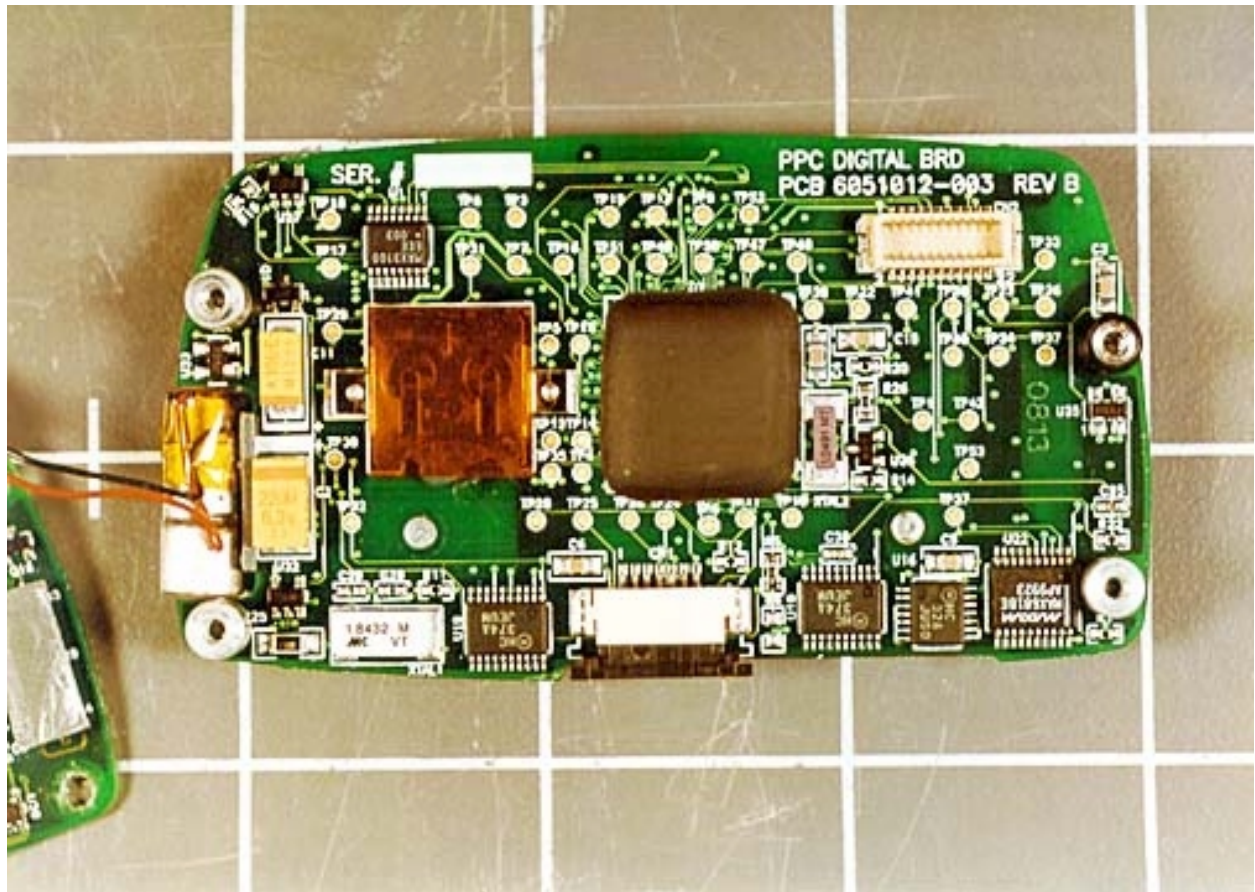
Top PPC Digital Board
