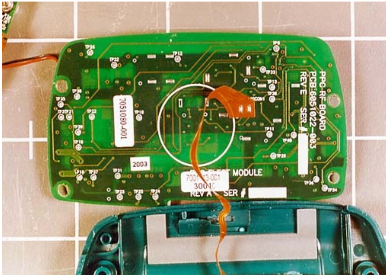
Top PPC RF Digital Board
