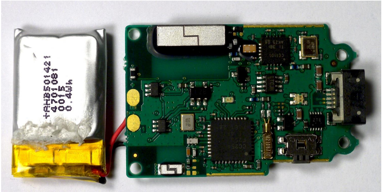
Medtronic Paradigm Translator PCBA opened: Top View
