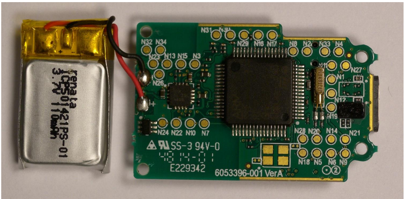
Medtronic Paradigm Translator PCBA opened: Bottom View
