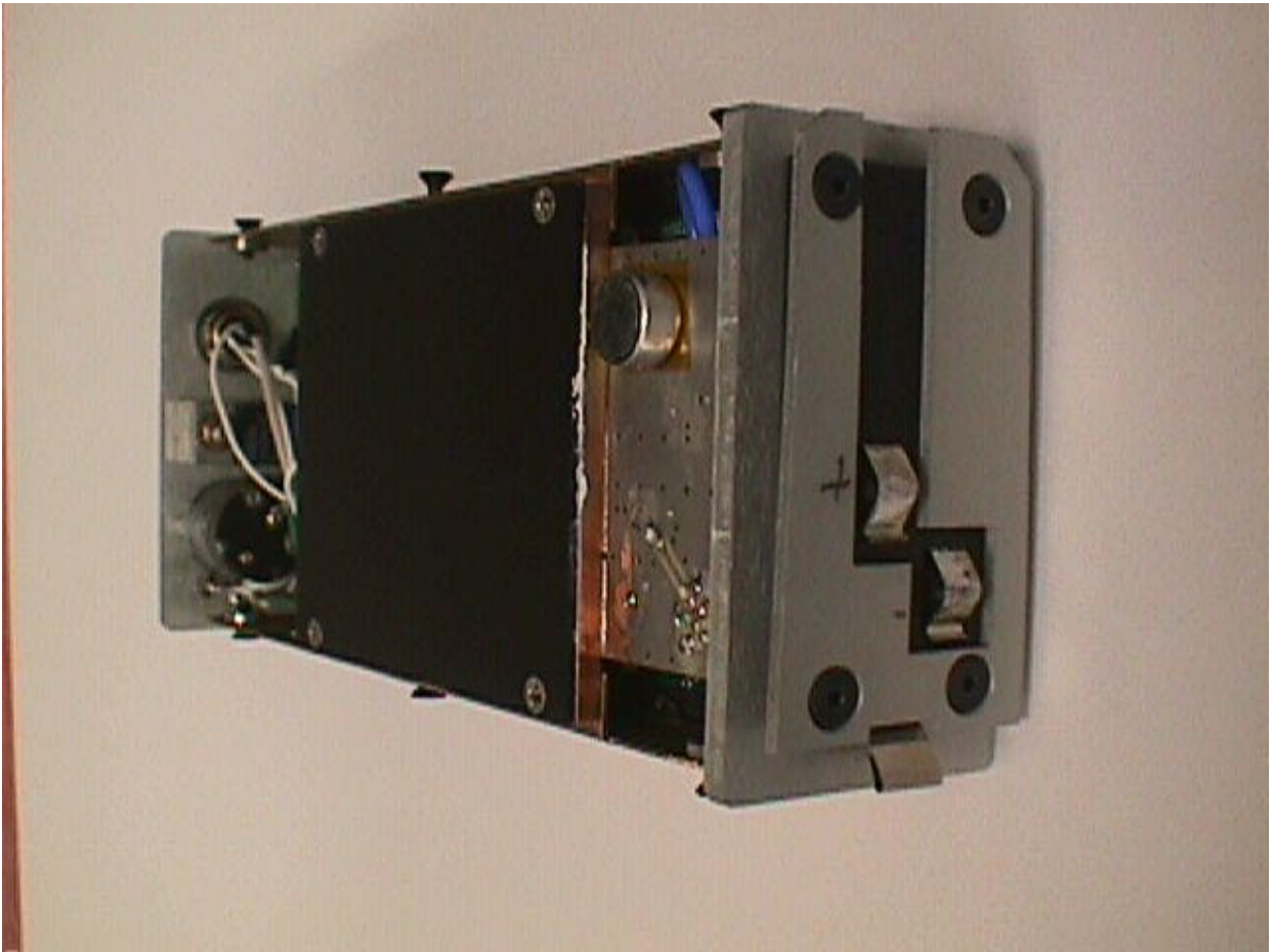
D4: TOP/BACK VIEW OF EUT WITHOUT COVER
