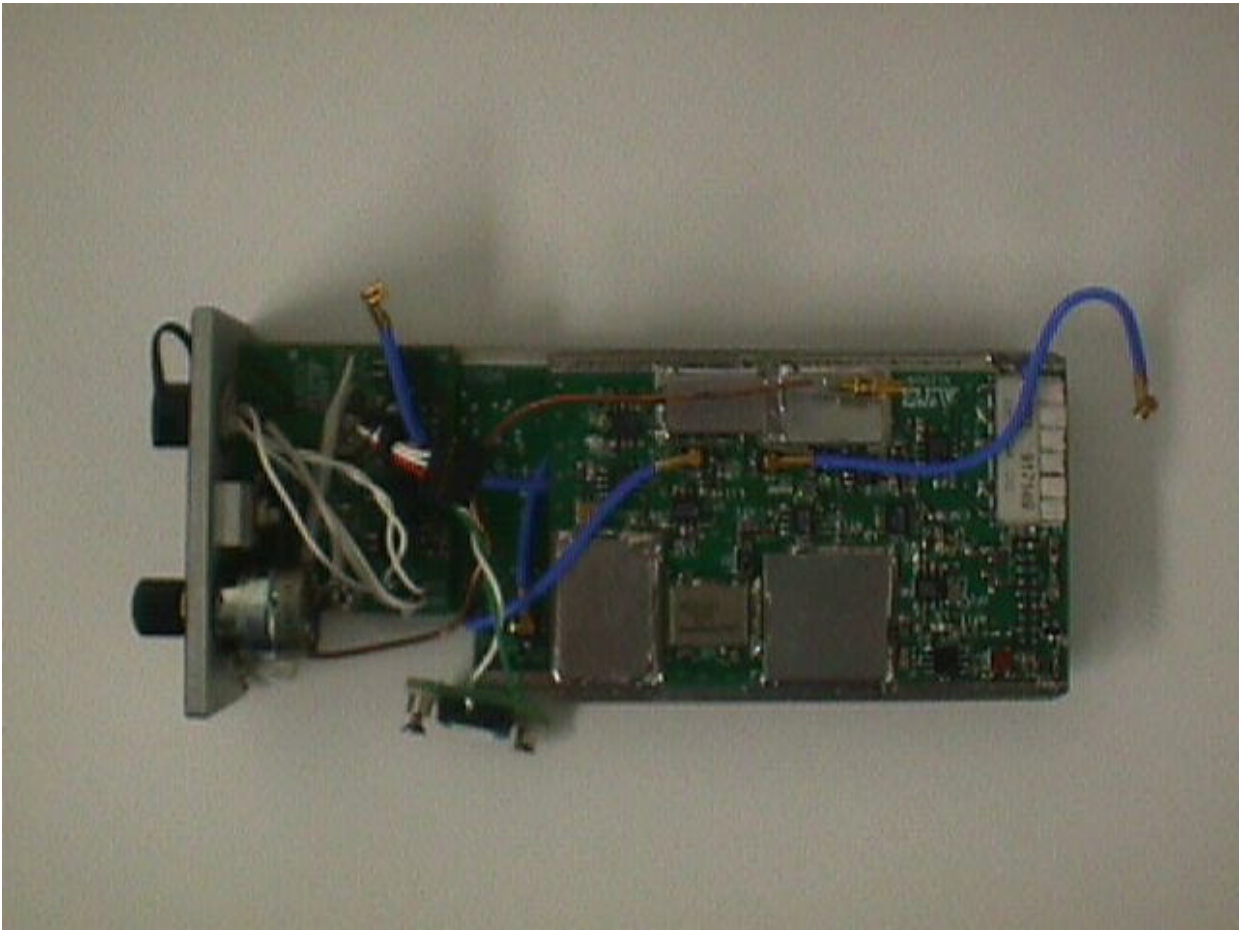
D7: TOP VIEW OF EUT WITH PCB BOARDS
