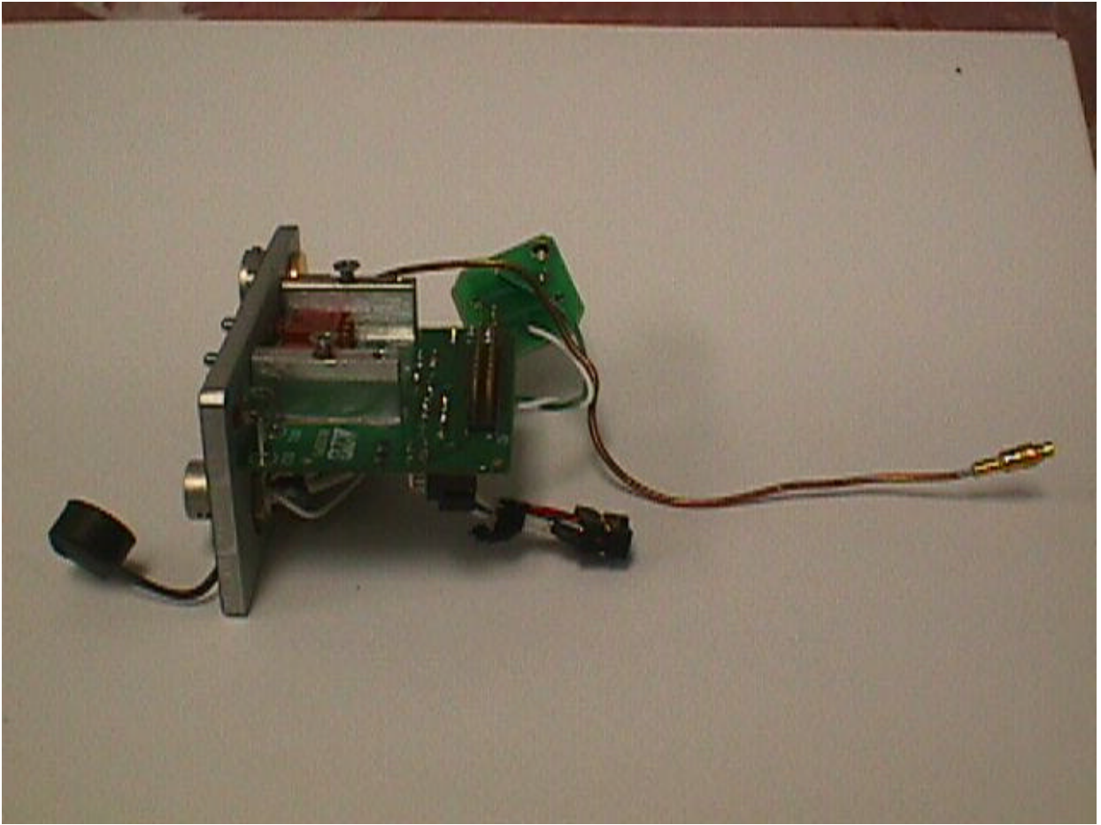
D23: SIDE VIEW OF A1225PS BOARD
