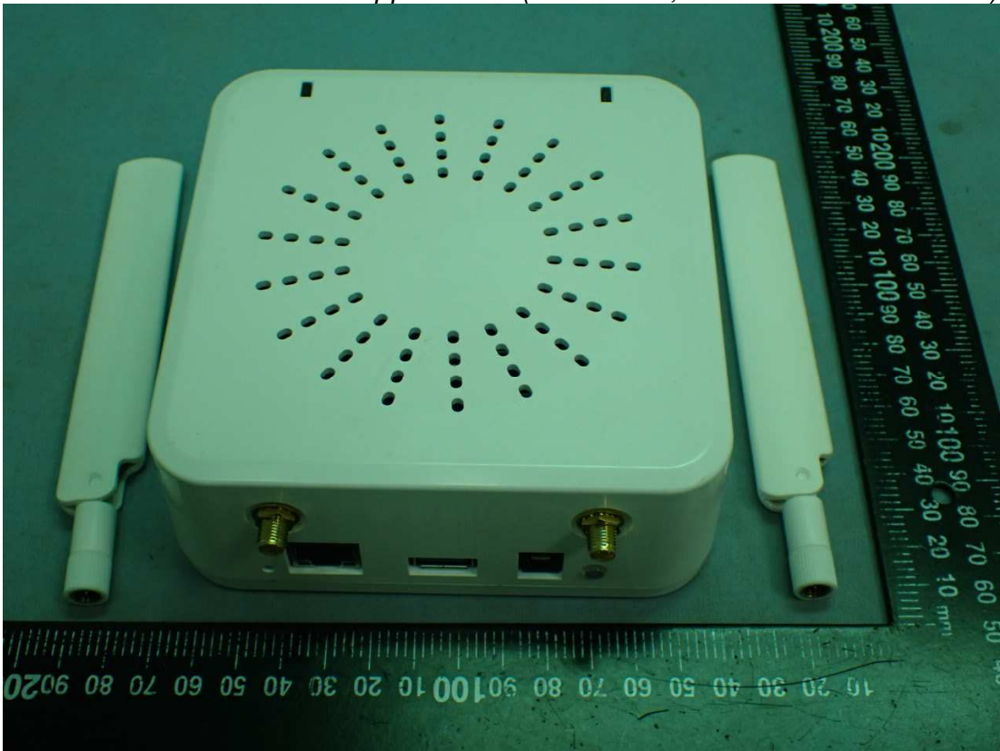
Figure 3 General Appearance (Front View, Removed LTE Antenna)
