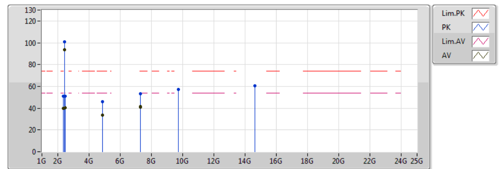
RE above 1GHz;Band:2.4G;HT20;BWch:20MHz;Nss:1,(M0-7);Nant:1;Ch:2437MHz;TX
