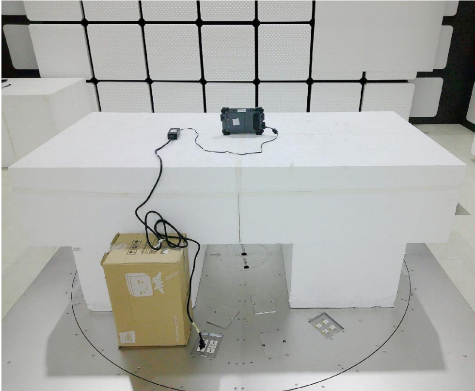
Description: Radiated Emission Test Setup for above 1GHz
