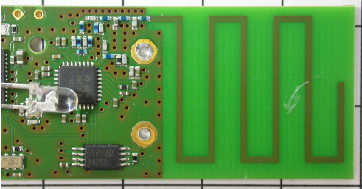
PCB top view (detailed RF part)
