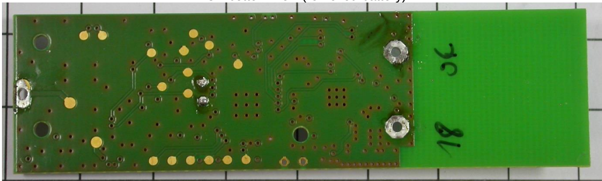
PCB bottom view (removed battery)
