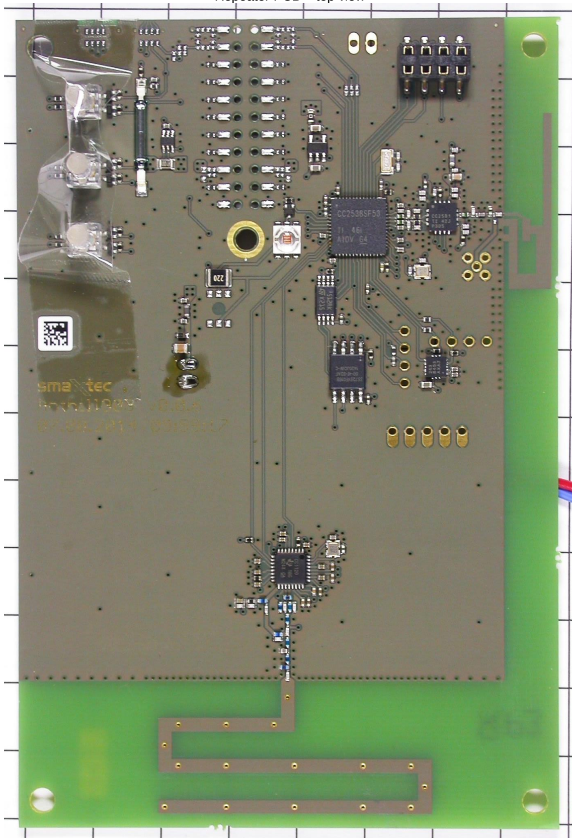
Repeater PCB – top view
