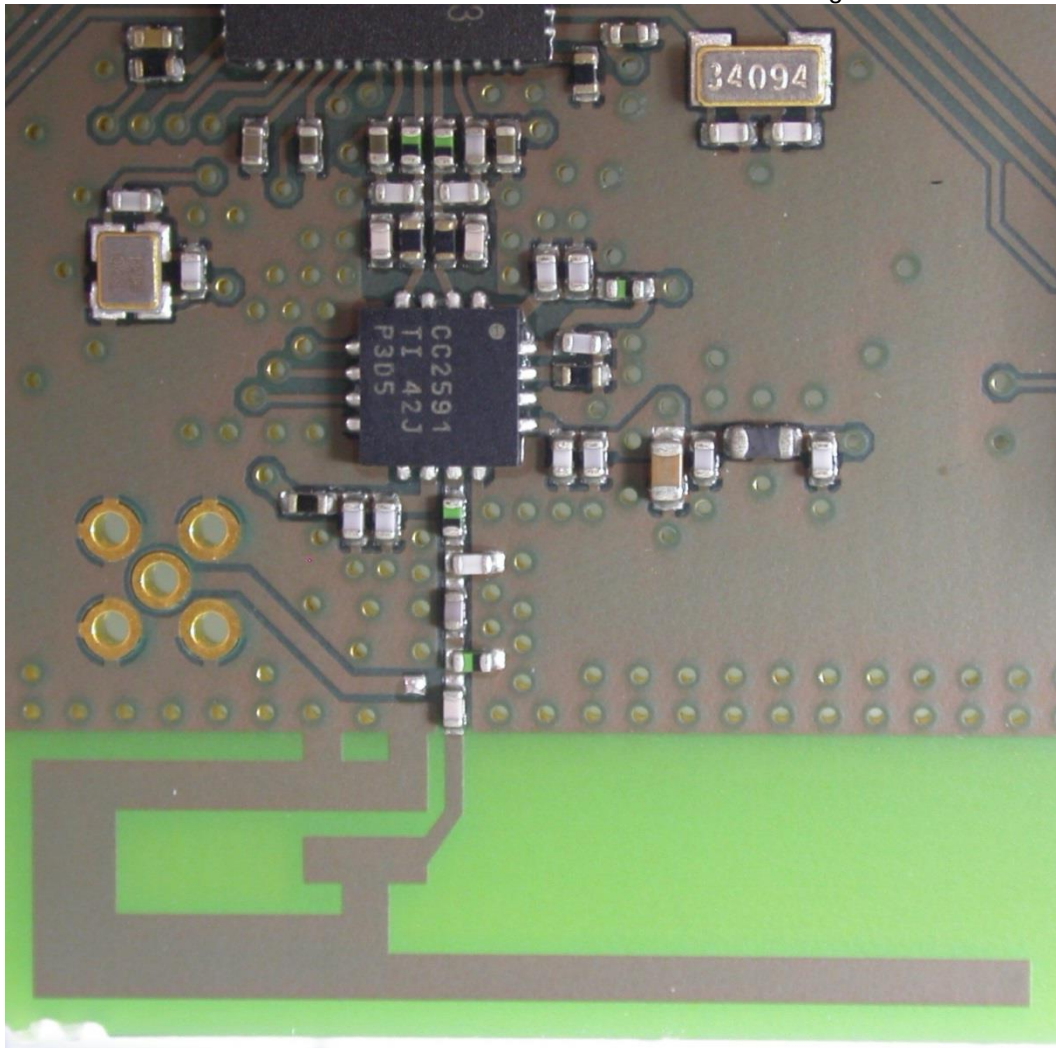
Printed antenna for 2400 MHz to 2483.5 MHz band – enlarged view
