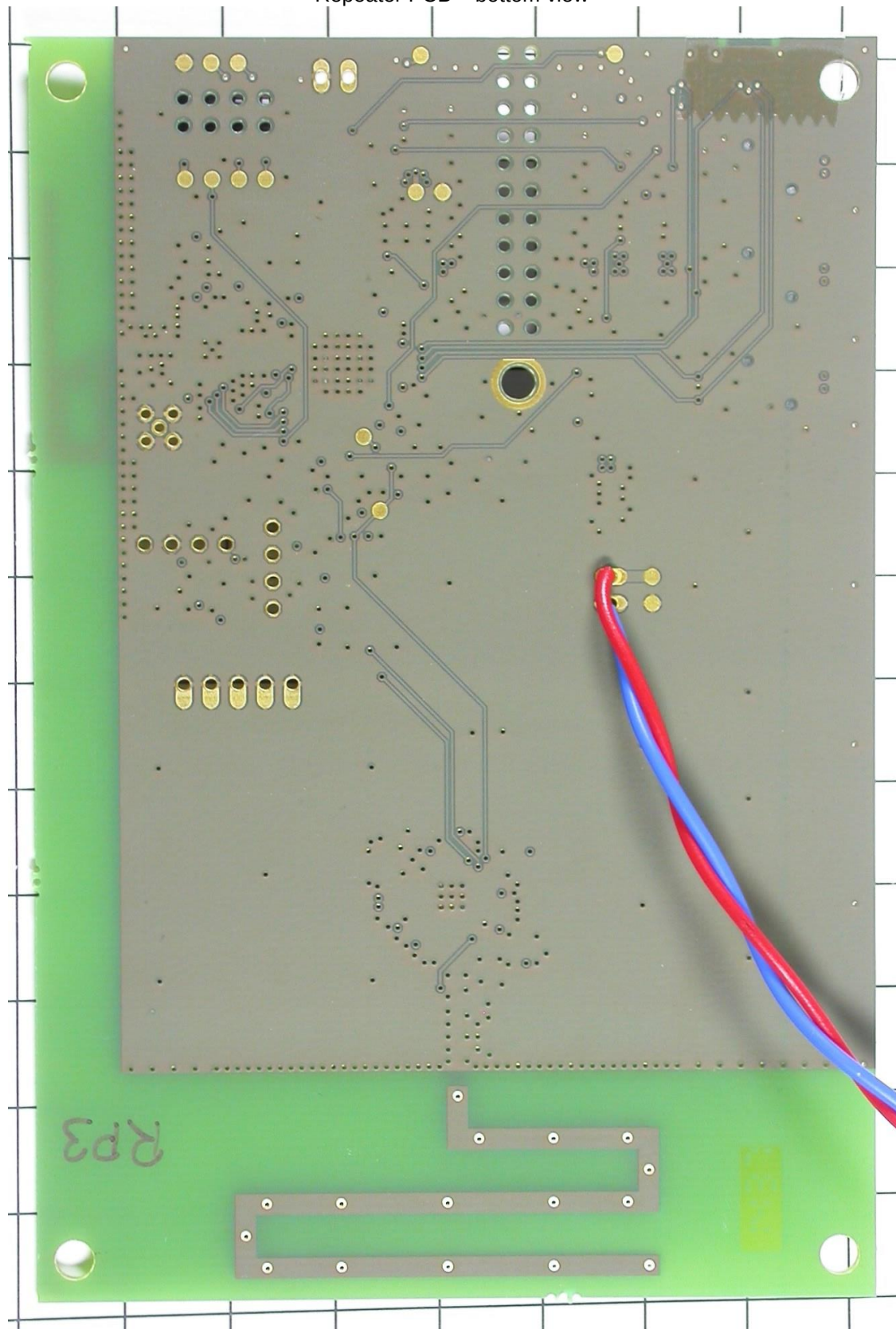
Repeater PCB – bottom view
