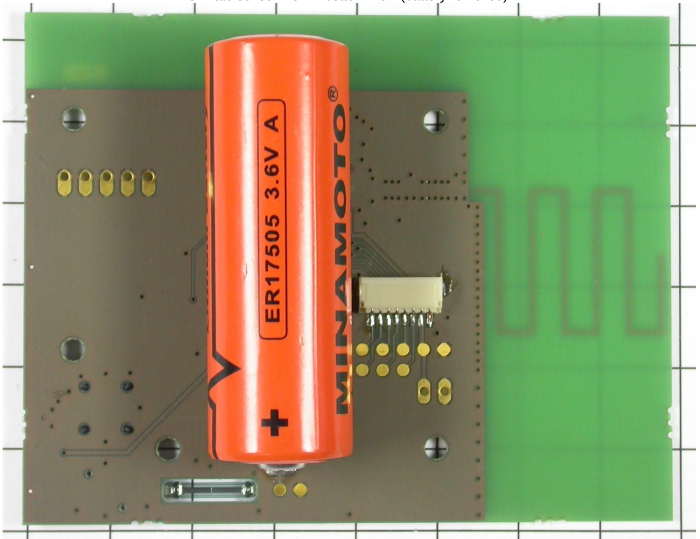
Climate sensor PCB – bottom view (battery removed)
