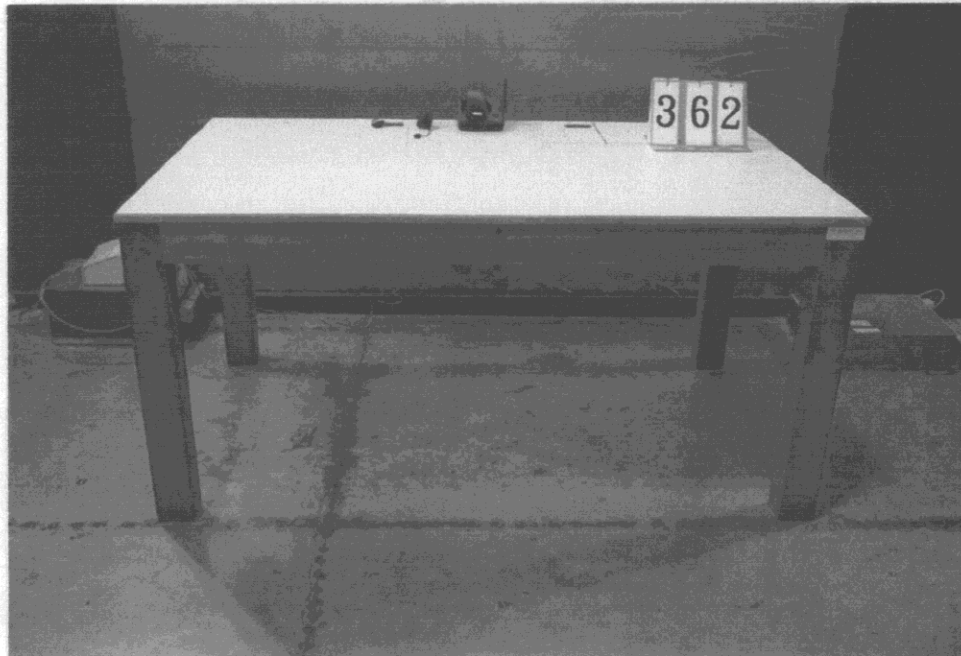
Fig. 1 Conducted emissions test placement (idle only)
