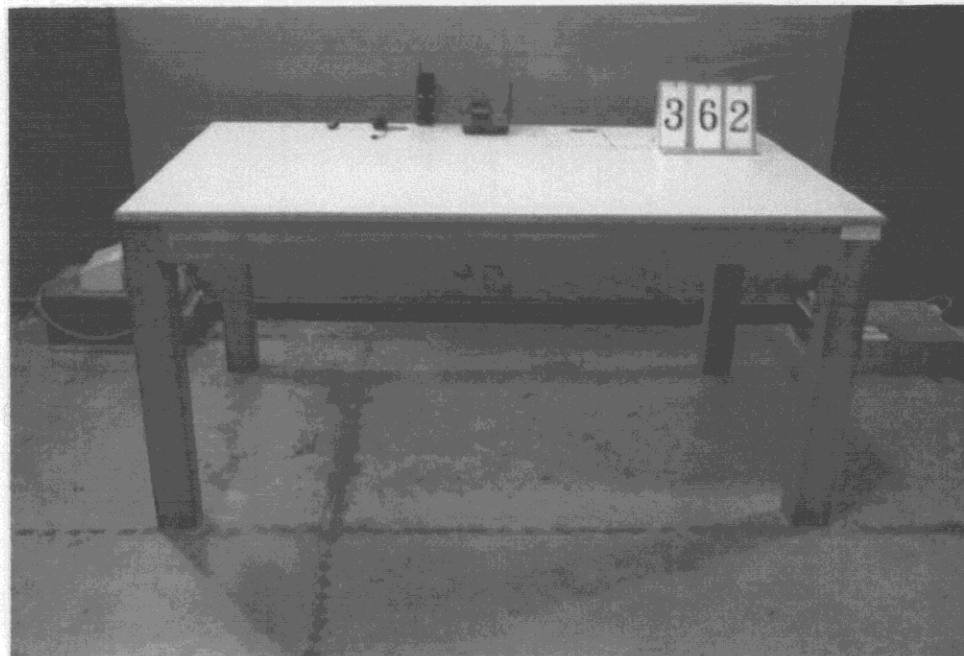
Fig. 2 Conducted emissions test placement (operating only)
