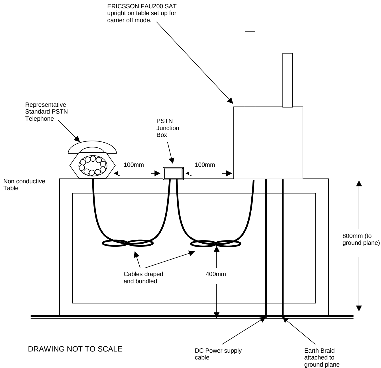
Figure 1: Ericsson FAU200 SAT CFR 47 Part 15.109 Radiated Emission Set up (Rear view)
