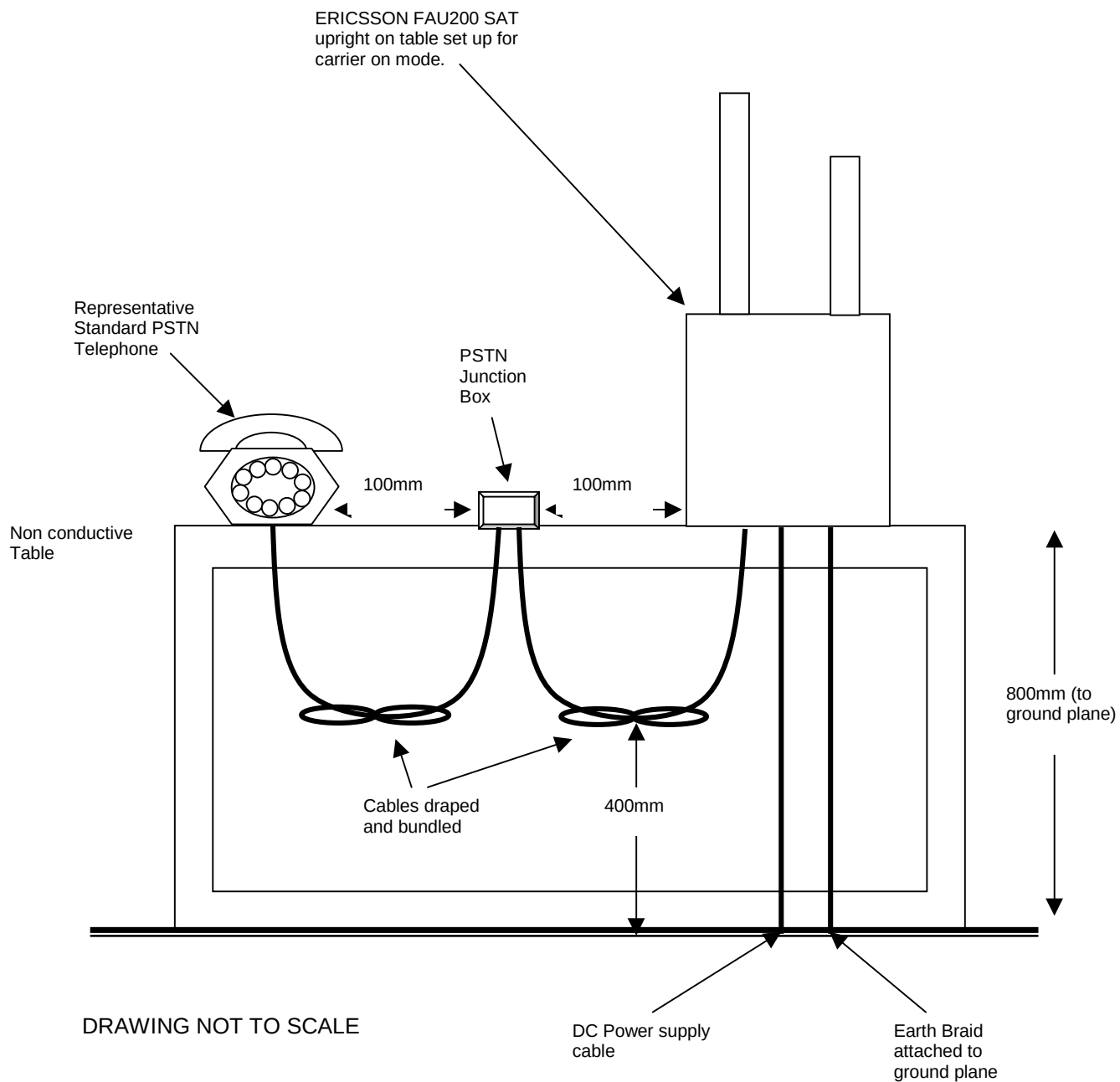
Figure 2: Ericsson FAU200 SAT CFR47 Part 25.202(f) Radiated Emission Set up (Rear view)
