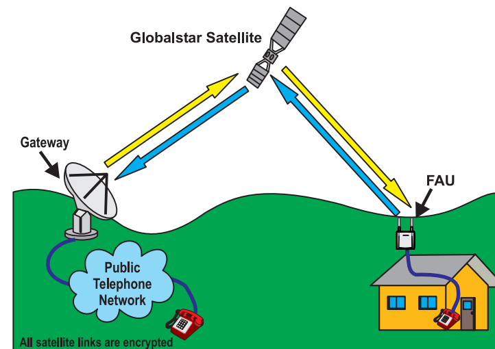
Typical Network
