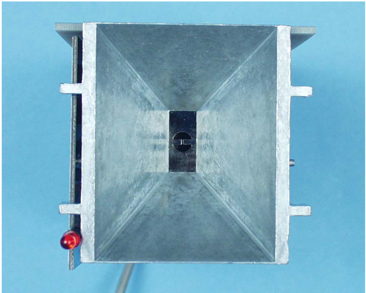
Internal Horn
