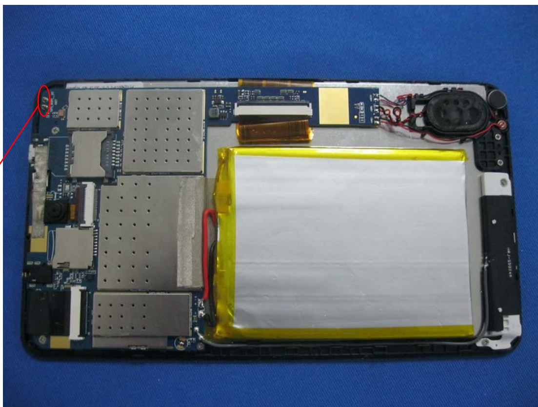
WIFI/BT ANTENNA
