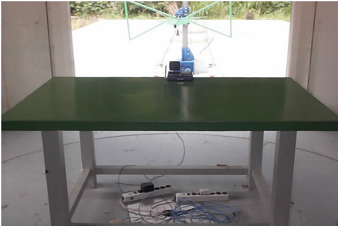
Back View of Radiated Emission Test (Mode 1)
