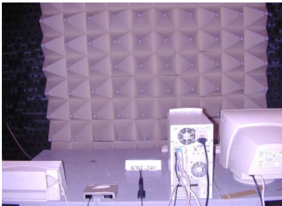
Photo 2: Spurious Set-up (rear)
