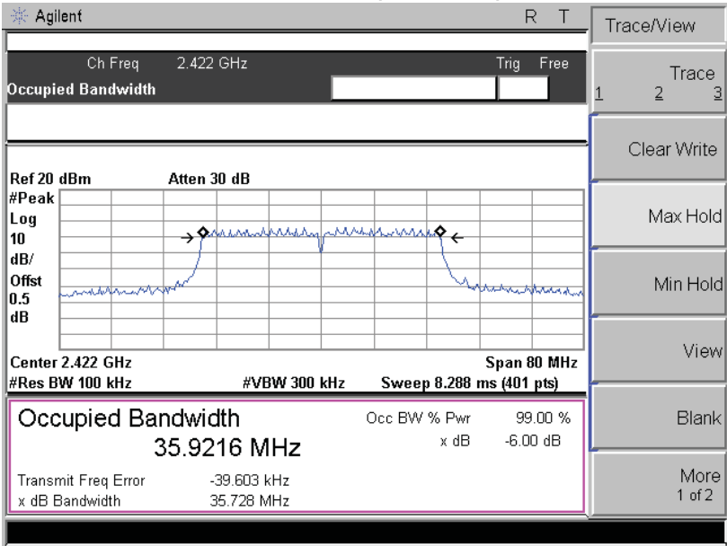
Channel 03 (2422MHz)
