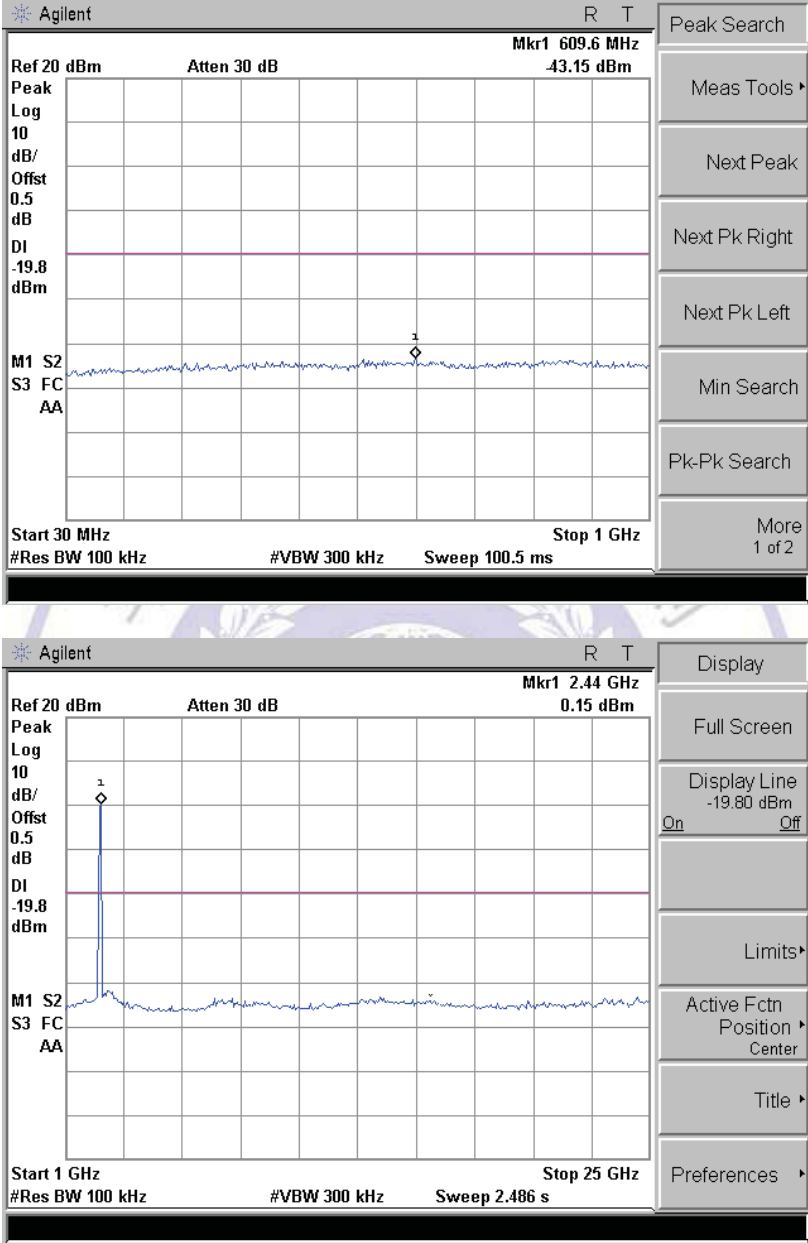
Channel 01 (2412MHz)
