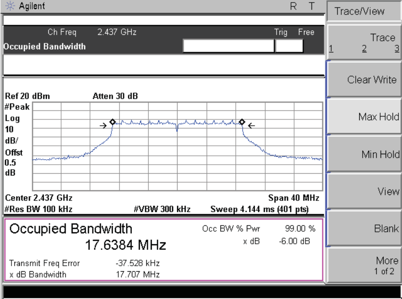
Channel 06 (2437MHz)
