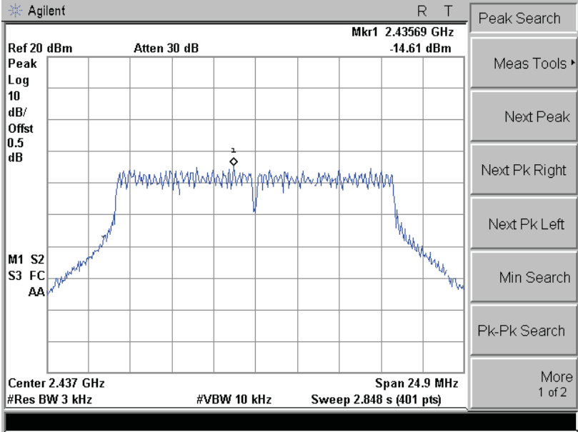
Channel 06 (2437MHz)
