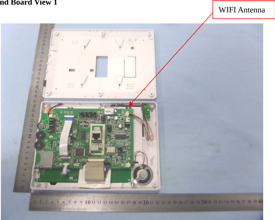
EUT Housing and Board View 1
