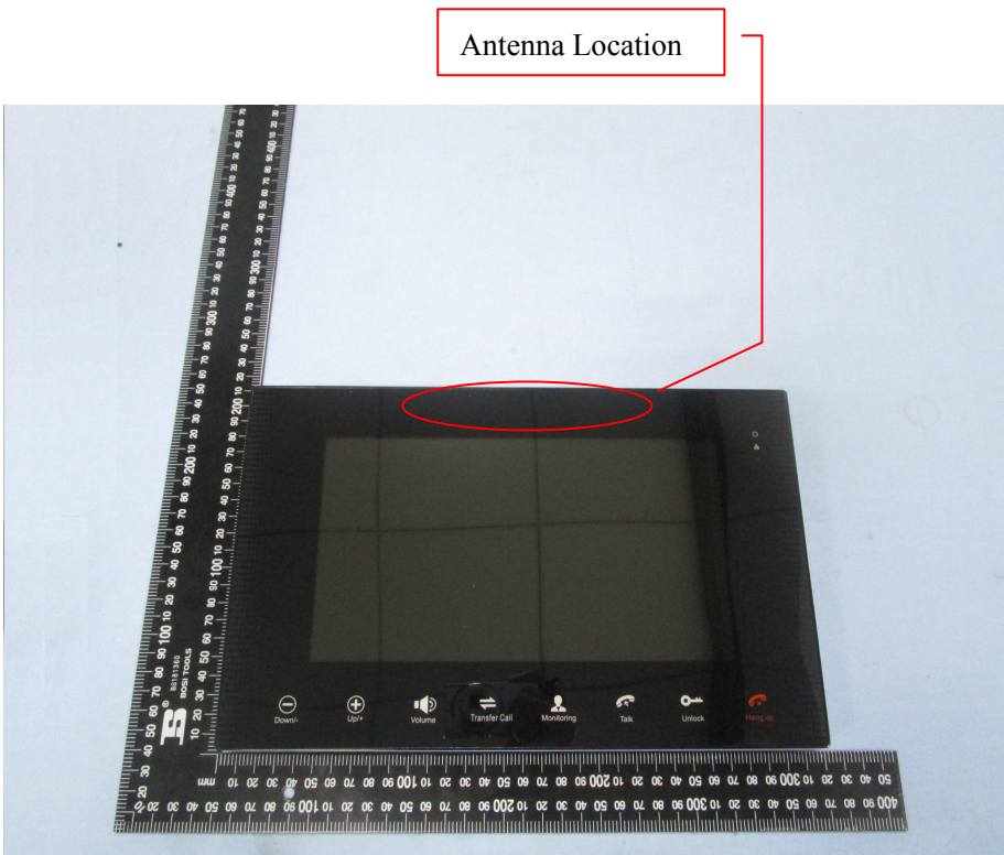
EUT View 2
