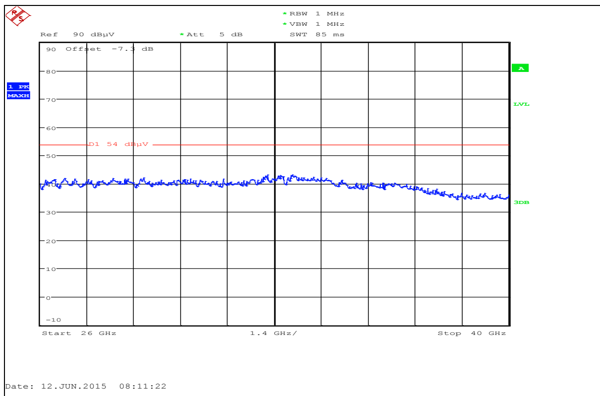
Plot 16: 26 GHz to 40 GHz, horizontal / vertical polarization, RX-mode
