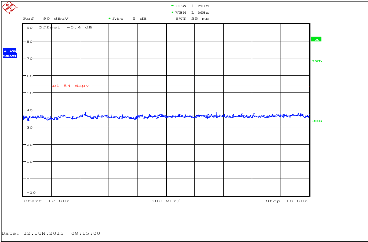
Plot 14: 12 GHz to 18 GHz, horizontal / vertical polarization, RX-mode
