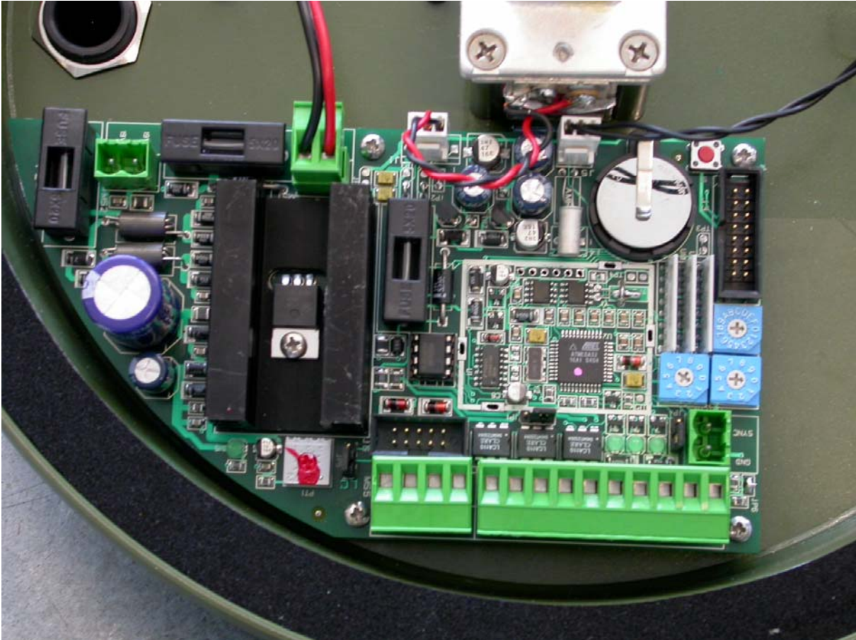
Transmitter
