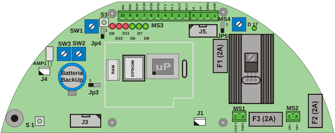
Figure 9 Layout of connectors, jumpers, LED and presetting in receiver board
