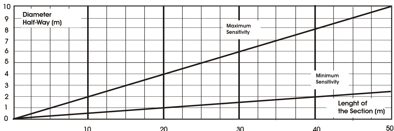
Figure 3 Diameter of sensitive beam at the half-section length (ERMO 482x PRO/ 50)
