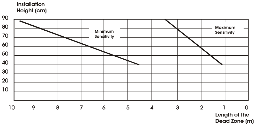
Figure 6 ERMOx 482. 80-120-200: Dead zone length near the equipment versus installation height.
