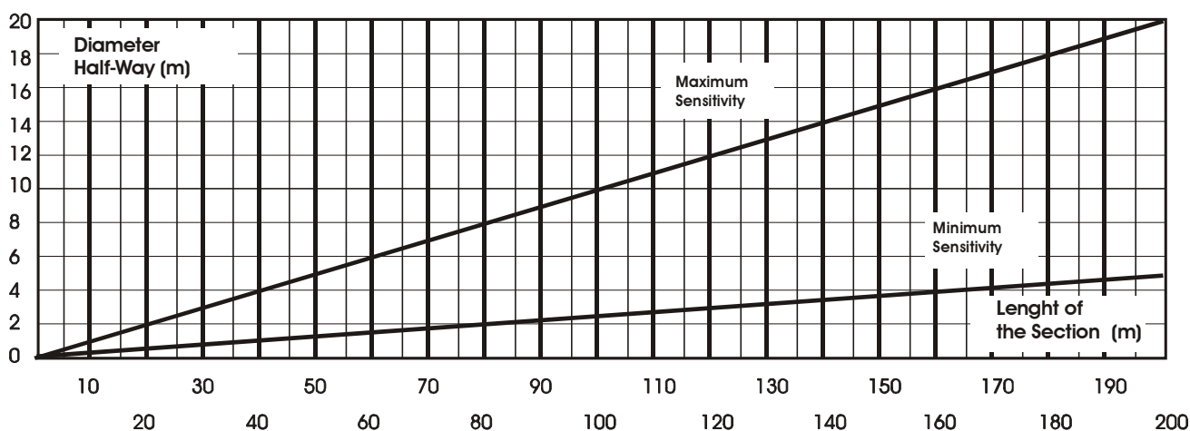
Figure 4 Diameter of sensitive beam at the half-section length (ERMO 482x PRO/ 80-120-200)
