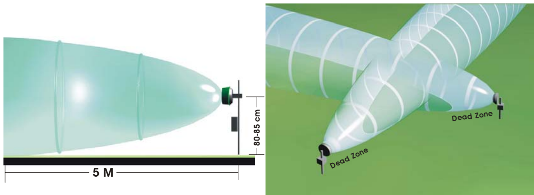
Figure 6 ERMOx 482. 80-120-200: Dead zone length near the equipment versus installation height.
