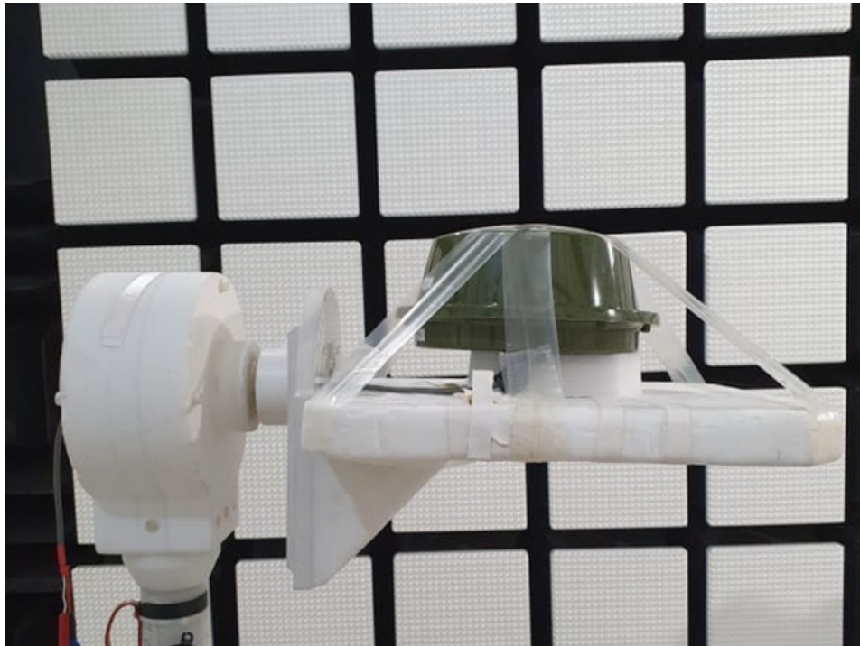
Photo 3: Setup Shielded fully anechoic chamber
