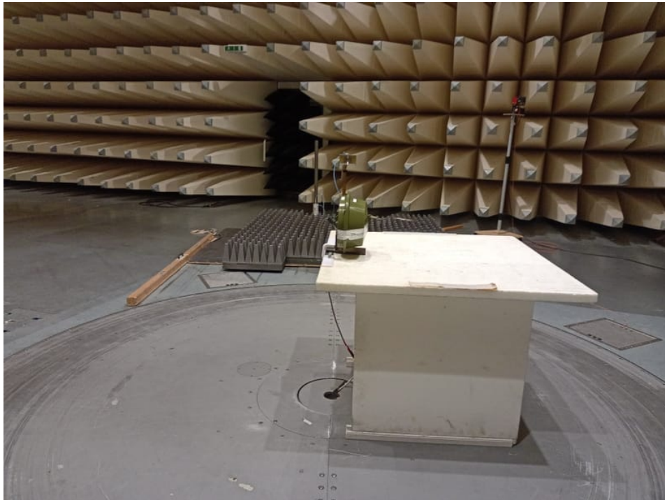
Photo 7: Setup Shielded semi anechoic chamber
