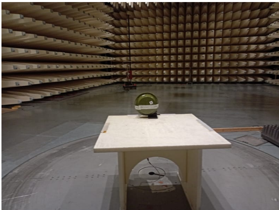
Photo 8: Setup Shielded semi anechoic
