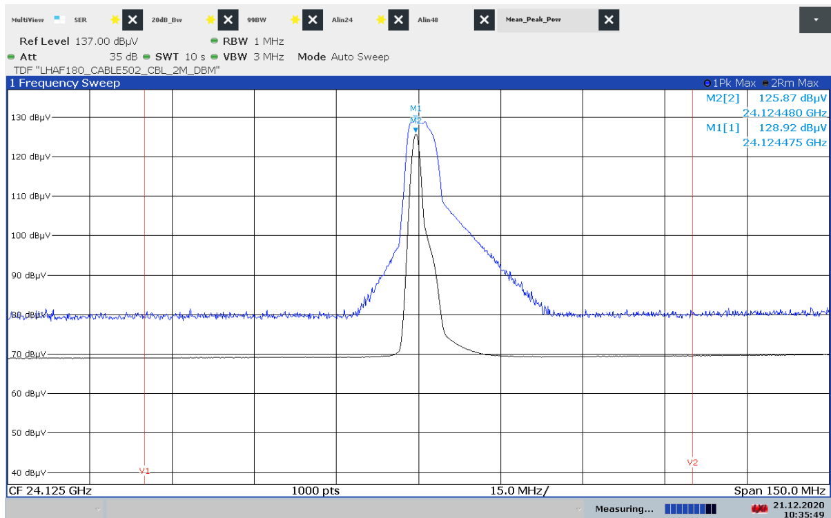
Plot 23: +20 °C, V_{\text{nom}}
