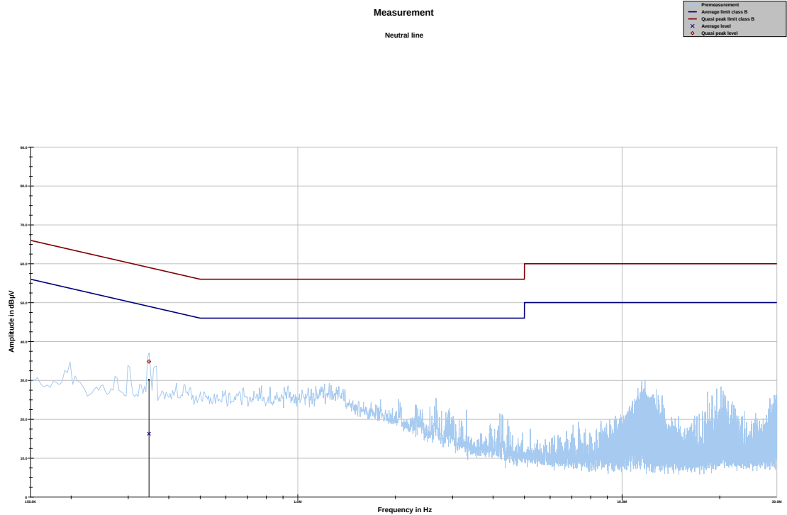
Plot 15: Neutral line, Transmitter
