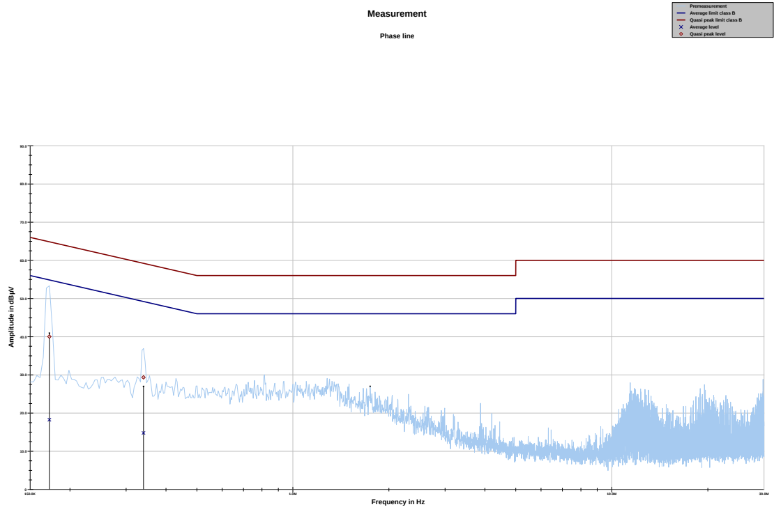
Plot 14: Phase line, Transmitter
