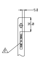
VIEW C
