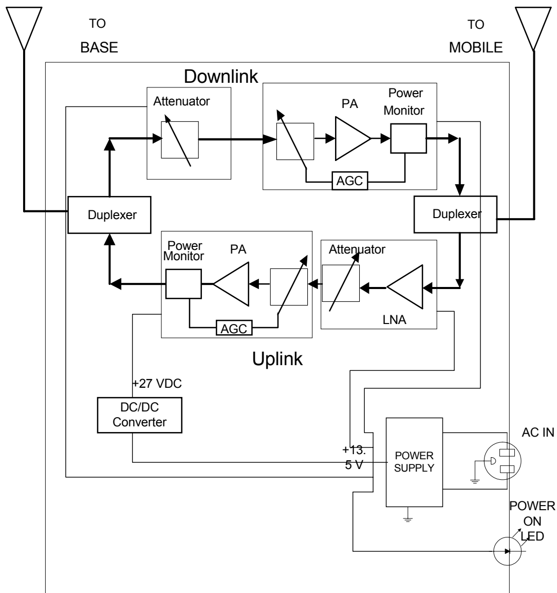
IBDB-10W40 ELECTRICAL SCHEMATICS
