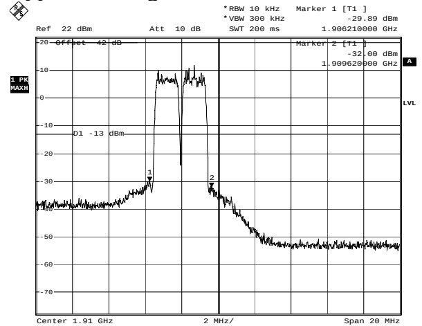
CDMA Upper Bandedge - Uplink
