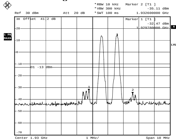
GSM Lower Bandedge - Downlink
