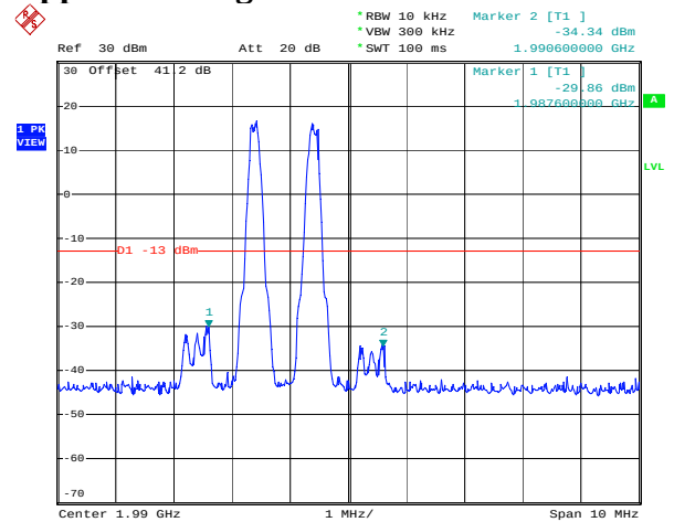
GSM Upper Bandedge - Downlink
