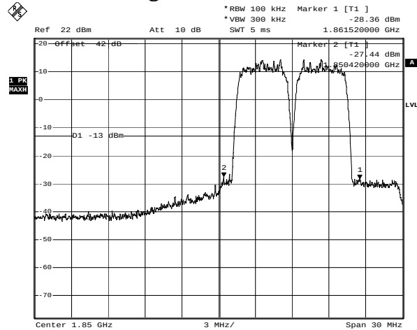
WCDMA Lower Bandedge - Uplink
