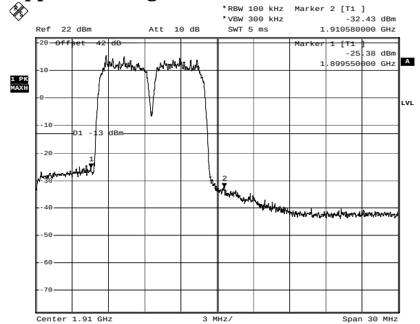
WCDMA Upper Bandedge - Uplink
