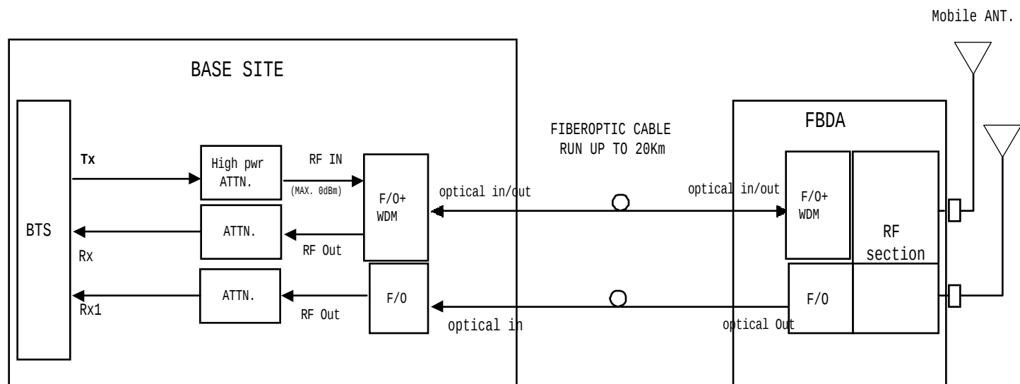
Fig.2 : FBDA SYSTEM BLOCK DIAGRAM
