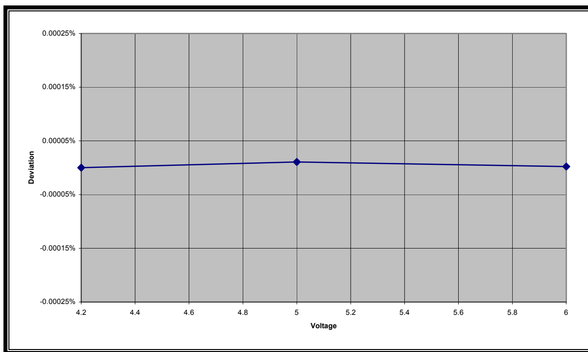
PLOT 4-2: FREQUENCY STABILITY VS VOLTAGE
