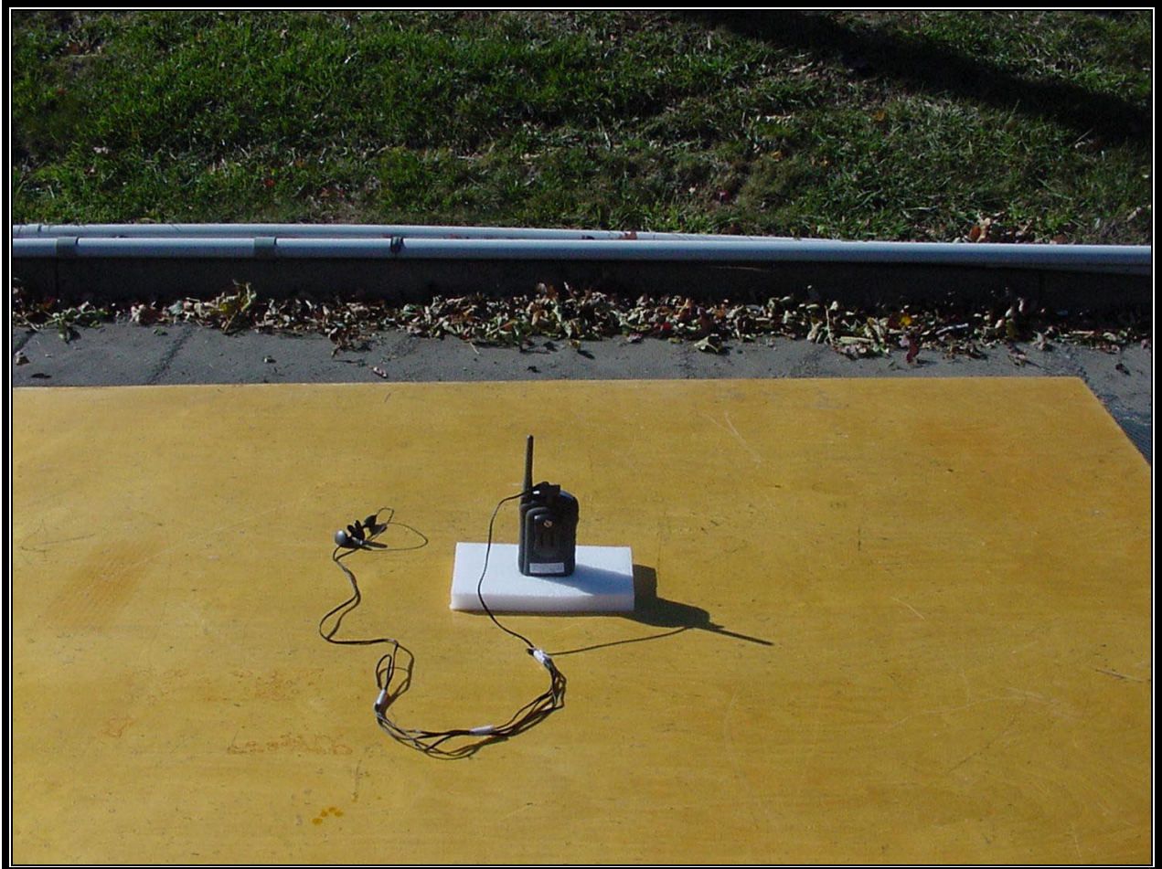
PHOTOGRAPH 2: REAR VIEW – RADIATED TESTING
