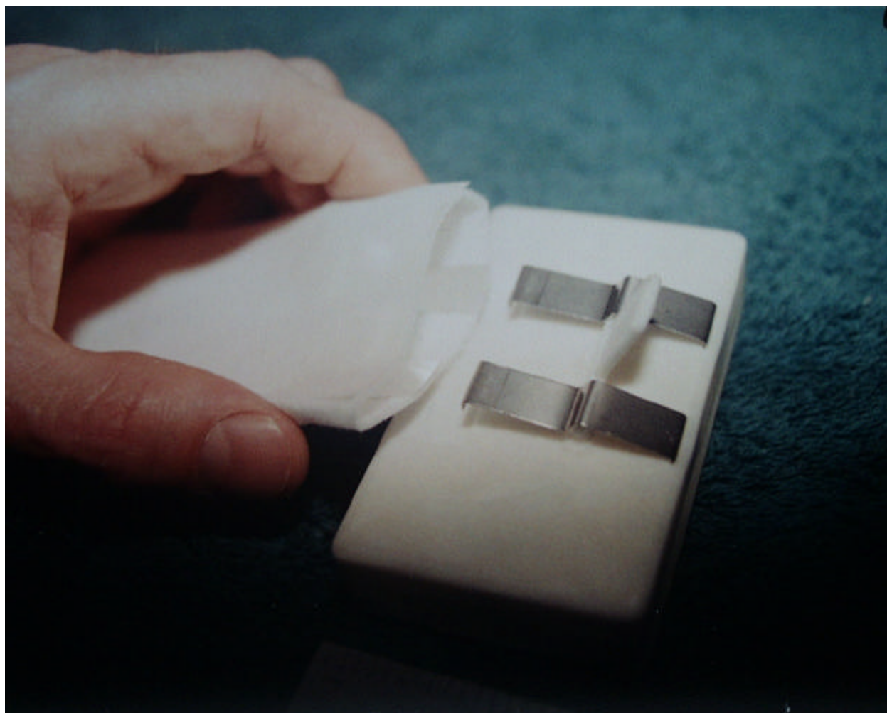
Back View of the 6000-4 showing Sensor'R Strip being installed
