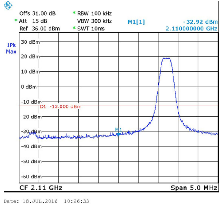
Figure 52. — GSM 2111.2 MHz
