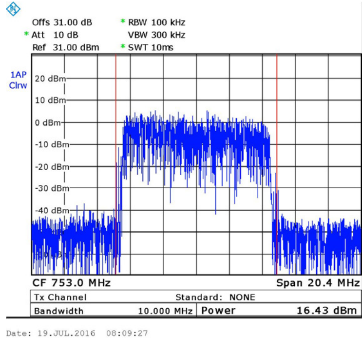
Figure 13. — 64QAM 753 MHz
