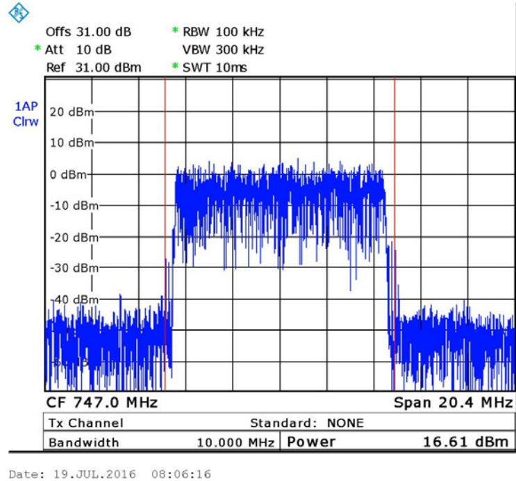
Figure 15. — 16QAM 747 MHz
