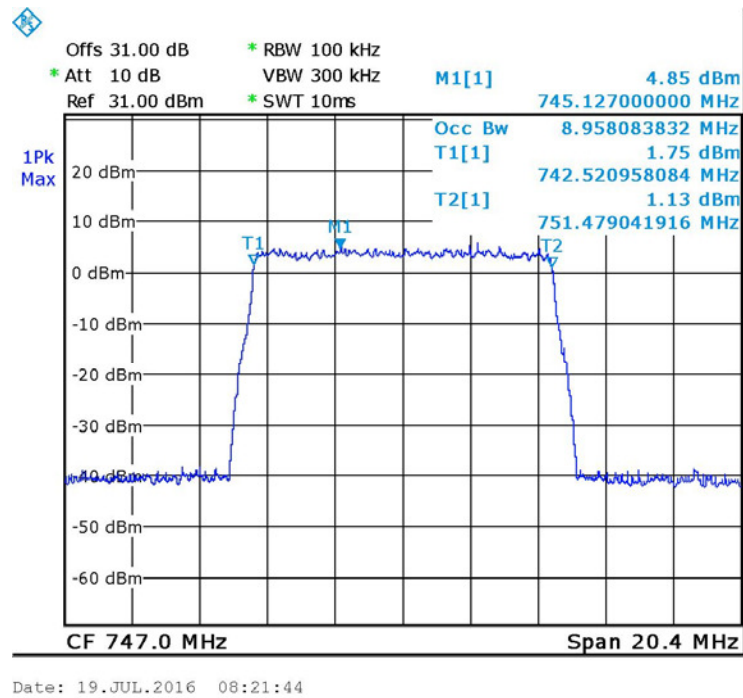
Figure 37. — QPSK 747 MHz OUT
