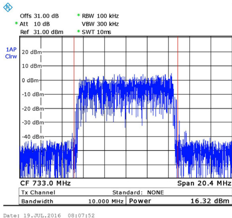
Figure 11. — 64QAM, 733 MHz
