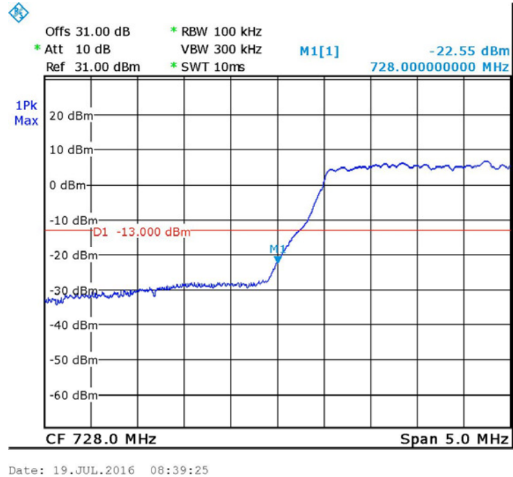
Figure 54.—16QAM 728.0 MHz
