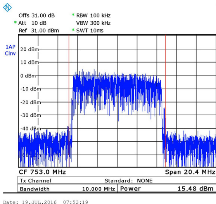
Figure 19. — QPSK 753 MHz
