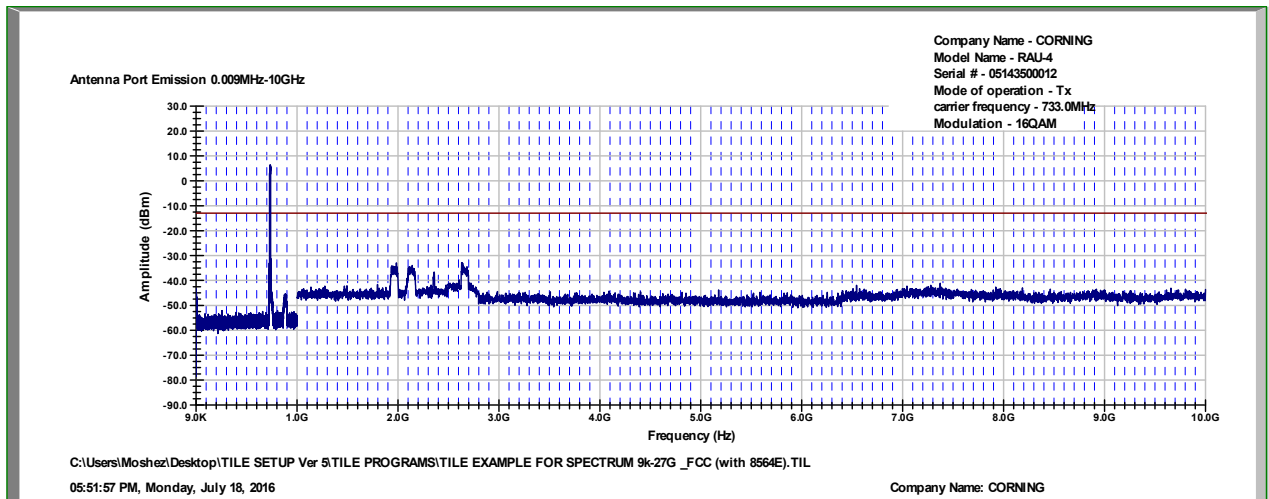
Figure 44 Spurious Emissions at Antenna Terminals 16QAM, 733MHz
