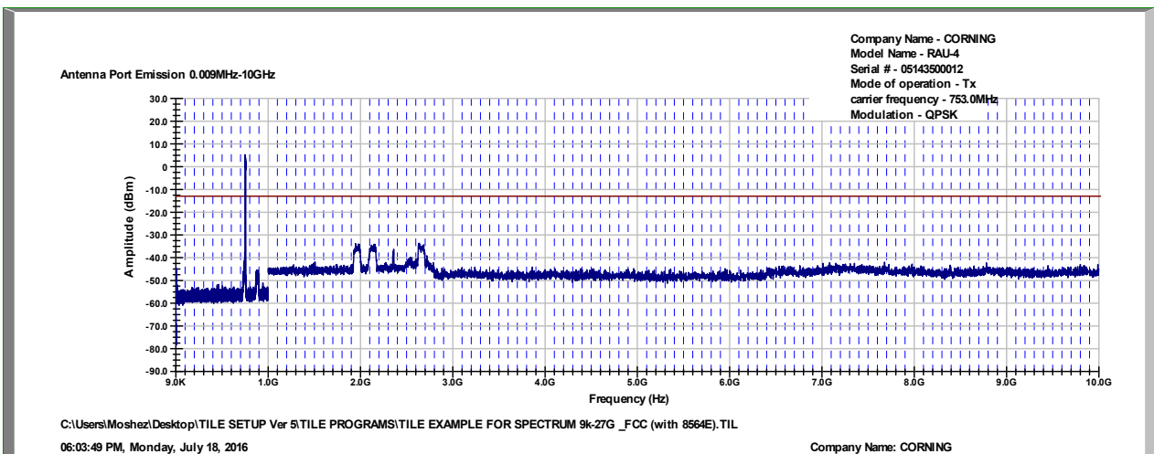
Figure 49 Spurious Emissions at Antenna Terminals QPSK, 753MHz
