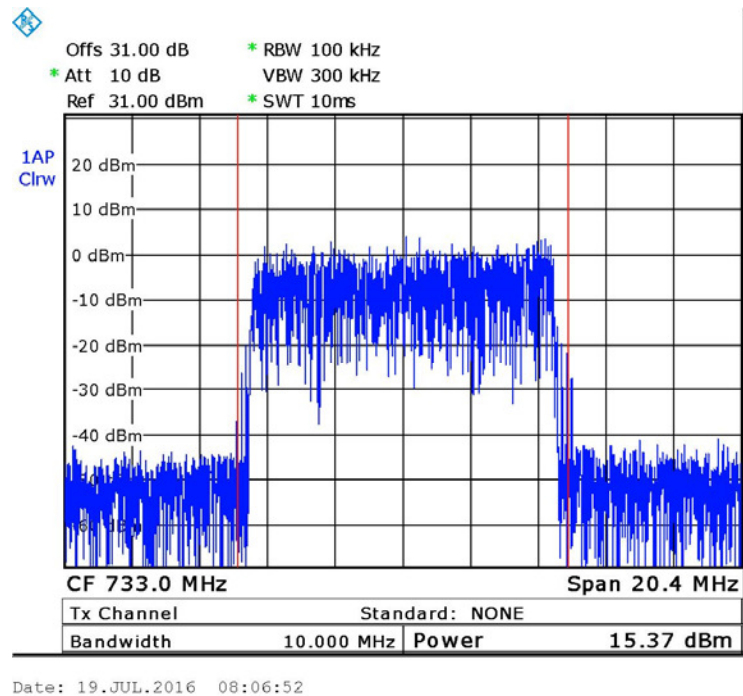
Figure 14. — 16QAM 733 MHz
