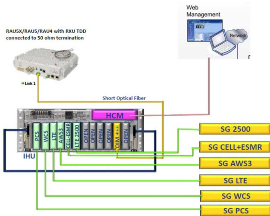
Figure 2. Test Set-Up – Radiated
