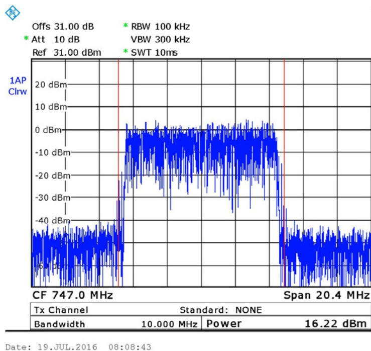
Figure 12. — 64QAM 747 MHz
