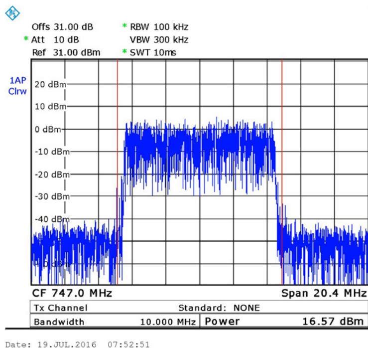
Figure 18. — QPSK 747 MHz
