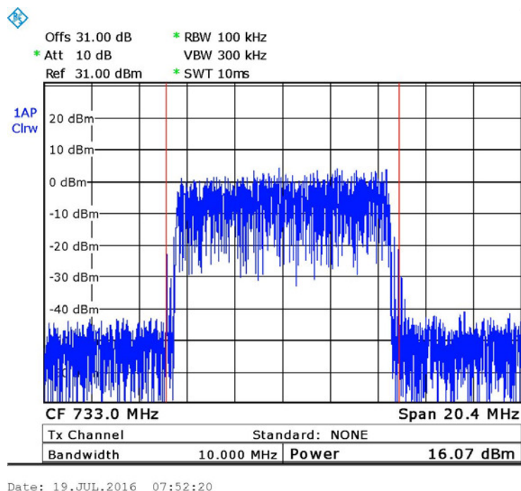
Figure 17. — QPSK 733 MHz
