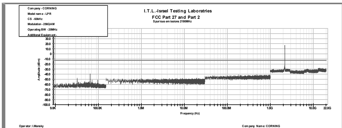
Figure 401: Spurious Emissions at Antenna Terminal 256QAM, 2190.0MHz, B.W. 20MHz, Sub Carrier 60 kHz
