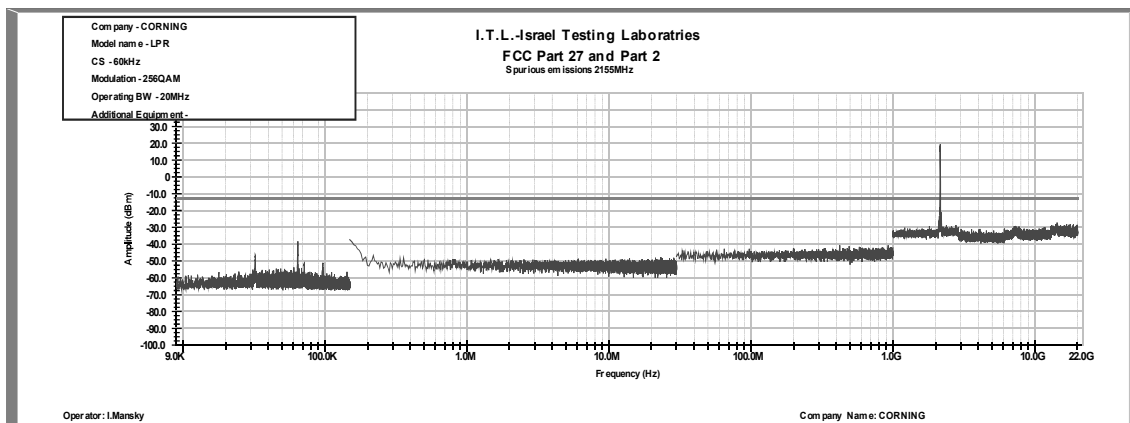
Figure 400: Spurious Emissions at Antenna Terminal 256QAM, 2155.0MHz, B.W. 20MHz, Sub Carrier 60 kHz
