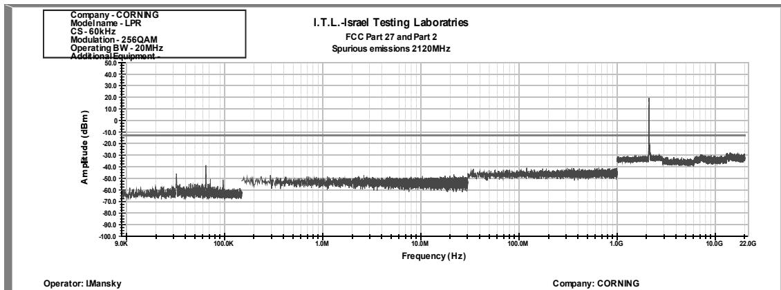
Figure 399: Spurious Emissions at Antenna Terminal 256QAM, 2120.0MHz, B.W. 20MHz, Sub Carrier 60 kHz
