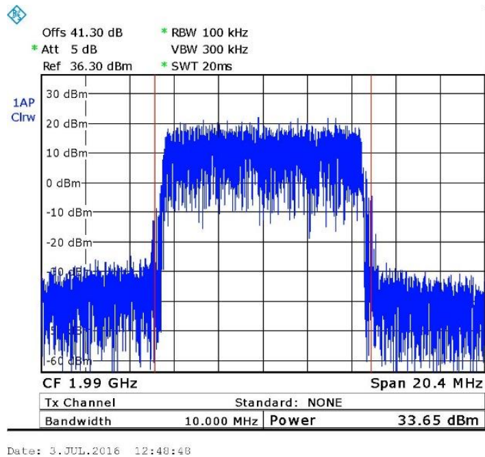
Figure 13. — LTE 64QAM 1990.00 MHz
