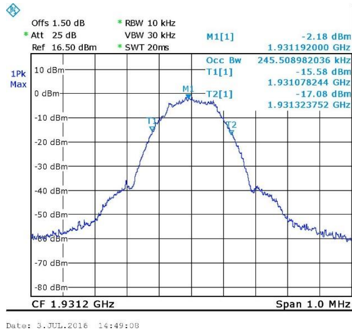
Figure 28. — GSM - Input 1931.2 MHz
