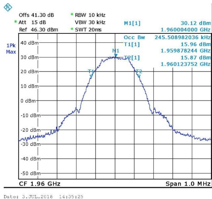
Figure 31. — GSM - Output 1960.0 MHz
