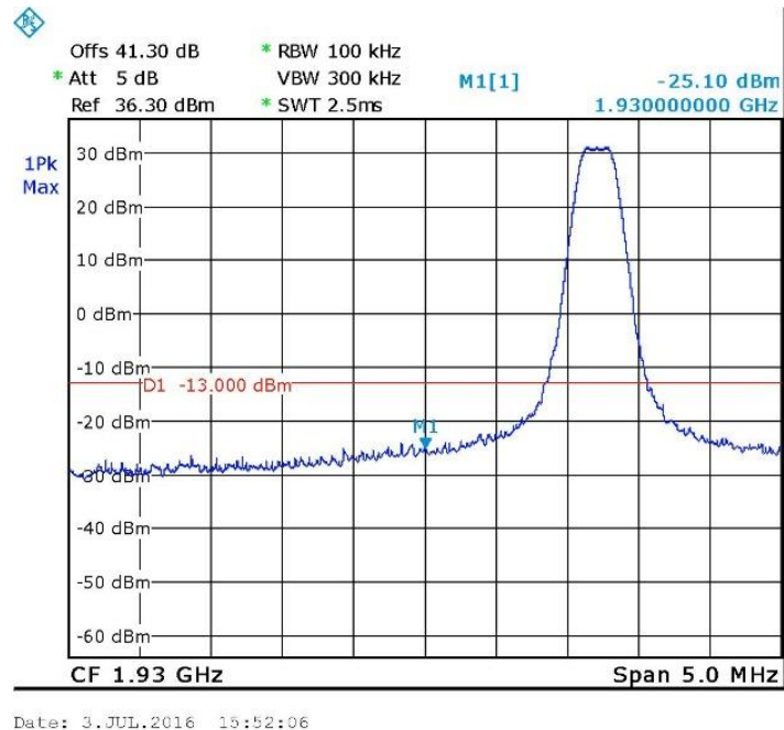
Figure 54. — GSM - 1931.2 MHz
