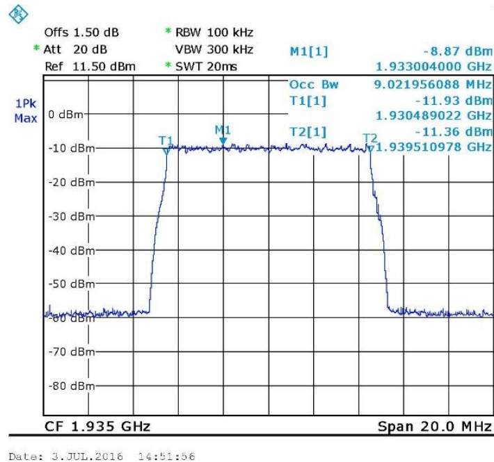
Figure 22. — LTE 64QAM Input 1935.0 MHz
