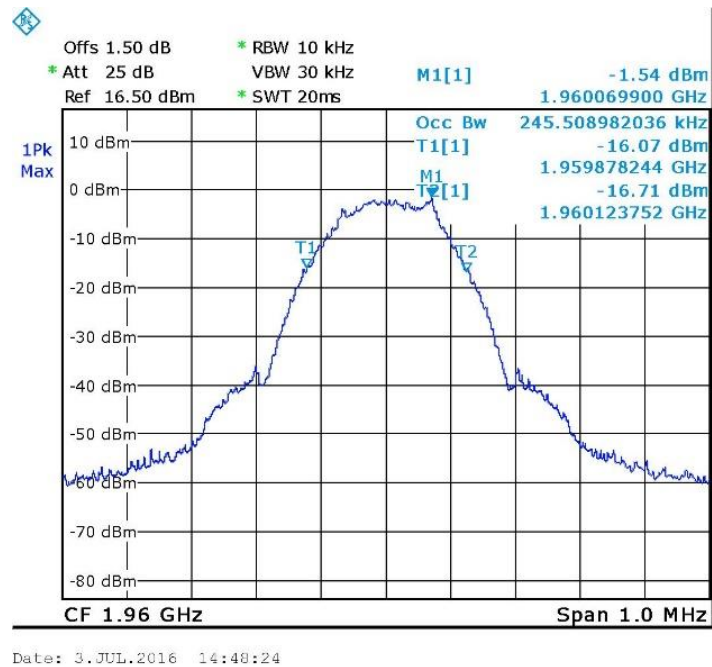
Figure 30. — GSM - Input 1960.0 MHz
