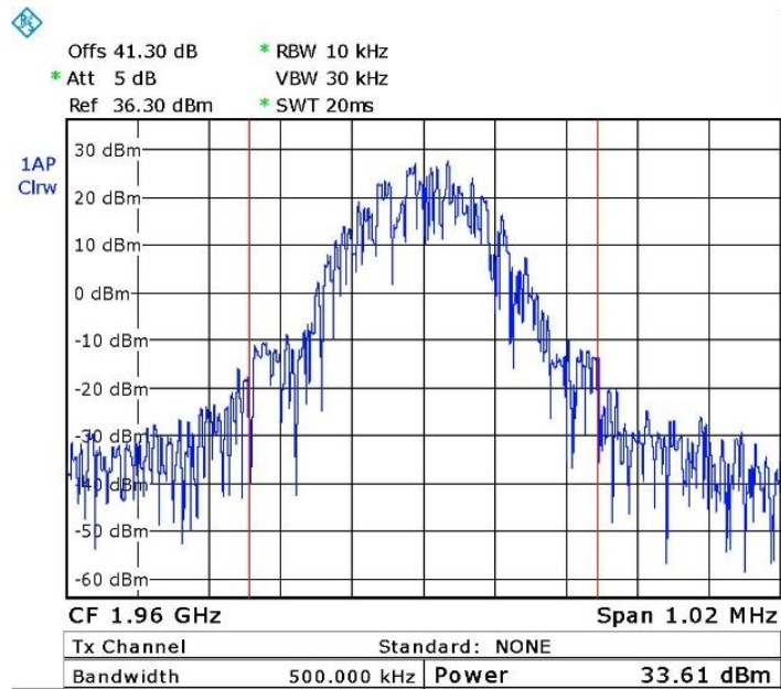
Figure 15. — GSM -1960.00 MHz
