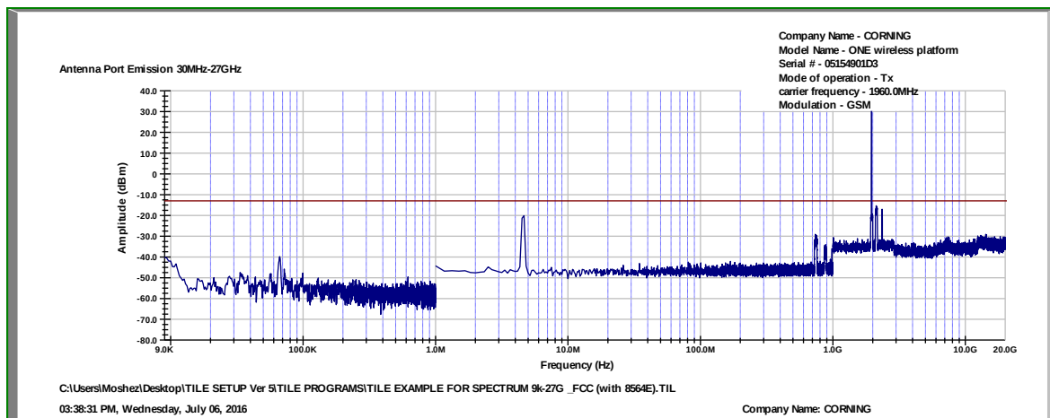
Figure 45. — GSM - 1960.0 MHz
