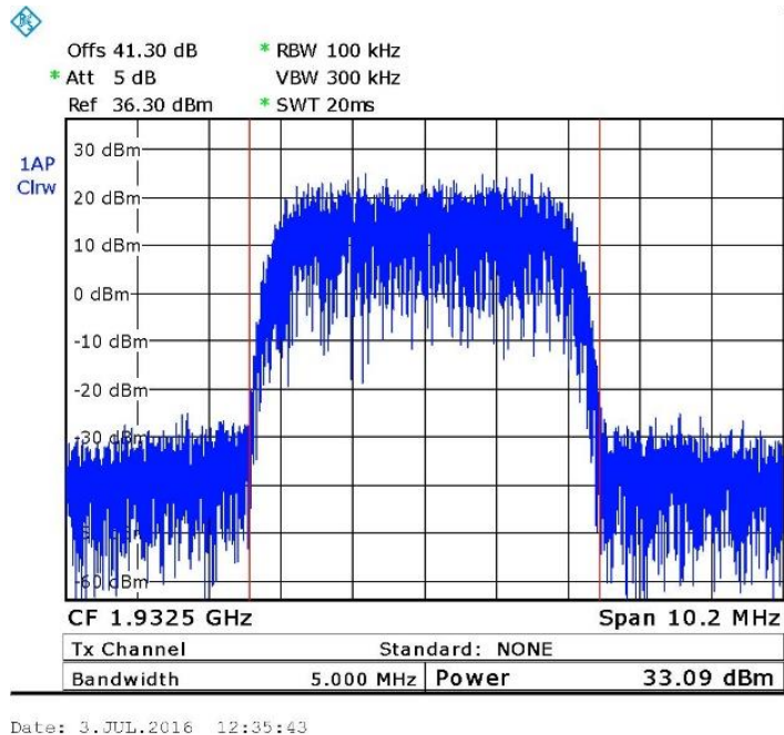
Figure 17. — W-CDMA - 1932.50 MHz
