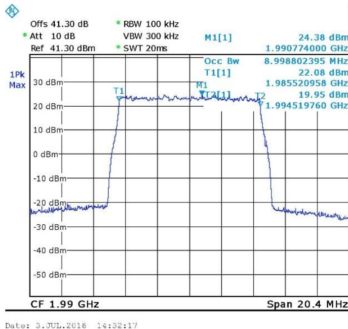
Figure 27. — LTE 64QAM Output 1990.0 MHz
