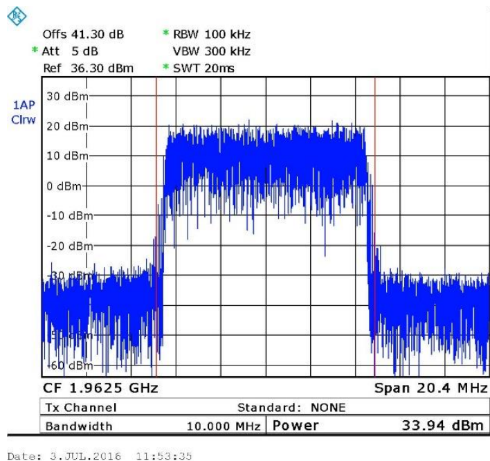
Figure 12. — LTE 64QAM 1962.50 MHz
