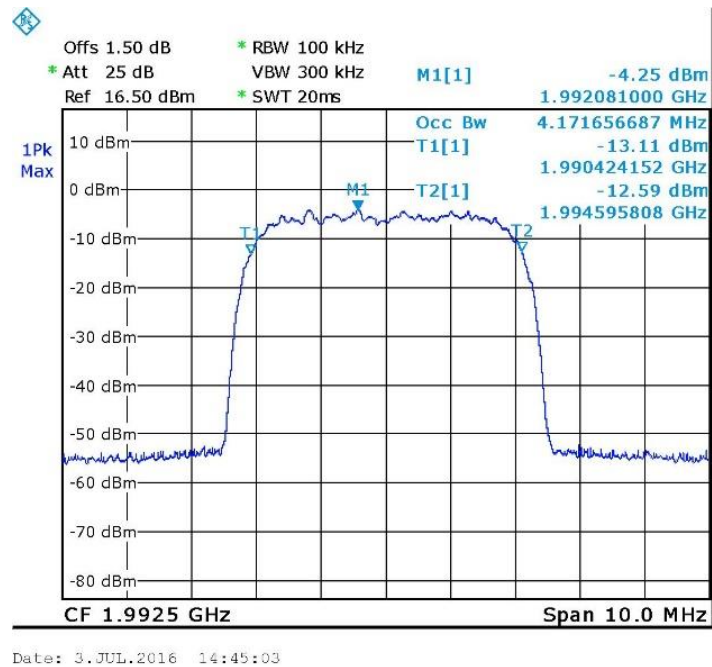
Figure 38. — W-CDMA - Input 1992.5 MHz
