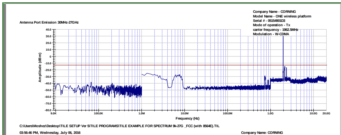
Figure 48. — W-CDMA - 1962.5 MHz
