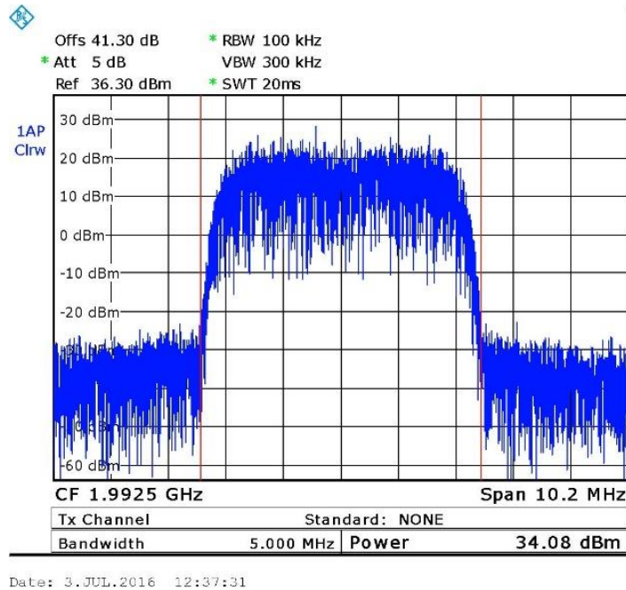
Figure 19. — W-CDMA - 1992.50 MHz
