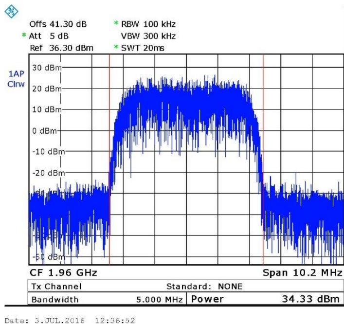
Figure 18. — W-CDMA - 1960.00 MHz
