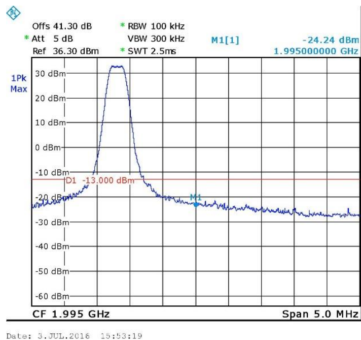
Figure 55. — GSM - 1993.8 MHz
