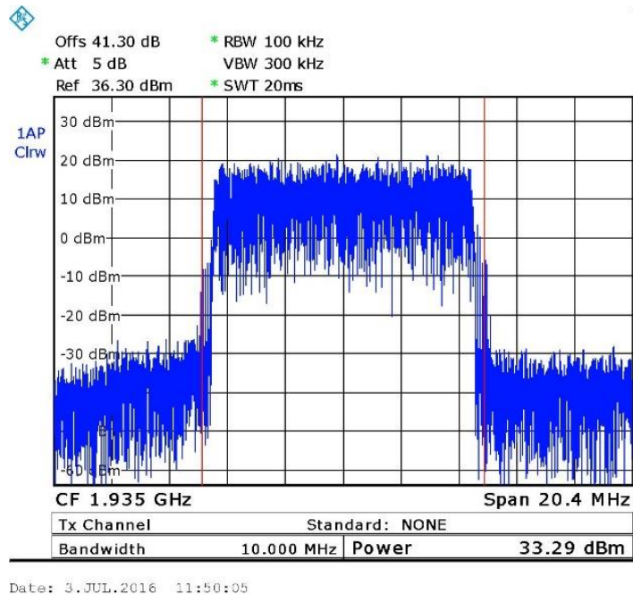
Figure 11. — LTE 64QAM 1935.00 MHz
