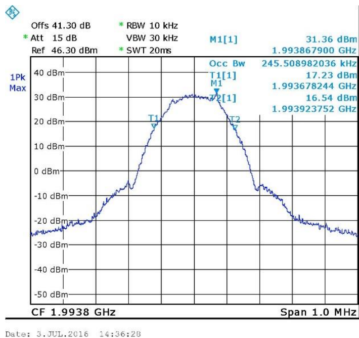
Figure 33. — GSM - Output 1993.8 MHz
