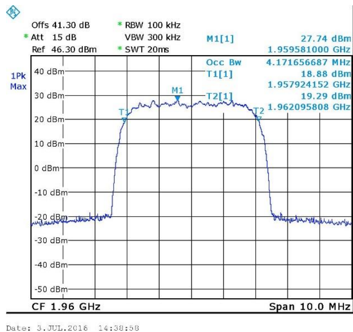
Figure 37. — W-CDMA - Output 1960.0 MHz
