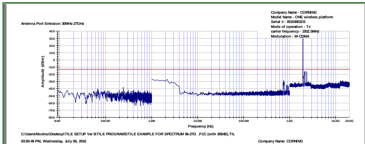
Figure 47. — W-CDMA - 1932.5 MHz
