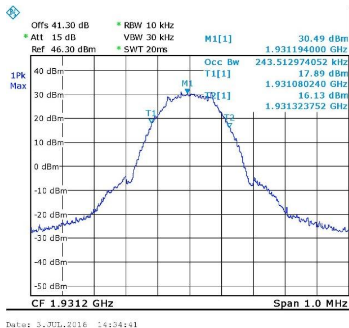
Figure 29. — GSM - Output 1931.2 MHz
