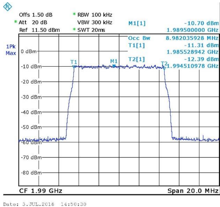
Figure 26. — LTE 64QAM Input 1990.0 MHz
