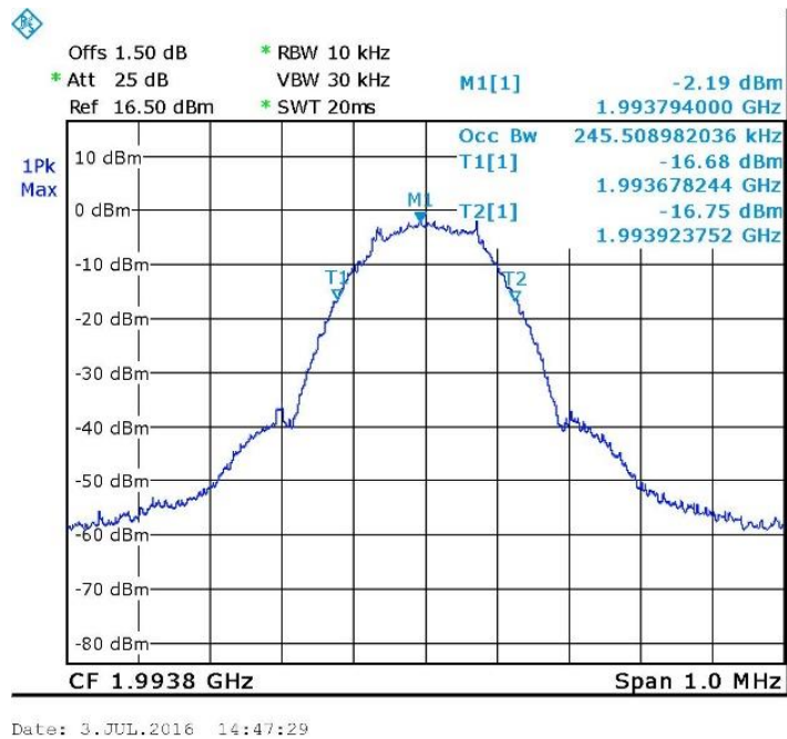
Figure 32. — GSM - Input 1993.8 MHz
