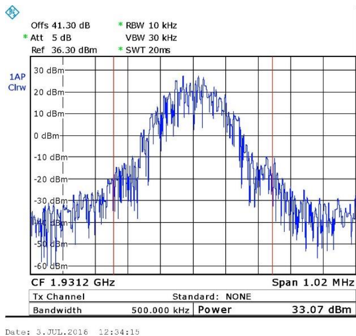
Figure 14. — GSM - 1931.20 MHz
