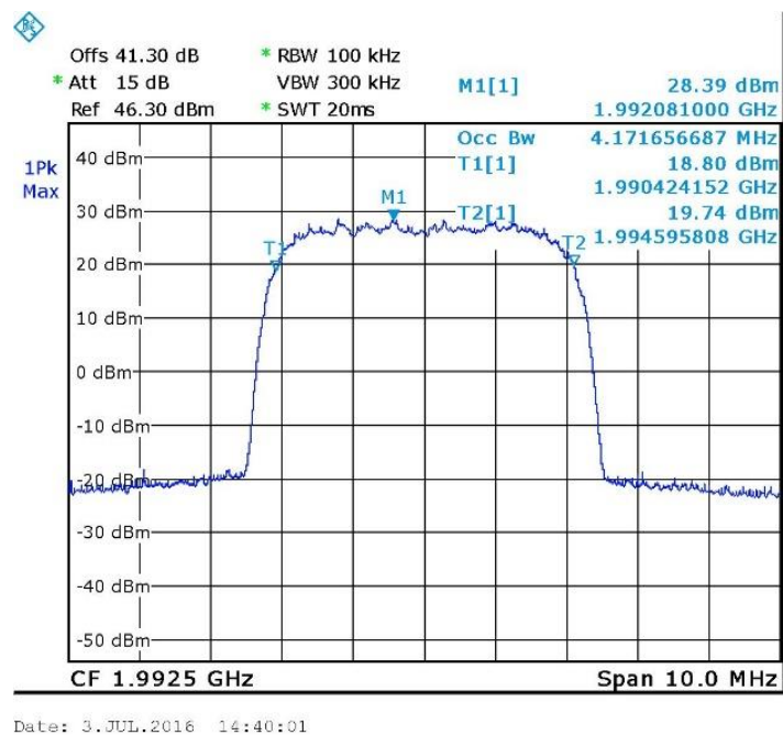
Figure 39. — W-CDMA - Output 1992.5 MHz
