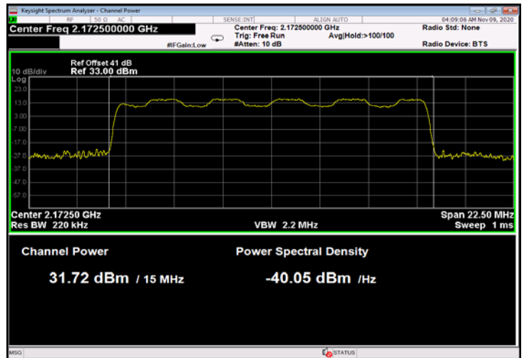
Figure 30: 16QAM 15MHz B.W.; 2172.5MHz, 15kHz
