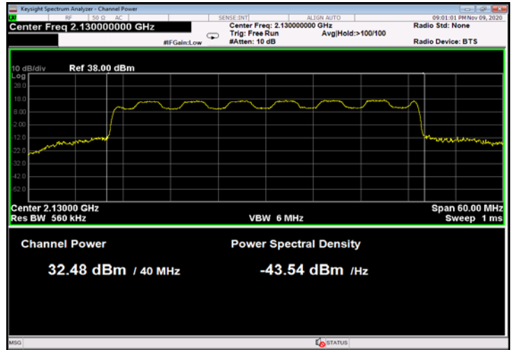
Figure 52: 16QAM 40MHz B.W.; 2130.0MHz, 30kHz
