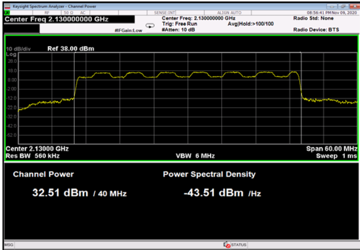
Figure 51: 16QAM 40MHz B.W.; 2130.0MHz, 15kHz
