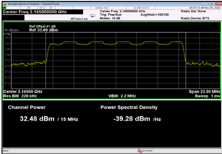
Figure 27: 16QAM 15MHz B.W.; 2145.0MHz, 15kHz
