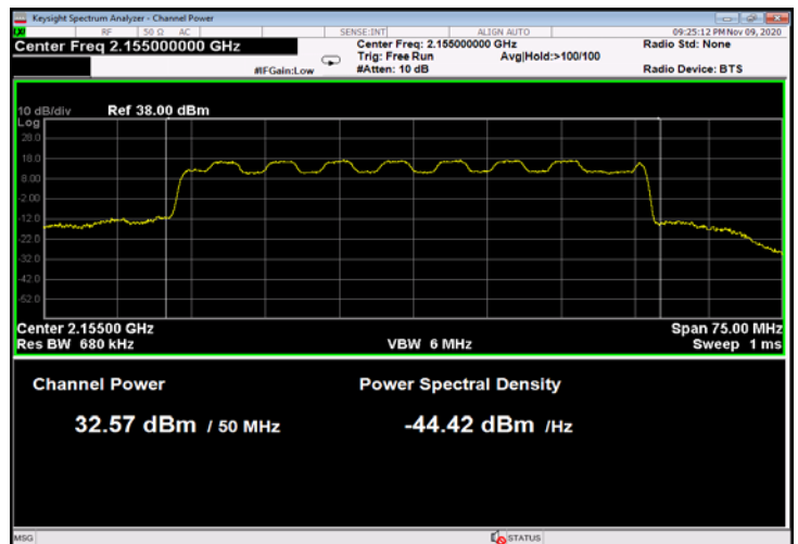
Figure 68: 16QAM 50MHz B.W.; 2155.0MHz, 60kHz
