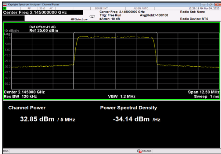
Figure 77: 64QAM 5MHz B.W.; 2145MHz, 15kHz
