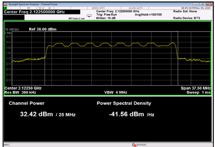
Figure 42: 16QAM 25MHz B.W.; 2122.5MHz, 15kHz
