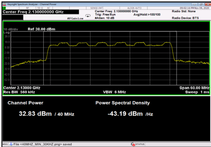
Figure 53: 16QAM 40MHz B.W.; 2130.0MHz, 60kHz
