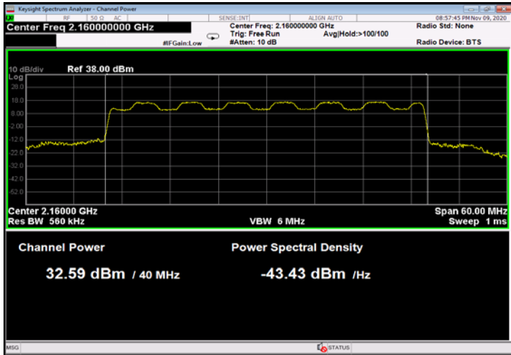
Figure 57: 16QAM 40MHz B.W.; 2160.0MHz, 15kHz
