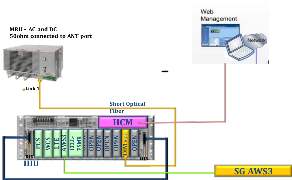
Figure 2. Radiated Test Set-Up
