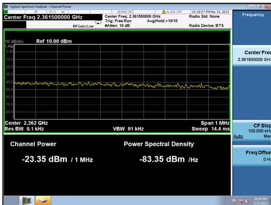
Figure 70. — 2361 MHz-2362MHz – W-CDMA
