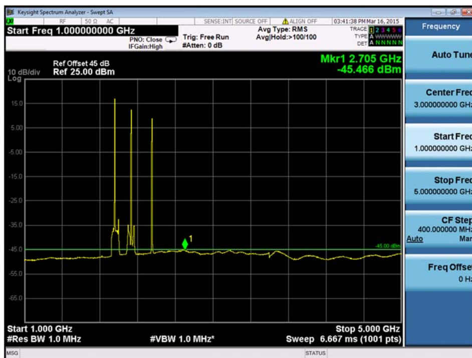
Figure 90 1000M-5000M
