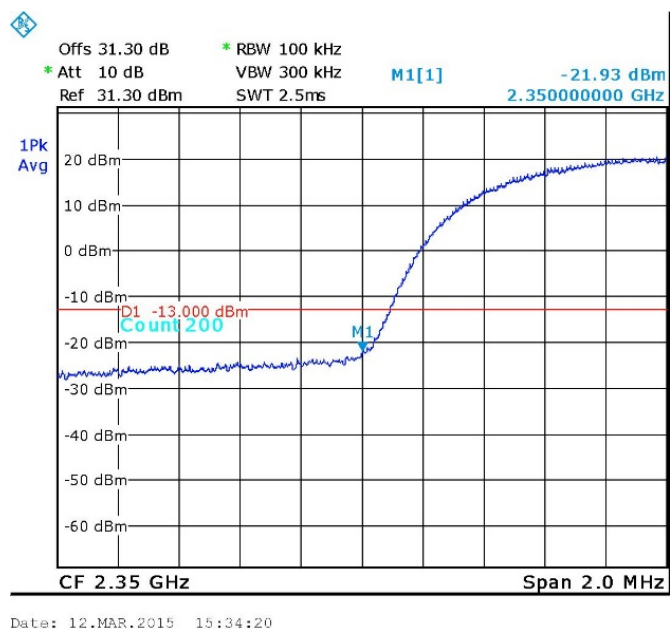
Figure 83. — Lower Block Edge -1MHz – W-CDMA
