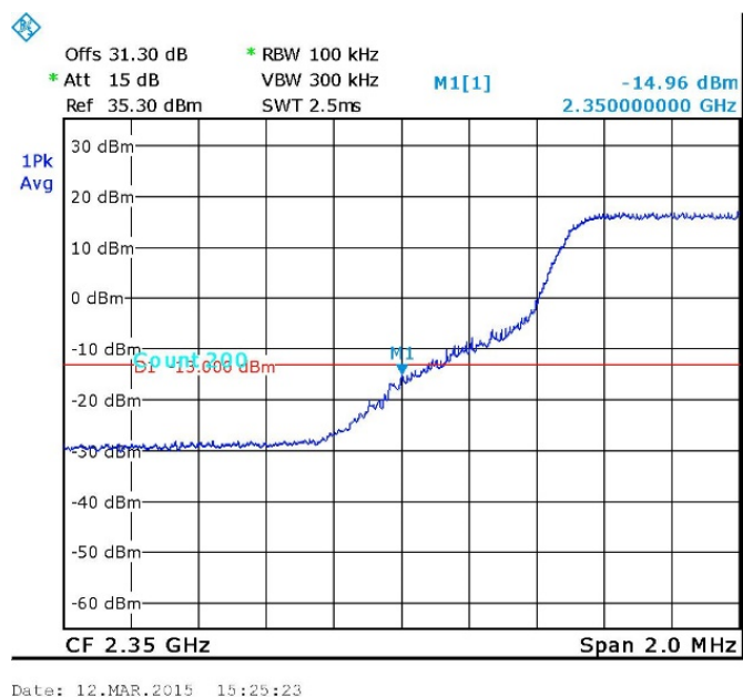
Figure 79. — Lower Block Edge -1MHz – LTE 64QAM
