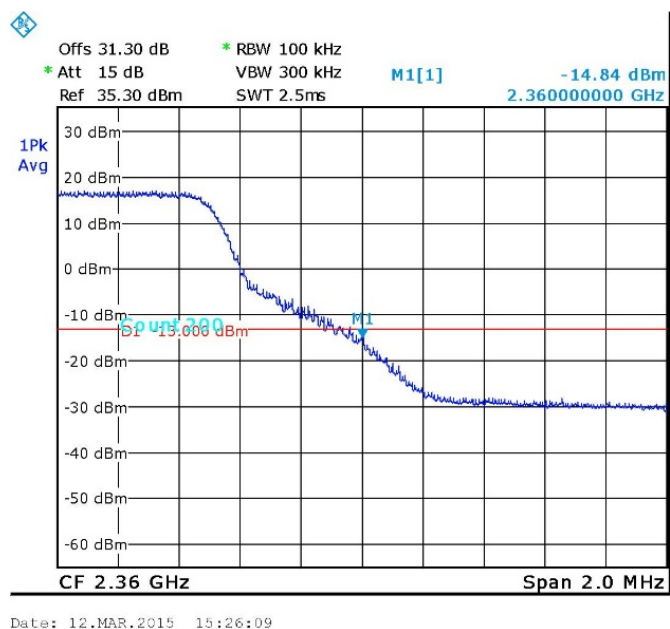
Figure 80. — Upper Band Edge +1MHz – LTE 64QAM
