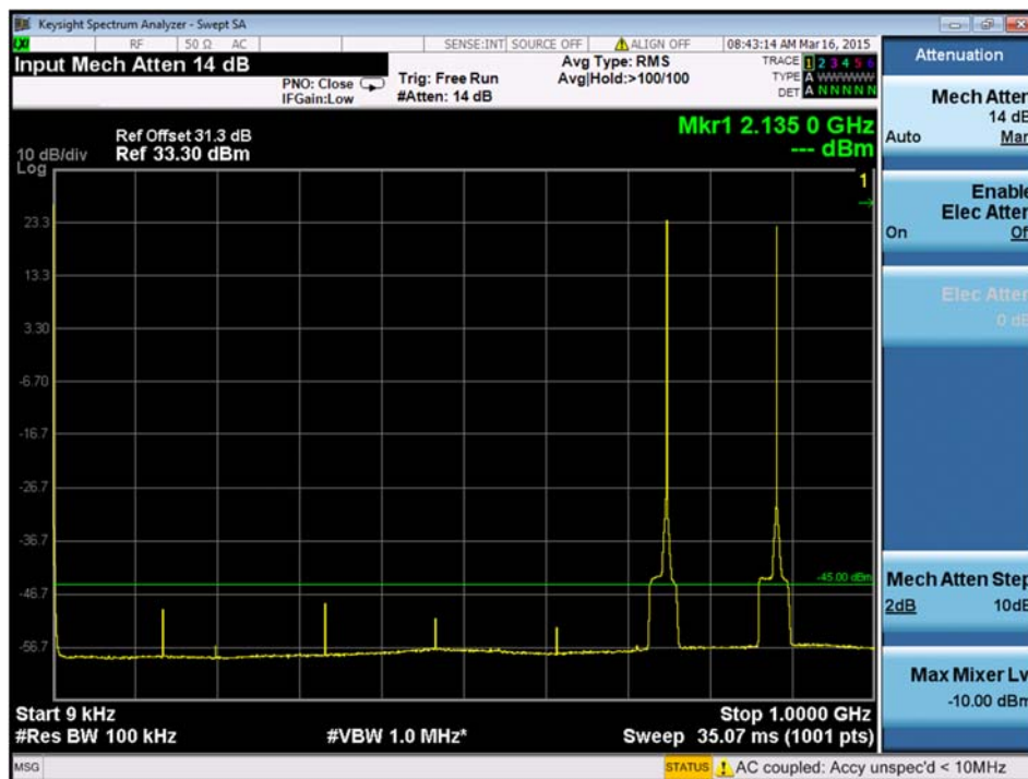
Figure 89 0.009M-1000M
