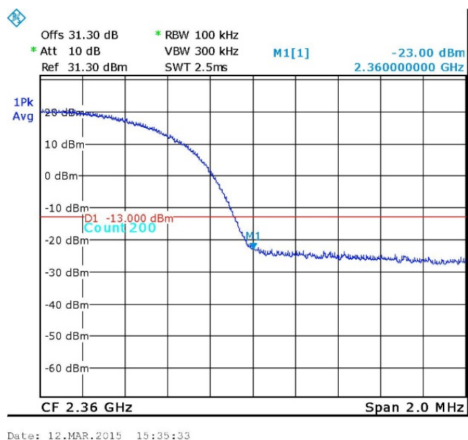
Figure 84. — Upper Band Edge +1MHz – W-CDMA
