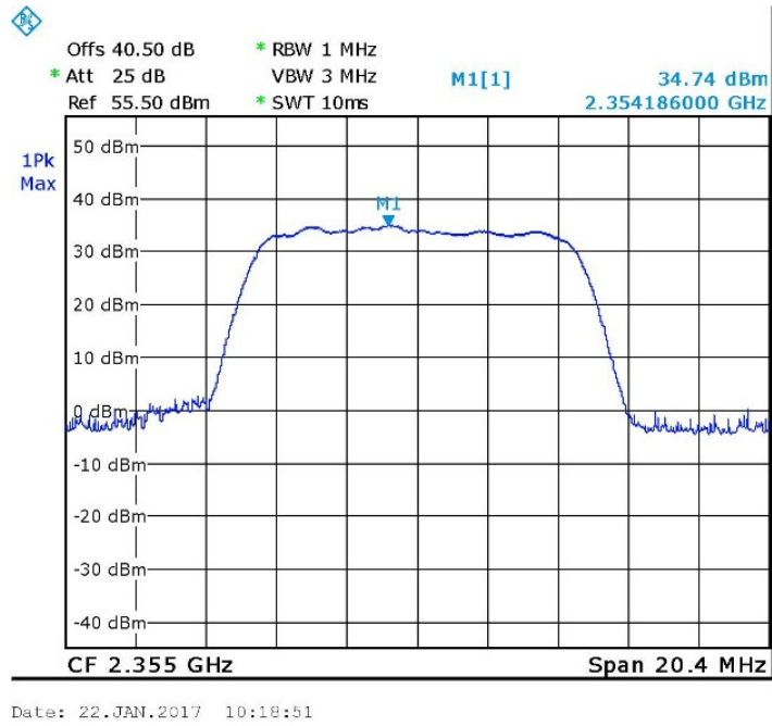
Figure 18. — 2355.0 MHz –64QAM
