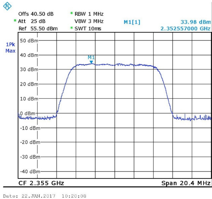
Figure 19. — 2355.0 MHz –16QAM
