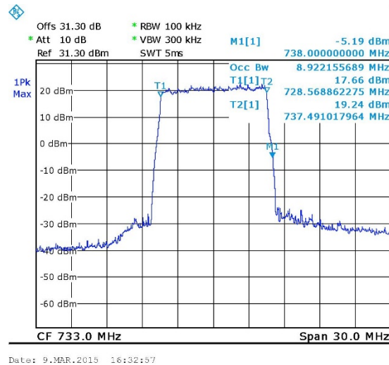
Figure 32. — QPSK 733 MHz OUT
