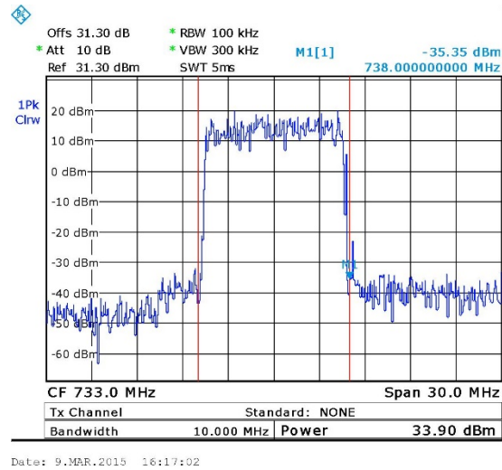
Figure 14. — QPSK 733 MHz
