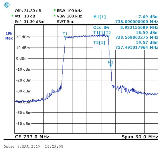
Figure 20. — 64QAM 733 MHz OUT
