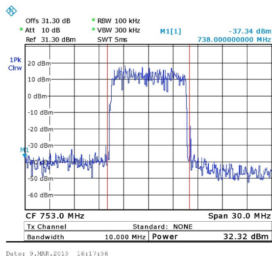
Figure 16. — QPSK 753 MHz
