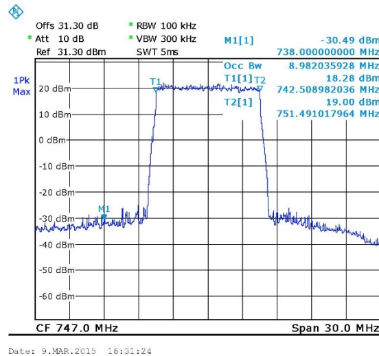
Figure 28. — 16QAM 747 MHz OUT
