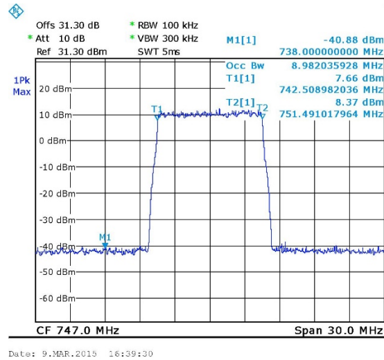
Figure 21. — 64QAM 747 MHz IN
