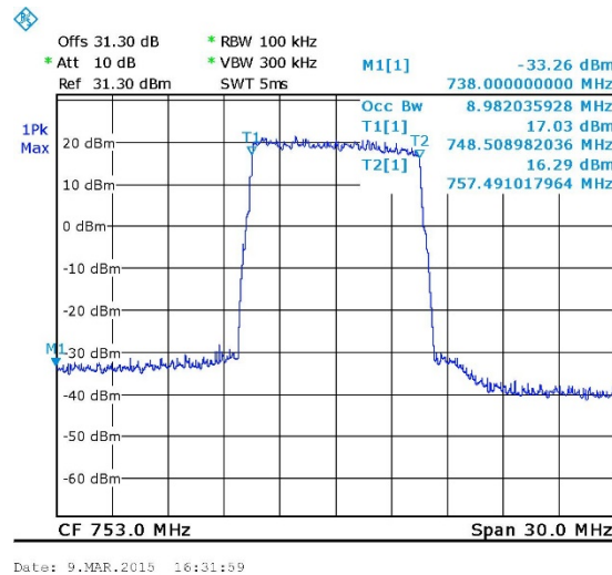
Figure 30. — 16QAM 753 MHz OUT
