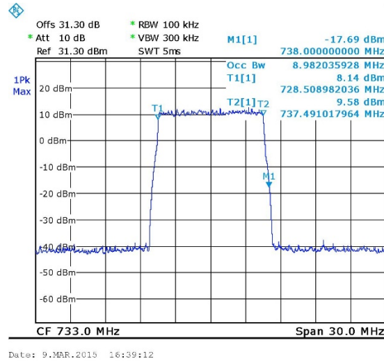
Figure 19. — 64QAM 733 MHz IN
