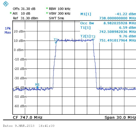
Figure 27. — 16QAM 747 MHz IN
