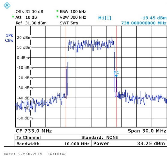
Figure 11. — 16QAM 733 MHz
