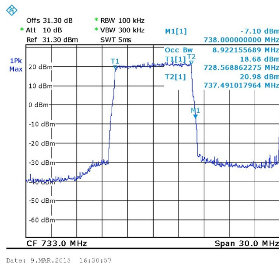
Figure 26. — 16QAM 733 MHz OUT
