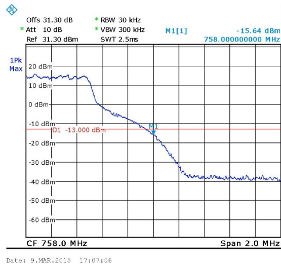
Figure 54. — QPSK 753.0 MHz
