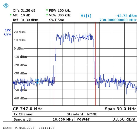
Figure 12. — 16QAM 747 MHz
