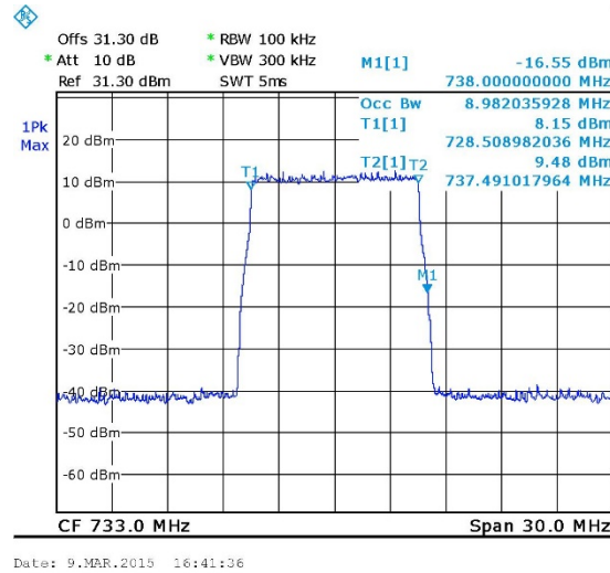
Figure 25. — 16QAM 733 MHz IN
