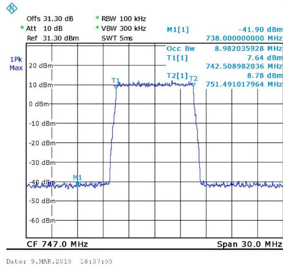
Figure 33. — QPSK 747 MHz IN
