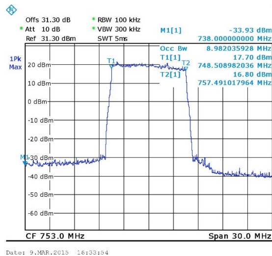
Figure 36. — QPSK 753 MHz OUT
