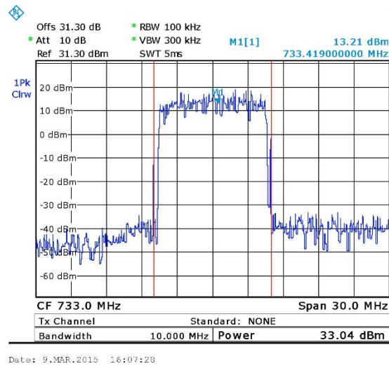
Figure 8. — 64QAM, 733 MHz
