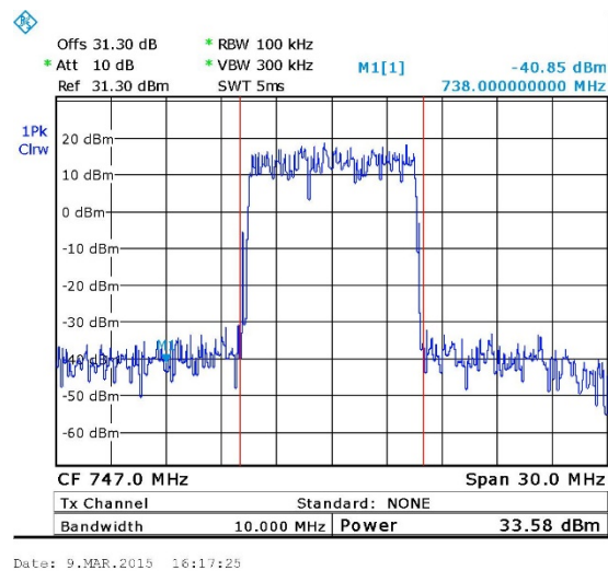
Figure 15. — QPSK 747 MHz
