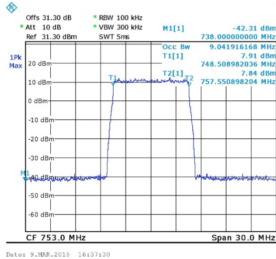
Figure 35. — QPSK 753 MHz IN
