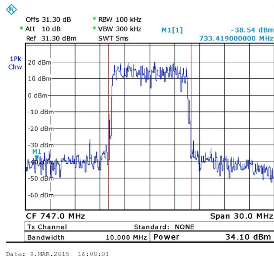
Figure 9. — 64QAM 747 MHz
