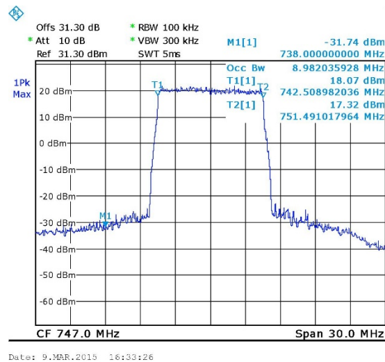
Figure 34. — QPSK 747 MHz OUT
