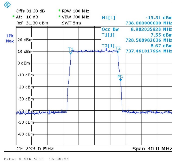
Figure 31. — QPSK 733 MHz IN
