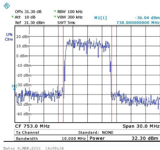
Figure 10. — 64QAM 753 MHz
