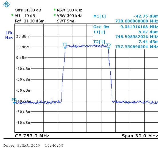
Figure 29. — 16QAM 753 MHz IN
