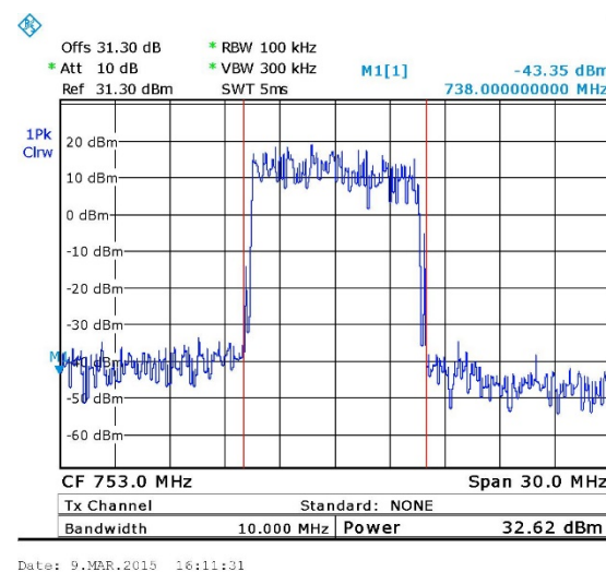
Figure 13. — 16QAM 753 MHz
