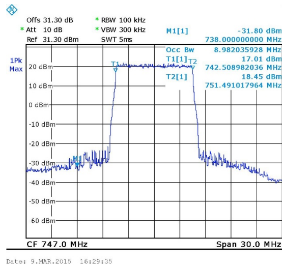
Figure 22. — 64QAM 747 MHz OUT
