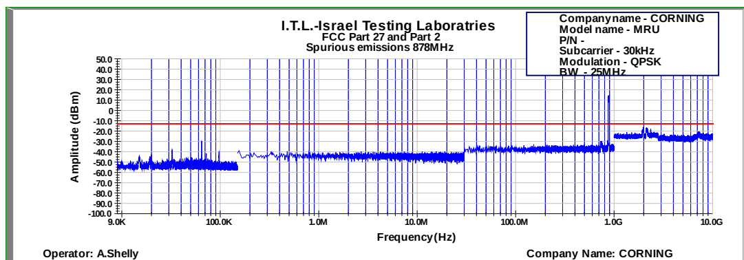
Figure 675: Spurious Emissions at Antenna Terminal QPSK 25MHz B.W.; 878.5MHz, 30kHz
