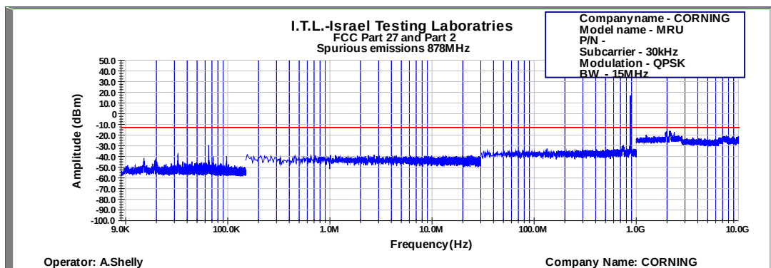
Figure 657: Spurious Emissions at Antenna Terminal QPSK 15MHz B.W.; 878.0MHz, 30kHz
