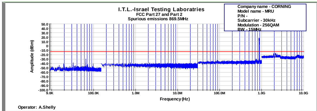
Figure 612: Spurious Emissions at Antenna Terminal 256QAM 15MHz B.W.; 869.5MHz, 30kHz
