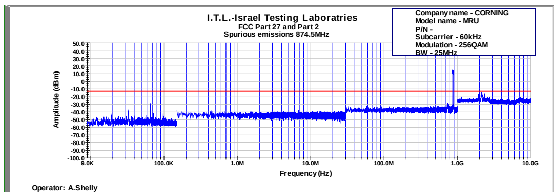
Figure 631: Spurious Emissions at Antenna Terminal 256QAM 25MHz B.W.; 874.5MHz, 60kHz
