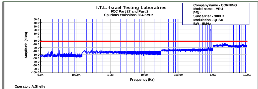
Figure 639: Spurious Emissions at Antenna Terminal QPSK 5MHz B.W.; 864.5MHz, 30kHz
