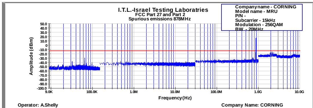
Figure 623: Spurious Emissions at Antenna Terminal 256QAM 20MHz B.W.; 878.0MHz, 15kHz
