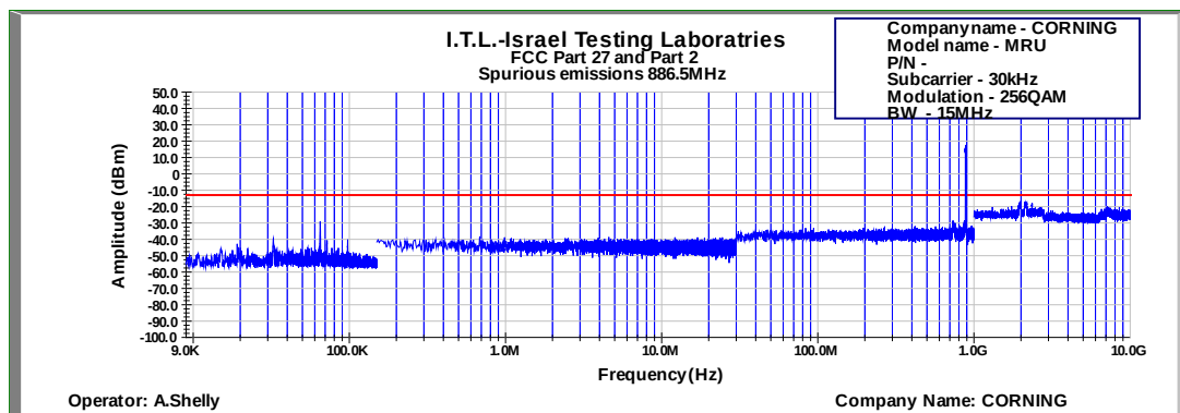
Figure 618: Spurious Emissions at Antenna Terminal 256QAM 15MHz B.W.; 886.5MHz, 30kHz
