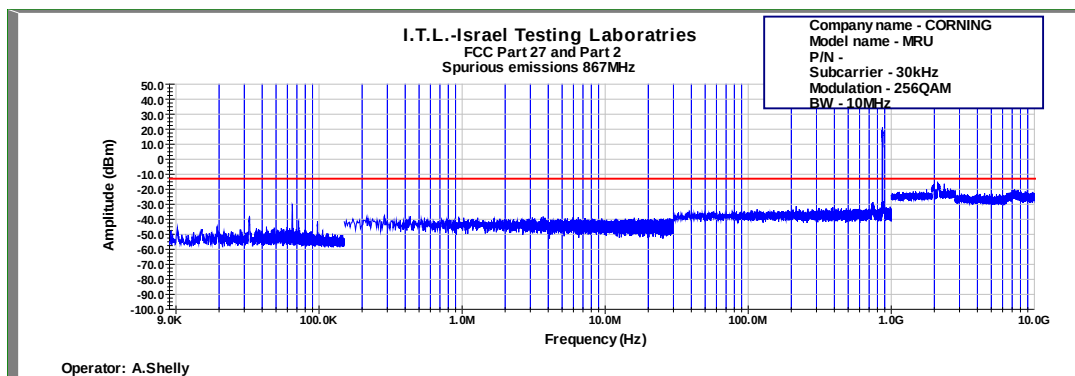
Figure 603: Spurious Emissions at Antenna Terminal 256QAM 10MHz B.W.; 867.0MHz, 30kHz
