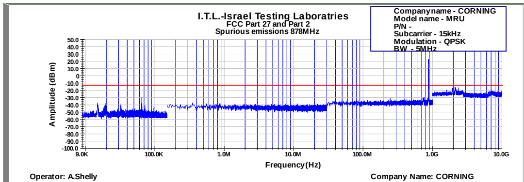
Figure 640: Spurious Emissions at Antenna Terminal QPSK 5MHz B.W.; 878.0MHz, 15kHz
