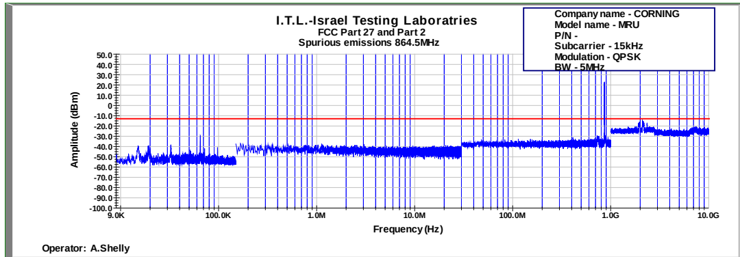
Figure 638: Spurious Emissions at Antenna Terminal QPSK 5MHz B.W.; 864.5MHz, 15kHz
