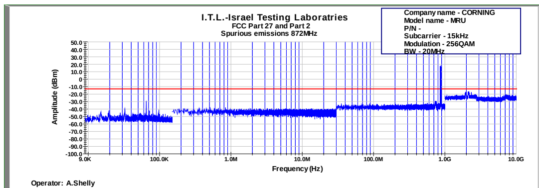
Figure 620: Spurious Emissions at Antenna Terminal 256QAM 20MHz B.W.; 872.0MHz, 15kHz
