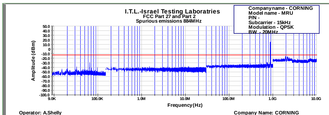
Figure 668: Spurious Emissions at Antenna Terminal QPSK 20MHz B.W.; 884.0MHz, 15kHz
