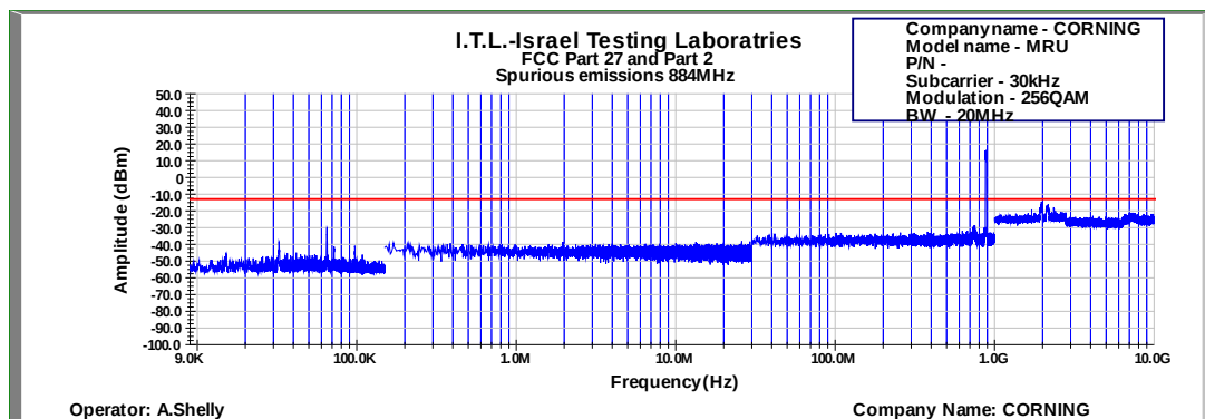
Figure 627: Spurious Emissions at Antenna Terminal 256QAM 20MHz B.W.; 884.0MHz, 30kHz
