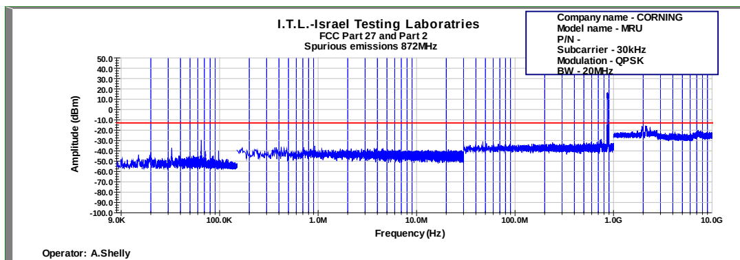
Figure 663: Spurious Emissions at Antenna Terminal QPSK 20MHz B.W.; 872.0MHz, 30kHz
