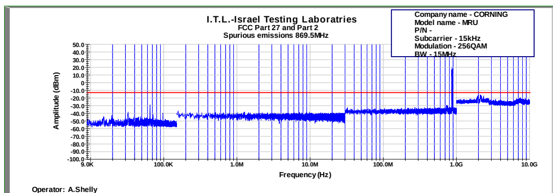
Figure 611: Spurious Emissions at Antenna Terminal 256QAM 15MHz B.W.; 869.5MHz, 15kHz
