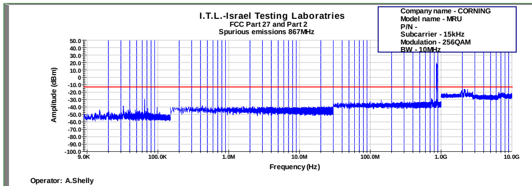
Figure 602: Spurious Emissions at Antenna Terminal 256QAM 10MHz B.W.; 867.0MHz, 15kHz
