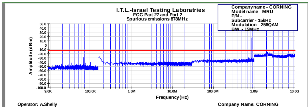
Figure 614: Spurious Emissions at Antenna Terminal 256QAM 15MHz B.W.; 878.0MHz, 15kHz
