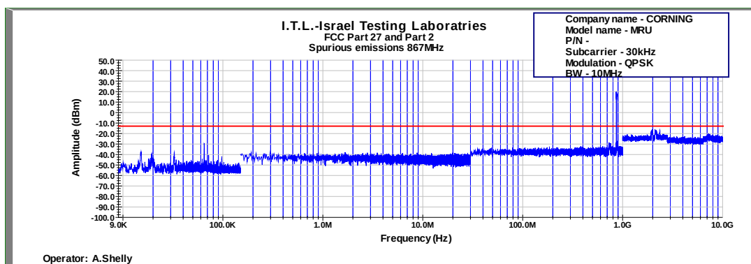
Figure 645: Spurious Emissions at Antenna Terminal QPSK 10MHz B.W.; 867.0MHz, 30kHz
