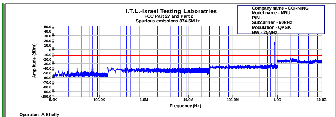
Figure 673: Spurious Emissions at Antenna Terminal QPSK 25MHz B.W.; 874.5MHz, 60kHz
