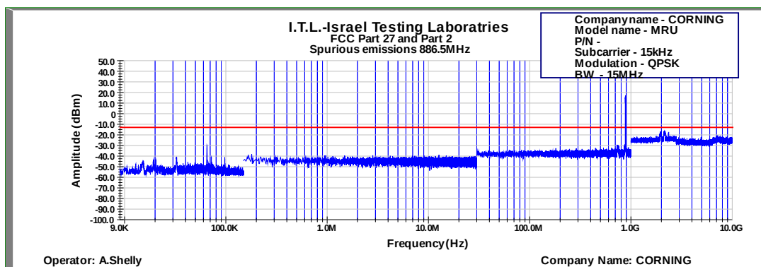
Figure 659: Spurious Emissions at Antenna Terminal QPSK 15MHz B.W.; 886.5MHz, 15kHz
