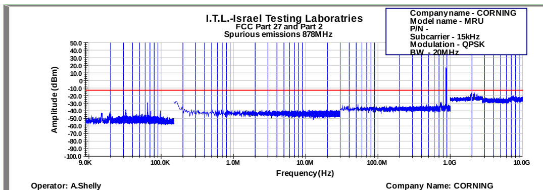
Figure 665: Spurious Emissions at Antenna Terminal QPSK 20MHz B.W.; 878.0MHz, 15kHz
