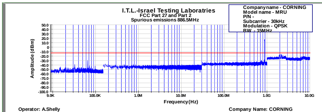
Figure 660: Spurious Emissions at Antenna Terminal QPSK 15MHz B.W.; 886.5MHz, 30kHz
