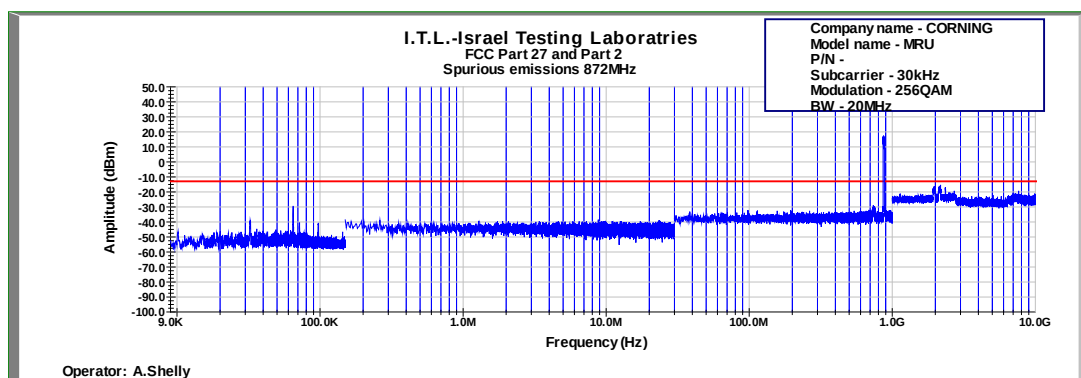
Figure 621: Spurious Emissions at Antenna Terminal 256QAM 20MHz B.W.; 872.0MHz, 30kHz
