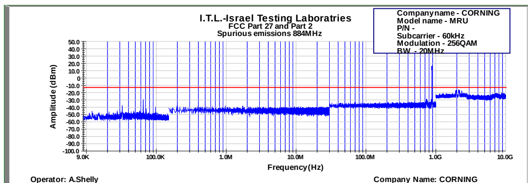
Figure 628: Spurious Emissions at Antenna Terminal 256QAM 20MHz B.W.; 884.0MHz, 60kHz
