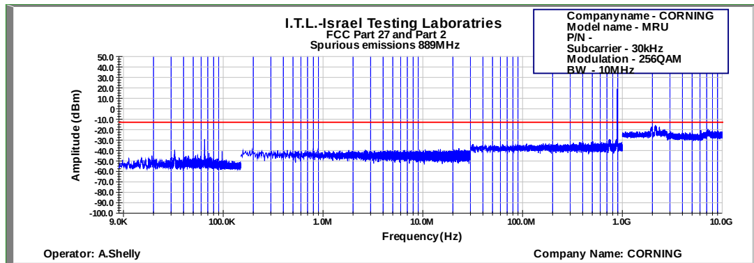
Figure 609: Spurious Emissions at Antenna Terminal 256QAM 10MHz B.W.; 889.0MHz, 30kHz
