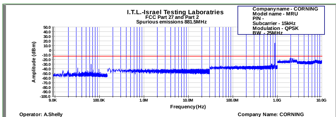
Figure 677: Spurious Emissions at Antenna Terminal QPSK 25MHz B.W.; 881.5MHz, 15kHz
