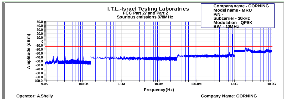
Figure 648: Spurious Emissions at Antenna Terminal QPSK 10MHz B.W.; 878.0MHz, 30kHz
