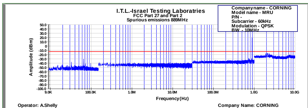
Figure 652: Spurious Emissions at Antenna Terminal QPSK 10MHz B.W.; 889.0MHz, 60kHz
