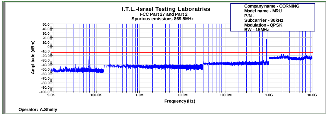
Figure 654: Spurious Emissions at Antenna Terminal QPSK 15MHz B.W.; 869.5MHz, 30kHz
