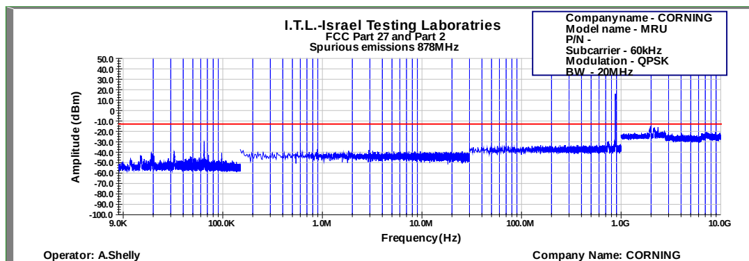
Figure 667: Spurious Emissions at Antenna Terminal QPSK 20MHz B.W.; 878.0MHz, 60kHz
