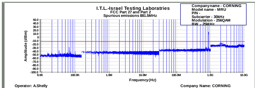
Figure 636: Spurious Emissions at Antenna Terminal 256QAM 25MHz B.W.; 881.5MHz, 30kHz
