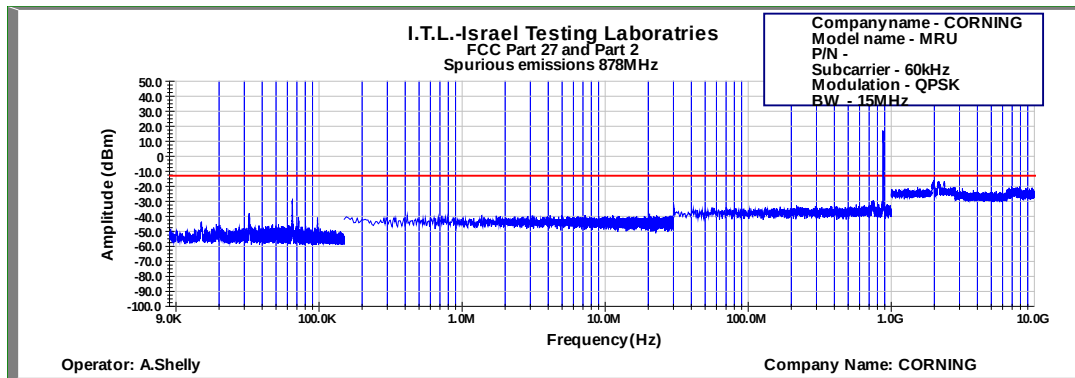
Figure 658: Spurious Emissions at Antenna Terminal QPSK 15MHz B.W.; 878.0MHz, 60kHz
