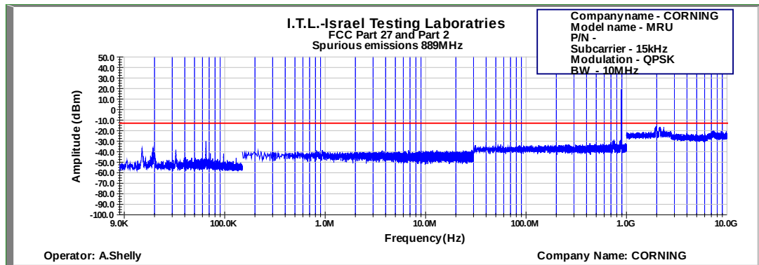
Figure 650: Spurious Emissions at Antenna Terminal QPSK 10MHz B.W.; 889.0MHz, 15kHz
