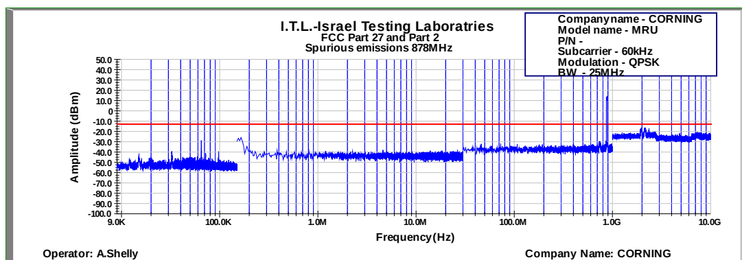
Figure 676: Spurious Emissions at Antenna Terminal QPSK 25MHz B.W.; 878.5MHz, 60kHz
