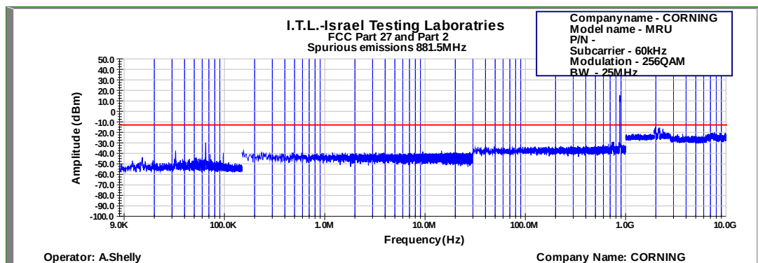
Figure 637: Spurious Emissions at Antenna Terminal 256QAM 25MHz B.W.; 881.5MHz, 60kHz
