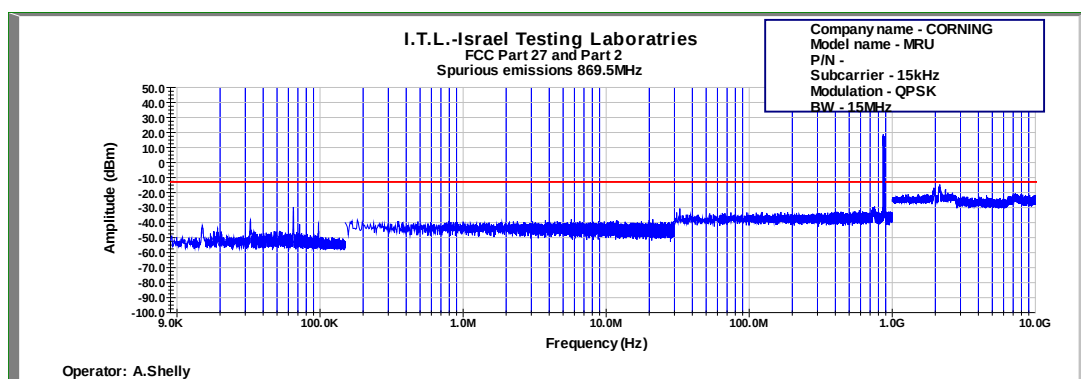
Figure 653: Spurious Emissions at Antenna Terminal QPSK 15MHz B.W.; 869.5MHz, 15kHz
