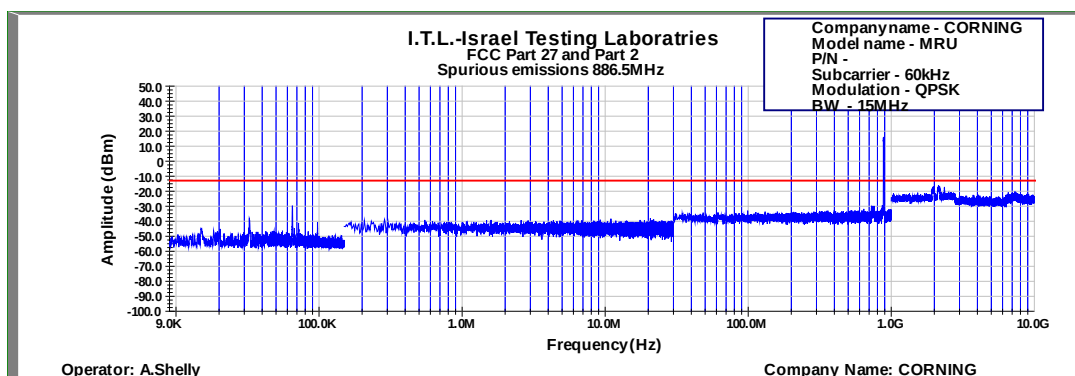
Figure 661: Spurious Emissions at Antenna Terminal QPSK 15MHz B.W.; 886.5MHz, 60kHz
