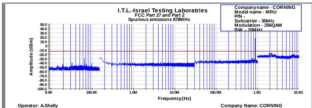
Figure 615: Spurious Emissions at Antenna Terminal 256QAM 15MHz B.W.; 878.0MHz, 30kHz
