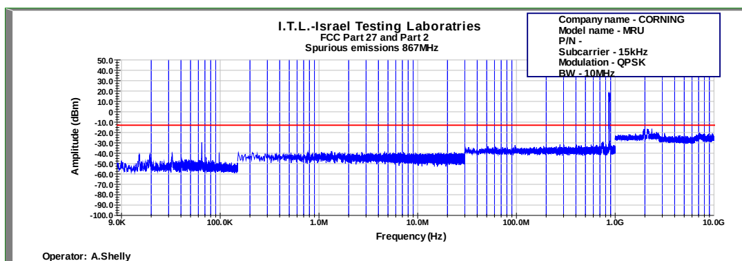
Figure 644: Spurious Emissions at Antenna Terminal QPSK 10MHz B.W.; 867.0MHz, 15kHz
