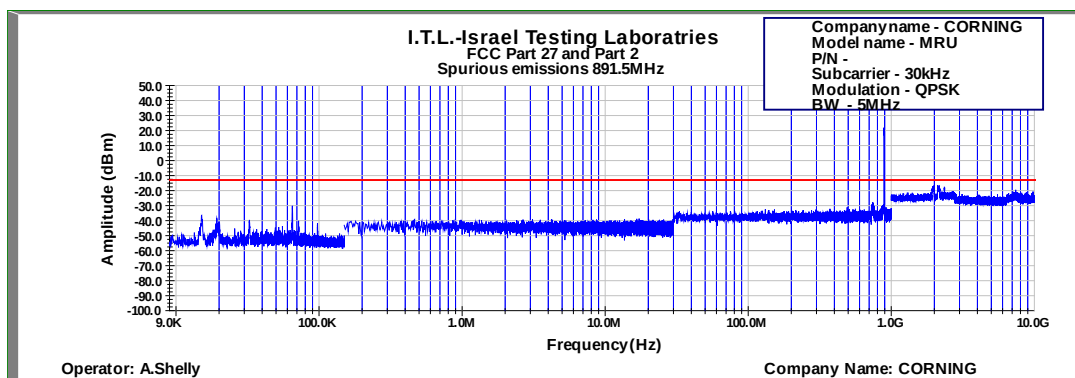
Figure 643: Spurious Emissions at Antenna Terminal QPSK 5MHz B.W.; 891.5MHz, 30kHz
