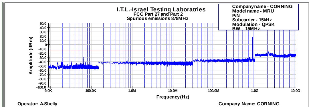
Figure 656: Spurious Emissions at Antenna Terminal QPSK 15MHz B.W.; 878.0MHz, 15kHz
