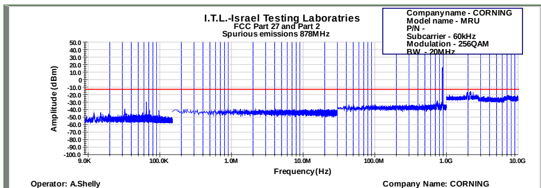
Figure 625: Spurious Emissions at Antenna Terminal 256QAM 20MHz B.W.; 878.0MHz, 60kHz
