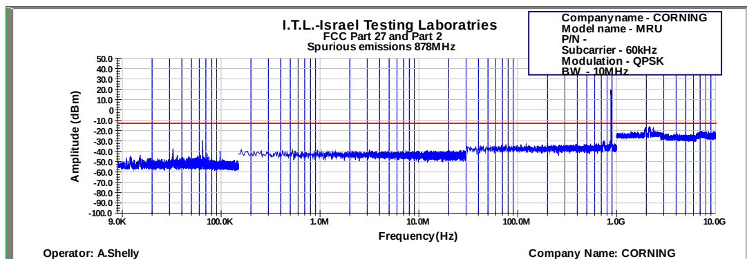
Figure 649: Spurious Emissions at Antenna Terminal QPSK 10MHz B.W.; 878.0MHz, 60kHz
