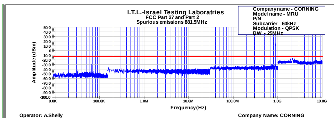
Figure 679: Spurious Emissions at Antenna Terminal QPSK 25MHz B.W.; 881.5MHz, 60kHz
