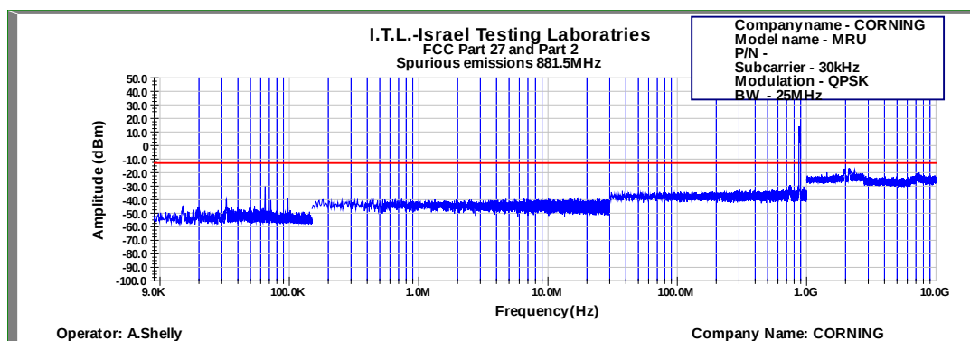
Figure 678: Spurious Emissions at Antenna Terminal QPSK 25MHz B.W.; 881.5MHz, 30kHz
