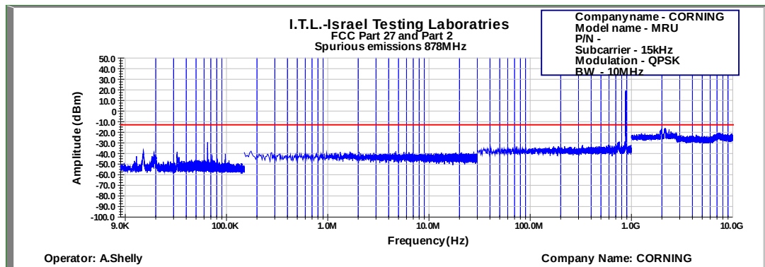
Figure 647: Spurious Emissions at Antenna Terminal QPSK 10MHz B.W.; 878.0MHz, 15kHz
