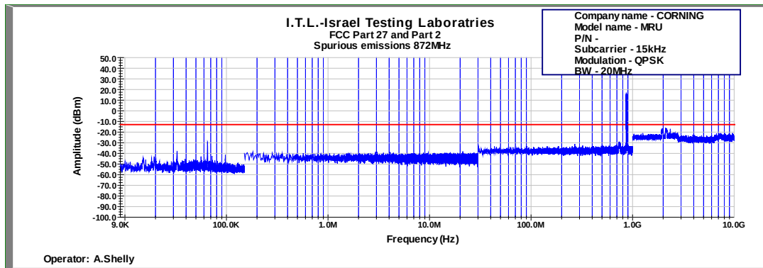
Figure 662: Spurious Emissions at Antenna Terminal QPSK 20MHz B.W.; 872.0MHz, 15kHz
