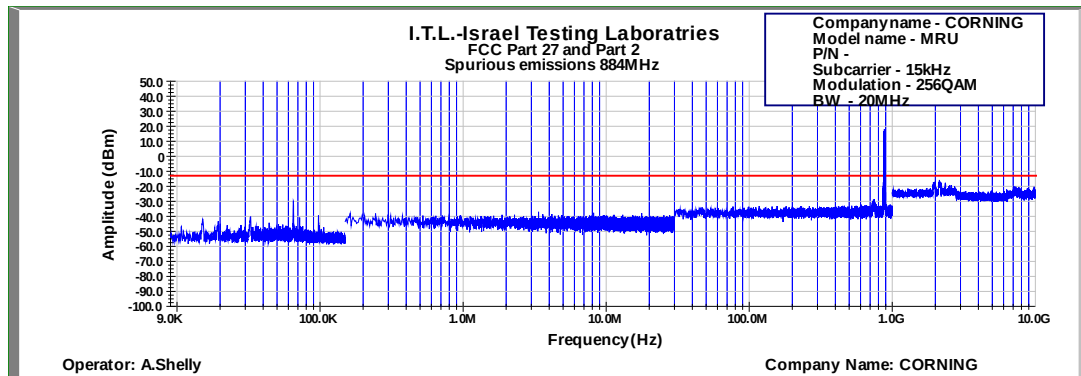
Figure 626: Spurious Emissions at Antenna Terminal 256QAM 20MHz B.W.; 884.0MHz, 15kHz
