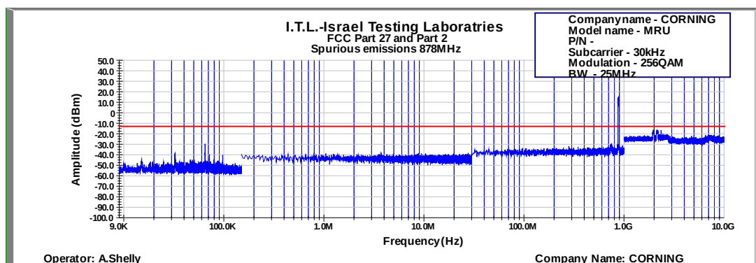
Figure 633: Spurious Emissions at Antenna Terminal 256QAM 25MHz B.W.; 878.5MHz, 30kHz
