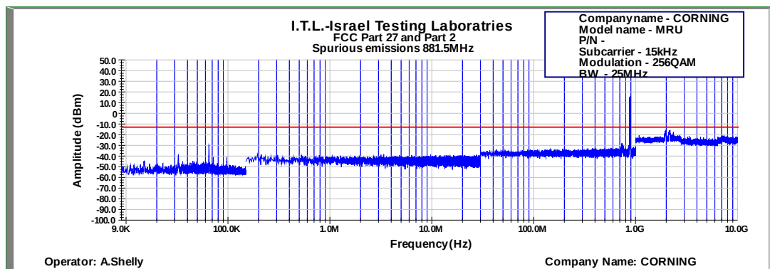
Figure 635: Spurious Emissions at Antenna Terminal 256QAM 25MHz B.W.; 881.5MHz, 15kHz
