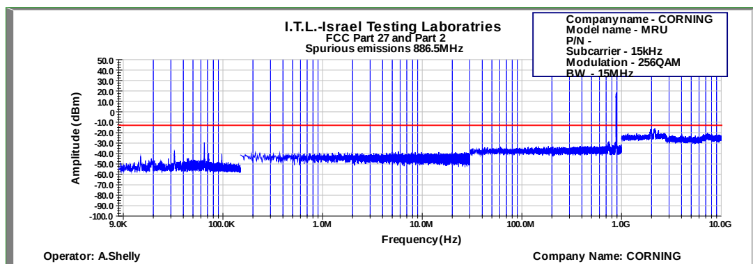
Figure 617: Spurious Emissions at Antenna Terminal 256QAM 15MHz B.W.; 886.5MHz, 15kHz
