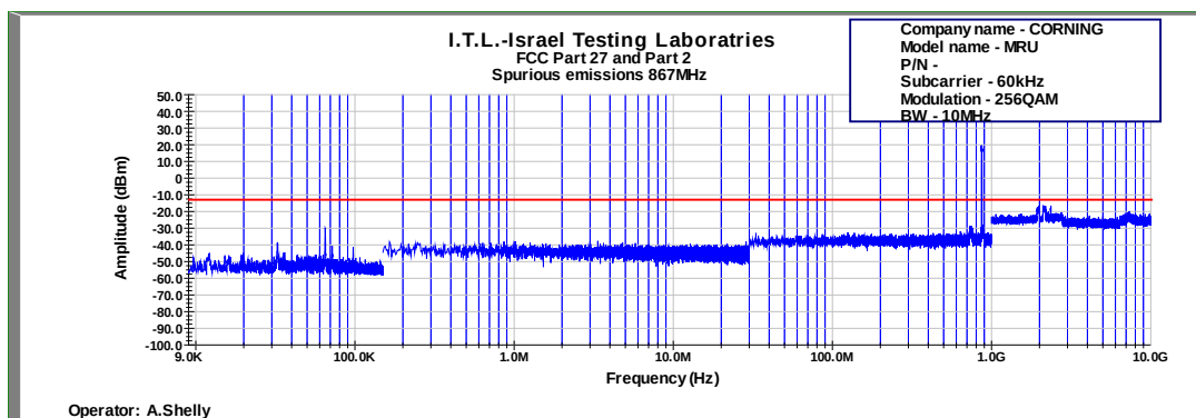
Figure 604: Spurious Emissions at Antenna Terminal 256QAM 10MHz B.W.; 867.0MHz, 60kHz
