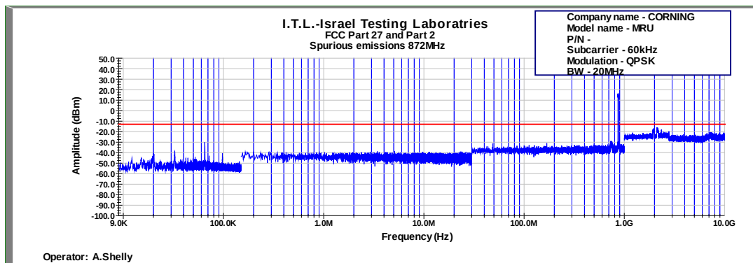
Figure 664: Spurious Emissions at Antenna Terminal QPSK 20MHz B.W.; 872.0MHz, 60kHz
