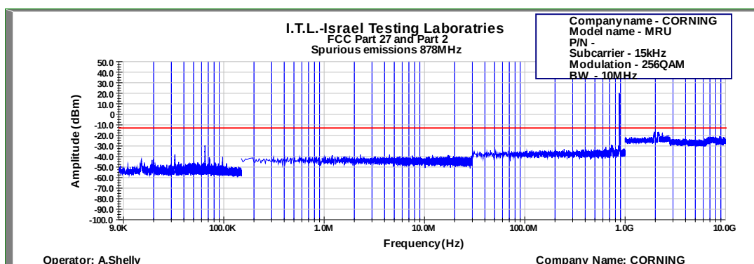
Figure 605: Spurious Emissions at Antenna Terminal 256QAM 10MHz B.W.; 878.0MHz, 15kHz
