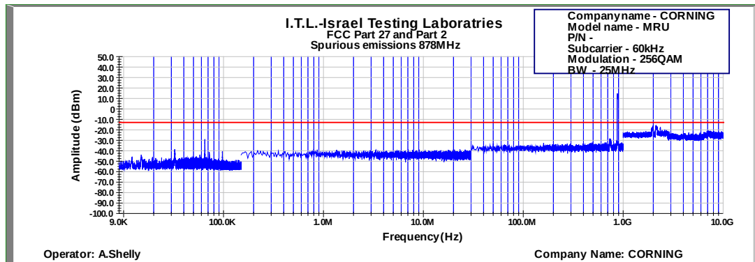
Figure 634: Spurious Emissions at Antenna Terminal 256QAM 25MHz B.W.; 878.5MHz, 60kHz
