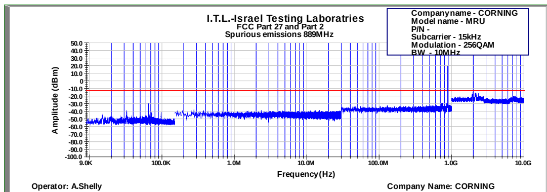
Figure 608: Spurious Emissions at Antenna Terminal 256QAM 10MHz B.W.; 889.0MHz, 15kHz
