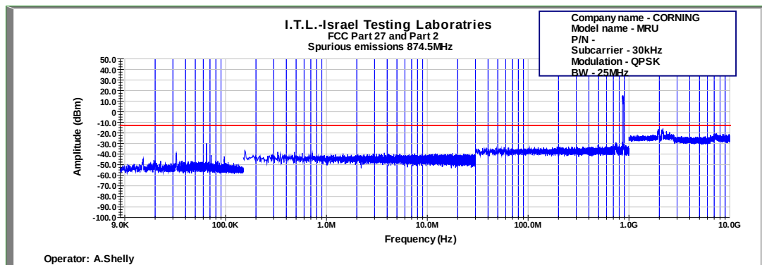
Figure 672: Spurious Emissions at Antenna Terminal QPSK 25MHz B.W.; 874.5MHz, 30kHz
