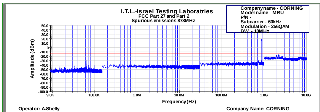
Figure 607: Spurious Emissions at Antenna Terminal 256QAM 10MHz B.W.; 878.0MHz, 60kHz
