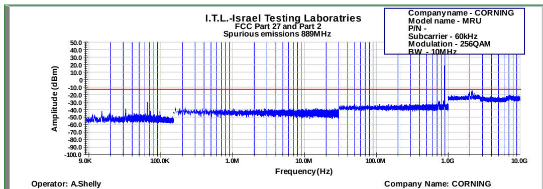
Figure 610: Spurious Emissions at Antenna Terminal 256QAM 10MHz B.W.; 889.0MHz, 60kHz
