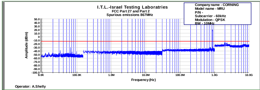
Figure 646: Spurious Emissions at Antenna Terminal QPSK 10MHz B.W.; 867.0MHz, 60kHz
