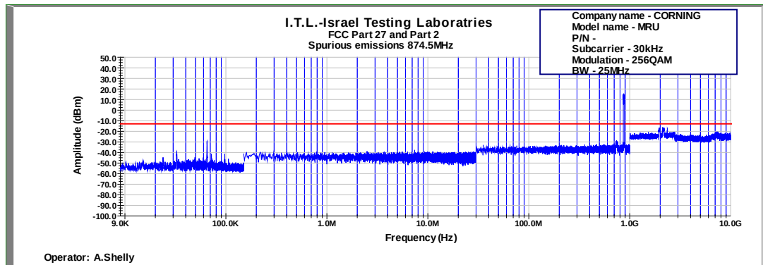
Figure 630: Spurious Emissions at Antenna Terminal 256QAM 25MHz B.W.; 874.5MHz, 30kHz
