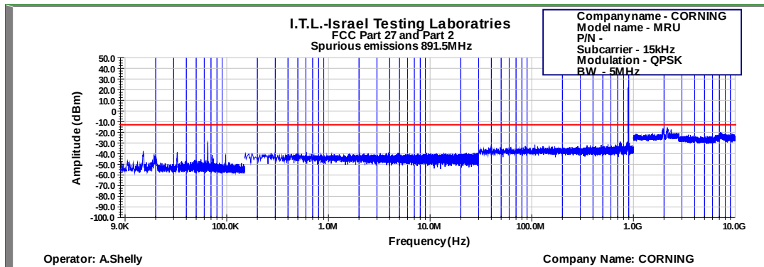
Figure 642: Spurious Emissions at Antenna Terminal QPSK 5MHz B.W.; 891.5MHz, 15kHz
