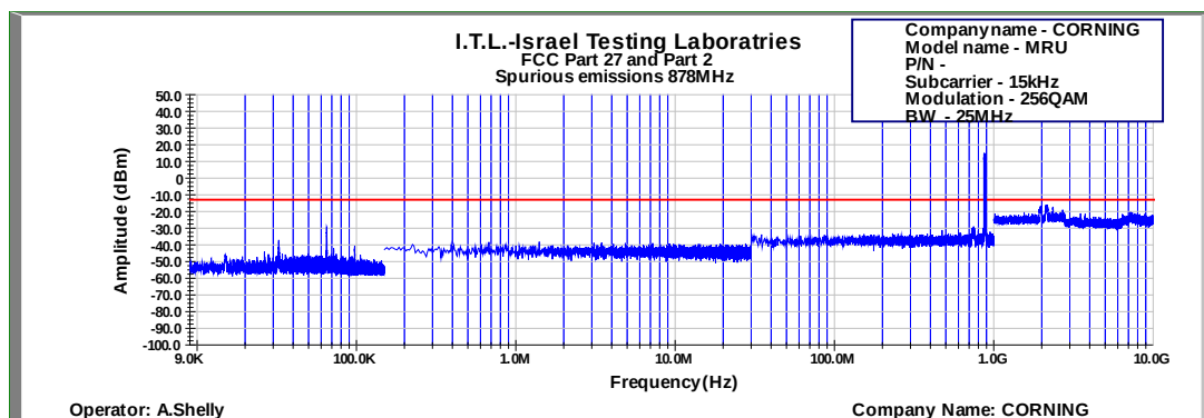
Figure 632: Spurious Emissions at Antenna Terminal 256QAM 25MHz B.W.; 878.0MHz, 15kHz
