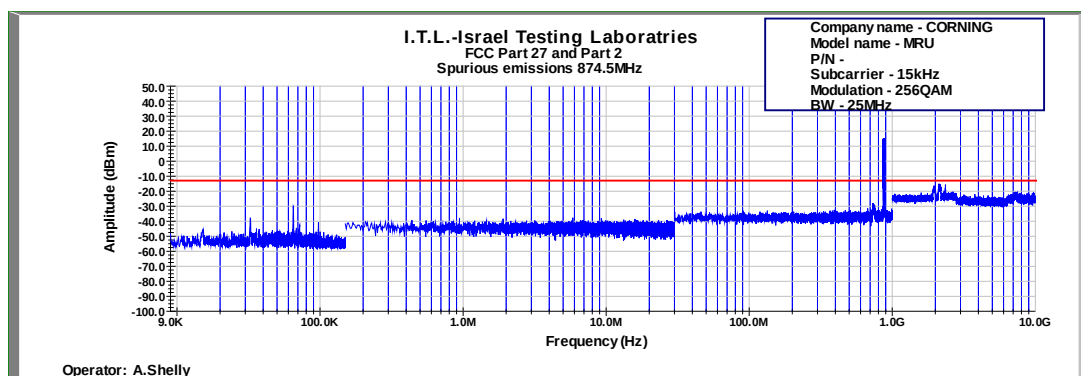
Figure 629: Spurious Emissions at Antenna Terminal 256QAM 25MHz B.W.; 874.5MHz, 15kHz
