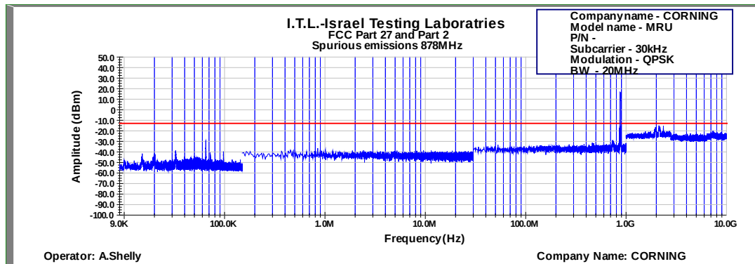
Figure 666: Spurious Emissions at Antenna Terminal QPSK 20MHz B.W.; 878.0MHz, 30kHz
