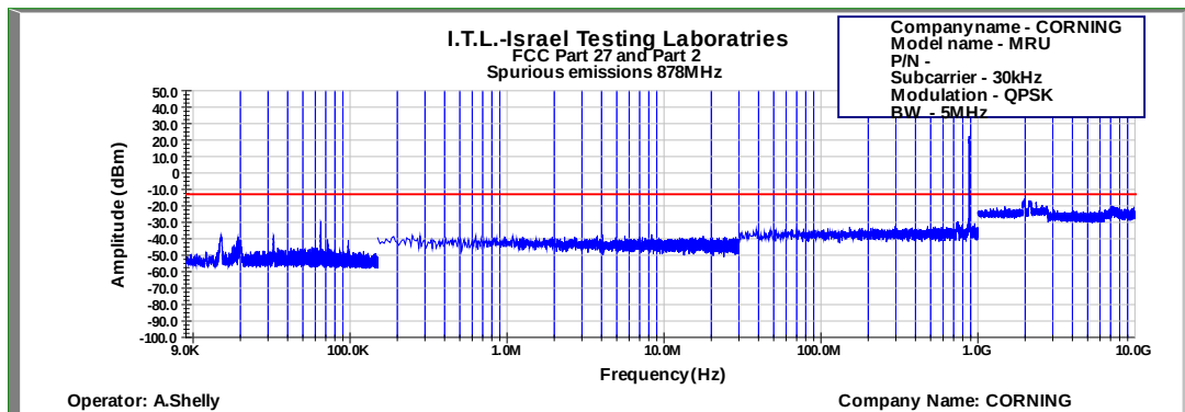
Figure 641: Spurious Emissions at Antenna Terminal QPSK 5MHz B.W.; 878.0MHz, 30kHz
