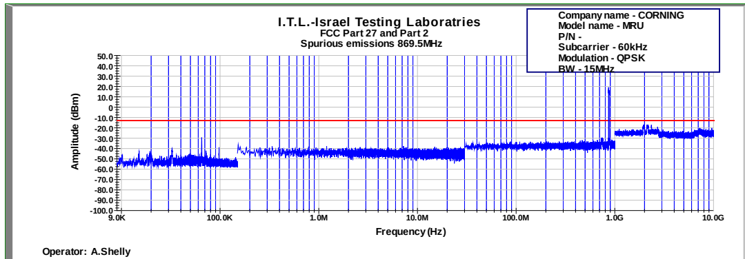
Figure 655: Spurious Emissions at Antenna Terminal QPSK 15MHz B.W.; 869.5MHz, 60kHz
