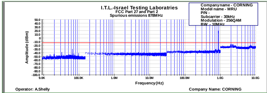
Figure 606: Spurious Emissions at Antenna Terminal 256QAM 10MHz B.W.; 878.0MHz, 30kHz
