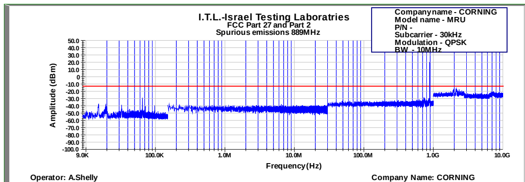
Figure 651: Spurious Emissions at Antenna Terminal QPSK 10MHz B.W.; 889.0MHz, 30kHz
