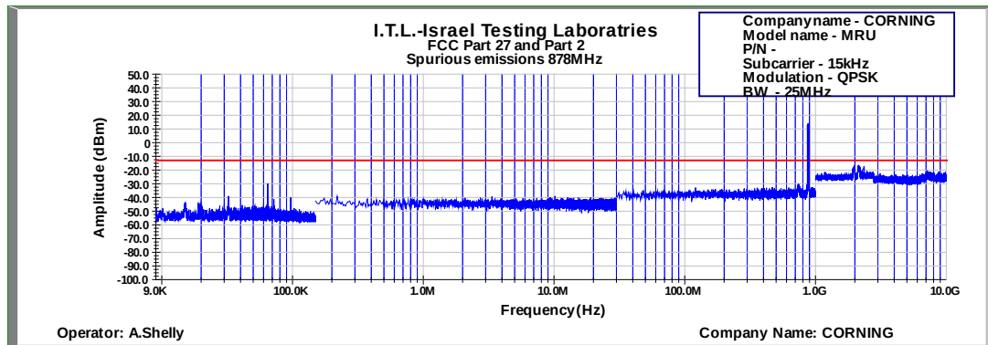
Figure 674: Spurious Emissions at Antenna Terminal QPSK 25MHz B.W.; 878.0MHz, 15kHz
