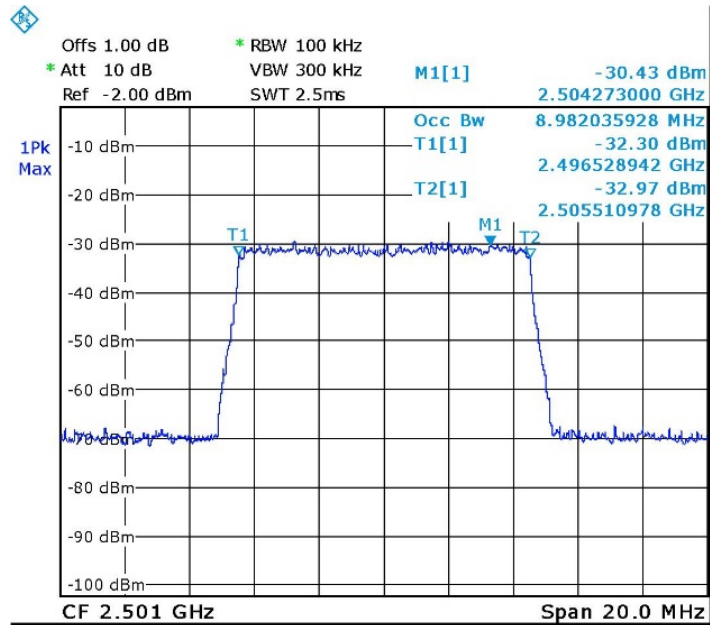
Figure 37 Occupied Bandwidth INPUT, 2501.0MHz, 16QAM
