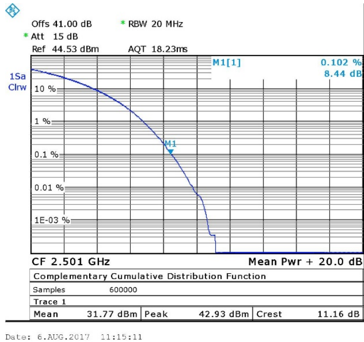
Figure 23. —16QAM, 2501.0 MHz
