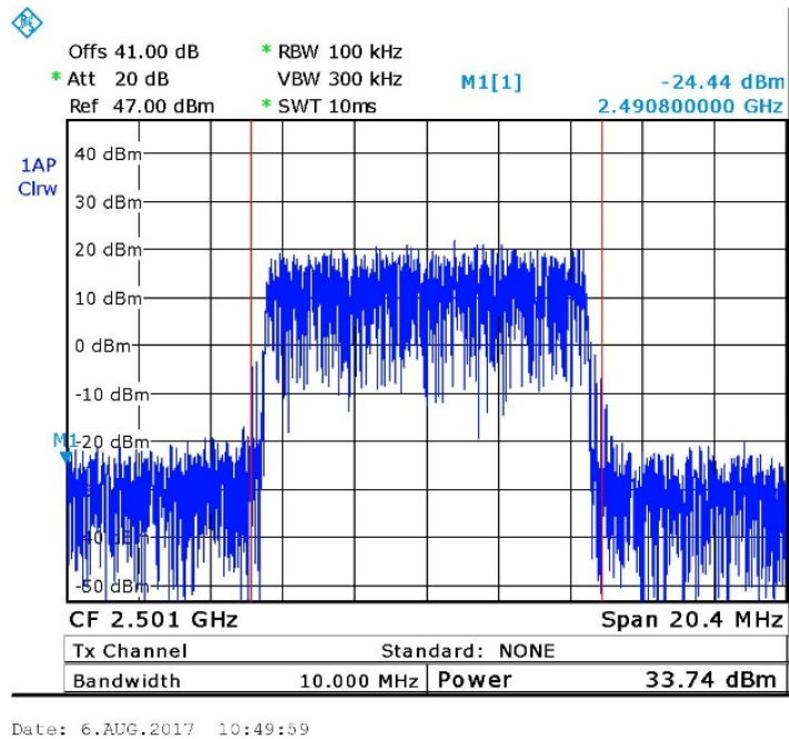
Figure 10. — 2501.0 MHz – 16QAM
