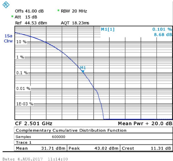
Figure 26. —QPSK, 2501.0 MHz
