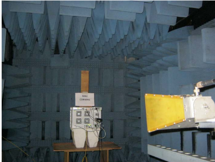
Figure 7. Radiated Emission Test – above 1GHz
