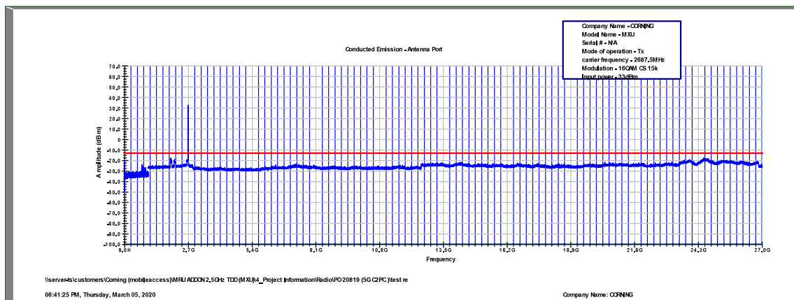
Figure 442: Spurious Emissions at Antenna Terminal 16QAM, 2687.5MHz, B.W. 5MHz, Sub Carrier 15kHz
