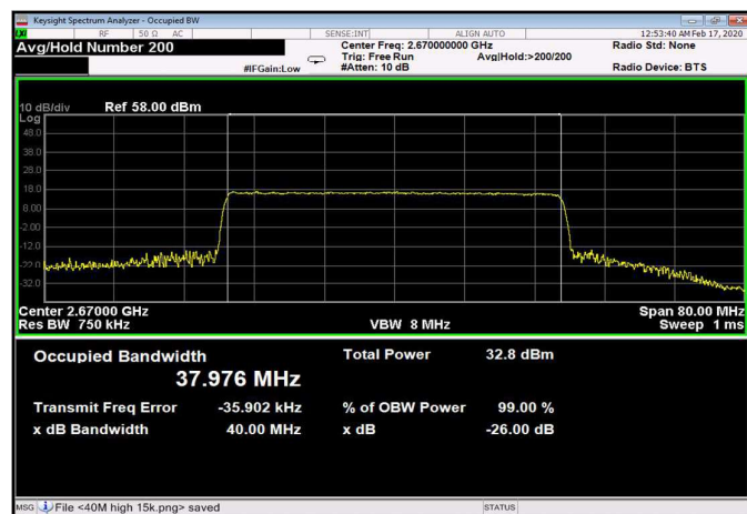
Figure 432: 256QAM 40MHz B.W.; 2670.0MHz, 30kHz Output
