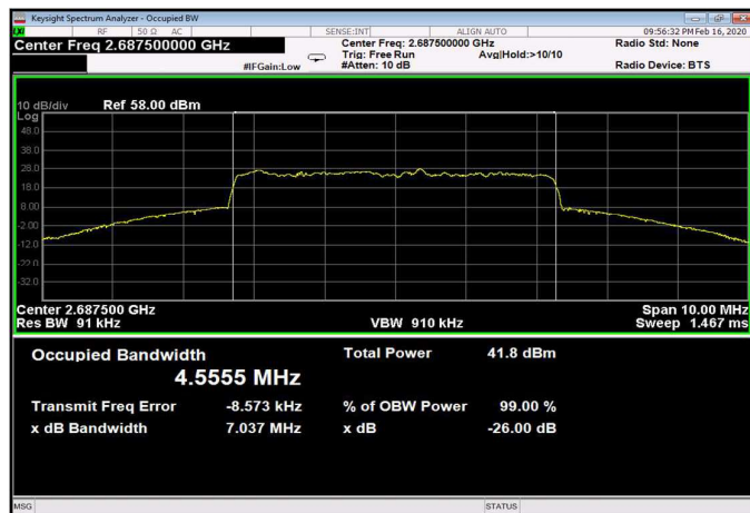
Figure 396: 256QAM 5MHz B.W.; 2687.5MHz, 15kHz Output
