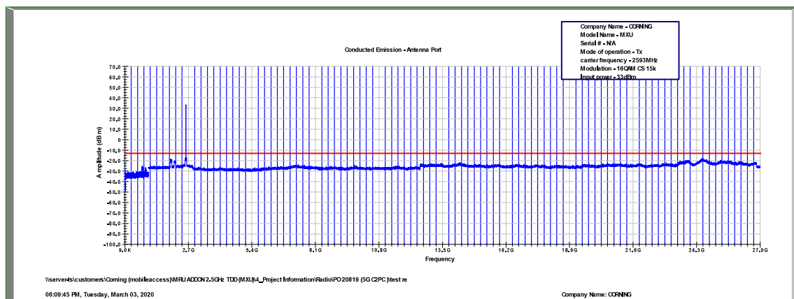
Figure 441: Spurious Emissions at Antenna Terminal 16QAM, 2593.0MHz, B.W. 5MHz, Sub Carrier 15kHz
