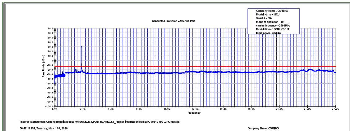
Figure 456: Spurious Emissions at Antenna Terminal 16QAM, 2593.0MHz, B.W. 15MHz, Sub Carrier 15kHz
