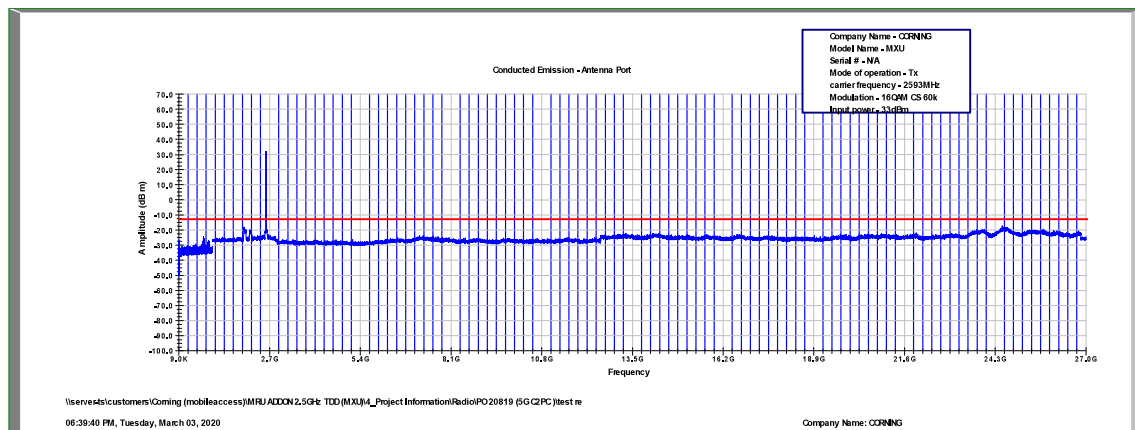
Figure 453: Spurious Emissions at Antenna Terminal 16QAM, 2593.0MHz, B.W. 10MHz, Sub Carrier 60kHz
