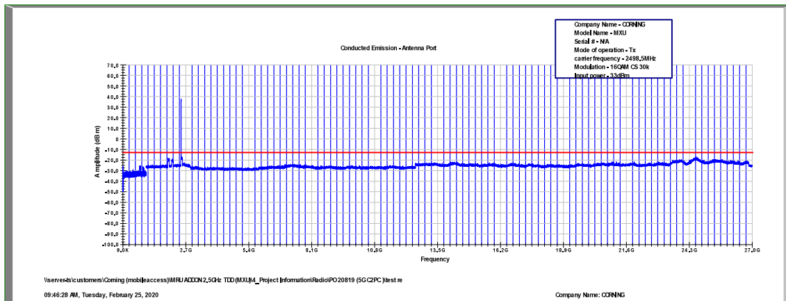
Figure 443: Spurious Emissions at Antenna Terminal 16QAM, 2498.5MHz, B.W. 5MHz, Sub Carrier 30kHz
