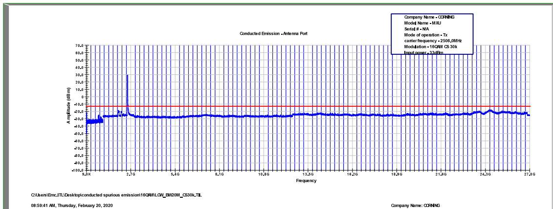
Figure 467: Spurious Emissions at Antenna Terminal 16QAM, 2506.0MHz, B.W. 20MHz, Sub Carrier 30kHz
