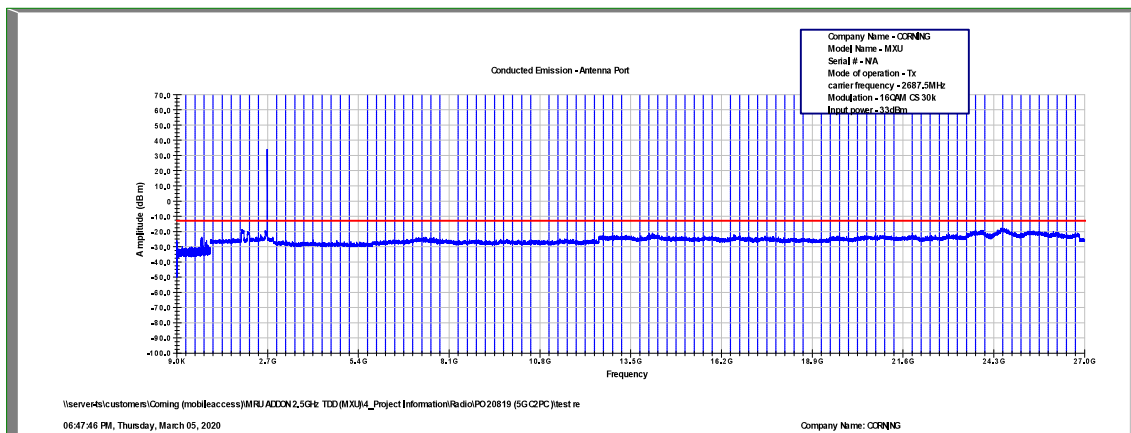
Figure 445: Spurious Emissions at Antenna Terminal 16QAM, 2687.5MHz, B.W. 5MHz, Sub Carrier 30kHz
