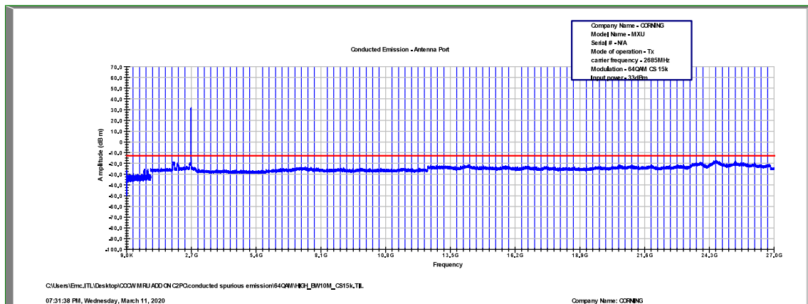
Figure 496: Spurious Emissions at Antenna Terminal 64QAM, 2685.0MHz, B.W. 10MHz, Sub Carrier 15kHz
