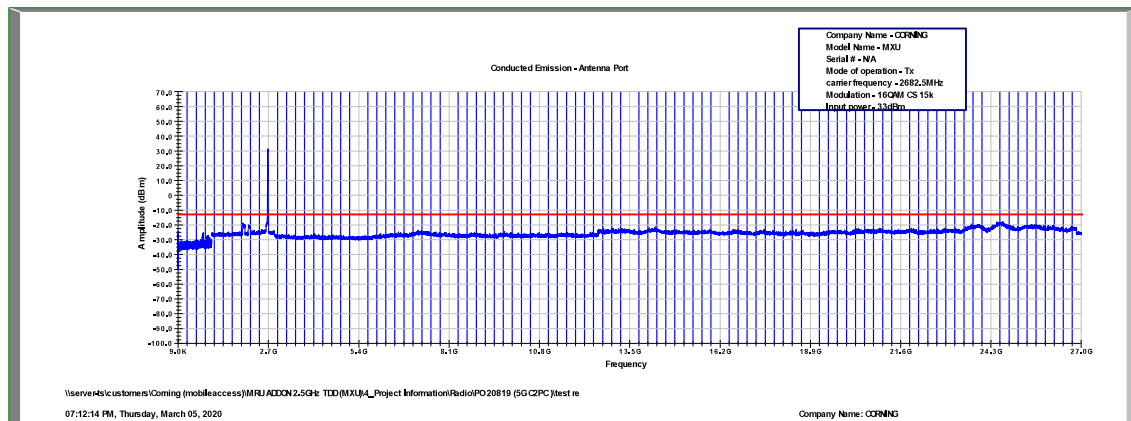
Figure 457: Spurious Emissions at Antenna Terminal 16QAM, 2682.5MHz, B.W. 15MHz, Sub Carrier 15kHz
