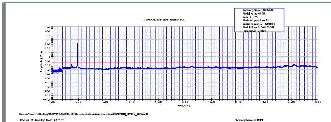
Figure 495: Spurious Emissions at Antenna Terminal 64QAM, 2593.0MHz, B.W. 10MHz, Sub Carrier 15kHz
