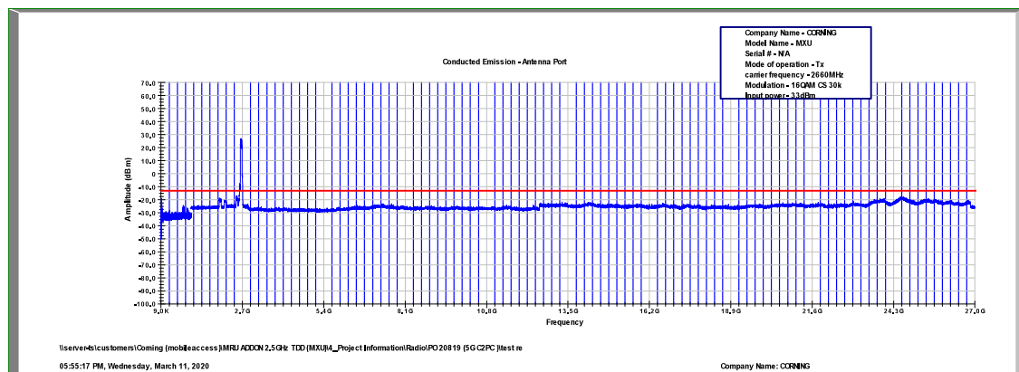
Figure 484: Spurious Emissions at Antenna Terminal 16QAM, 2660.0MHz, B.W. 60MHz, Sub Carrier 30kHz
