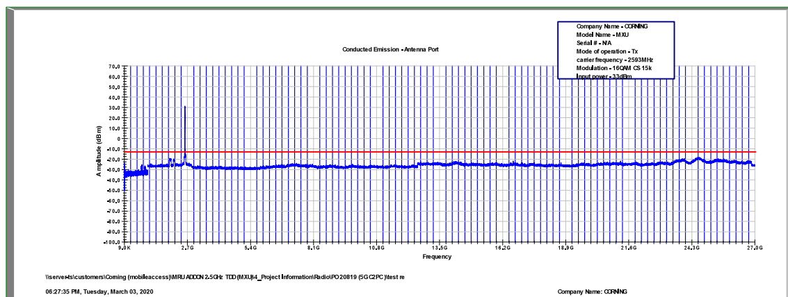
Figure 447: Spurious Emissions at Antenna Terminal 16QAM, 2593.0MHz, B.W. 10MHz, Sub Carrier 15kHz
