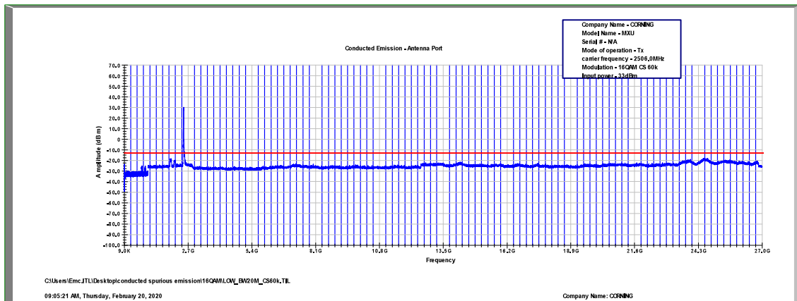
Figure 470: Spurious Emissions at Antenna Terminal 16QAM, 2506.0MHz, B.W. 20MHz, Sub Carrier 60kHz
