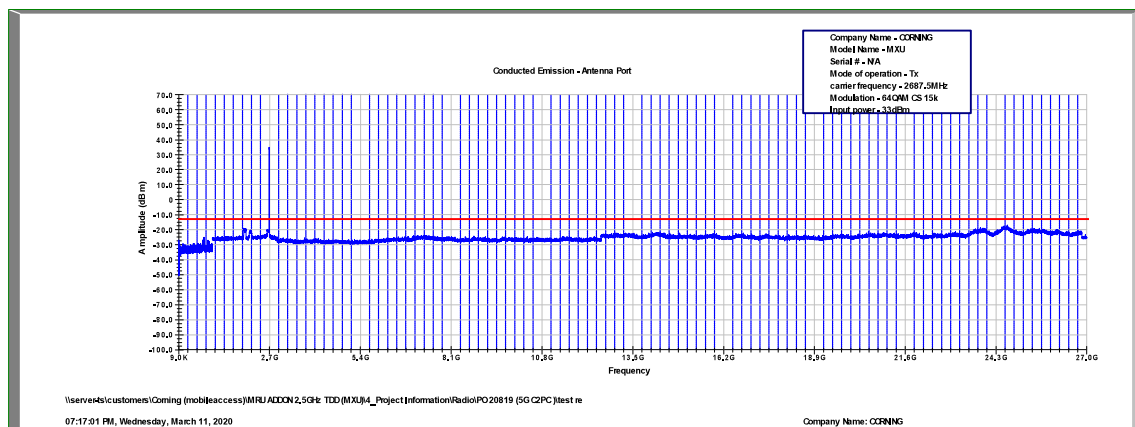
Figure 490: Spurious Emissions at Antenna Terminal 64QAM, 2887.5MHz, B.W. 5MHz, Sub Carrier 15kHz
