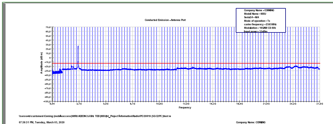
Figure 480: Spurious Emissions at Antenna Terminal 16QAM, 2593.0MHz, B.W. 40MHz, Sub Carrier 60kHz
