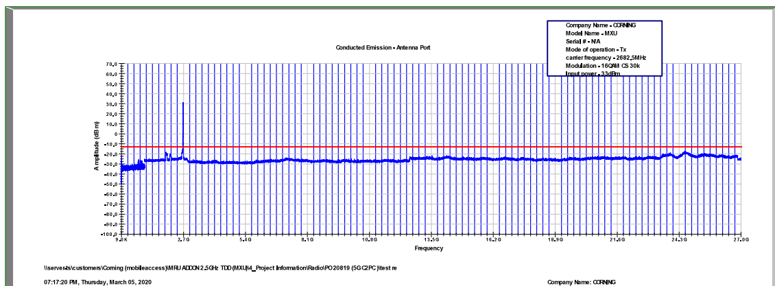
Figure 460: Spurious Emissions at Antenna Terminal 16QAM, 2682.5MHz, B.W. 15MHz, Sub Carrier 30kHz
