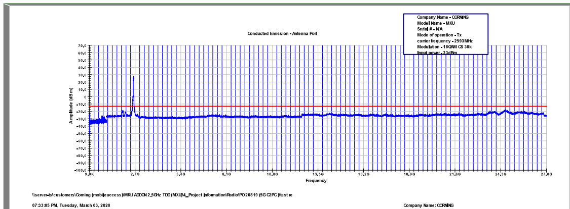
Figure 477: Spurious Emissions at Antenna Terminal 16QAM, 2593.0MHz, B.W. 40MHz, Sub Carrier 30kHz
