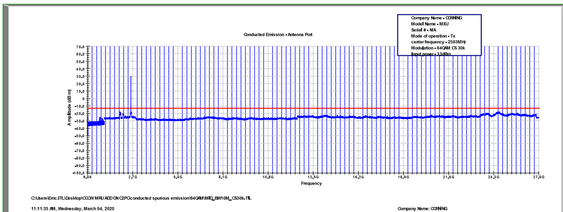
Figure 498: Spurious Emissions at Antenna Terminal 64QAM, 2593.0MHz, B.W. 10MHz, Sub Carrier 30kHz
