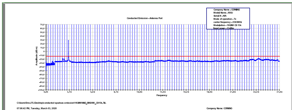
Figure 465: Spurious Emissions at Antenna Terminal 16QAM, 2593.0MHz, B.W. 20MHz, Sub Carrier 15kHz
