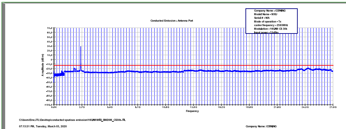
Figure 468: Spurious Emissions at Antenna Terminal 16QAM, 2593.0MHz, B.W. 20MHz, Sub Carrier 30kHz
