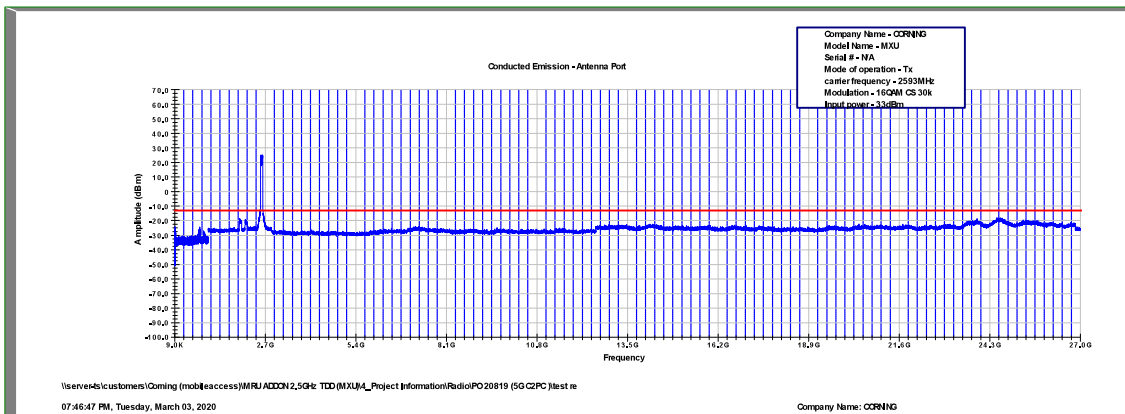
Figure 483: Spurious Emissions at Antenna Terminal 16QAM, 2593.0MHz, B.W. 60MHz, Sub Carrier 30kHz
