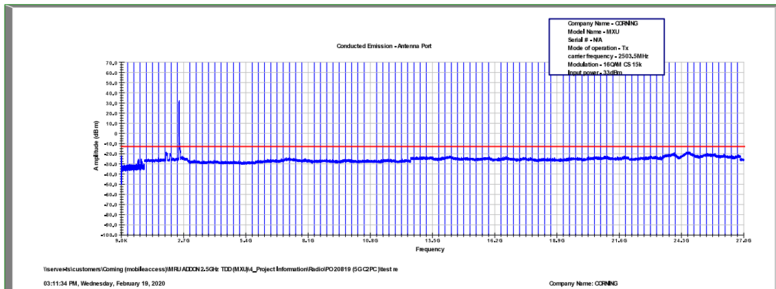
Figure 455: Spurious Emissions at Antenna Terminal 16QAM, 2503.5MHz, B.W. 15MHz, Sub Carrier 15kHz
