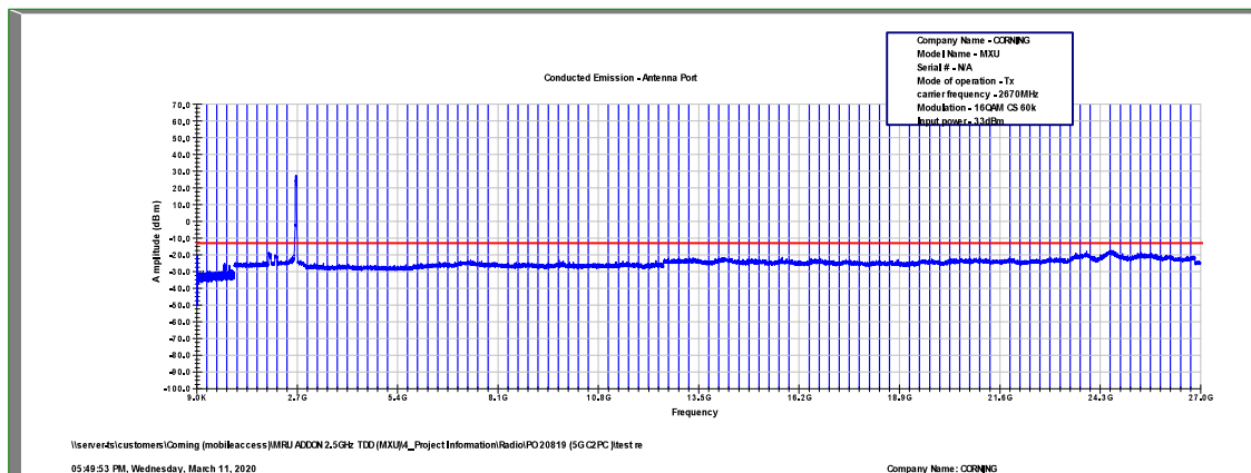
Figure 481: Spurious Emissions at Antenna Terminal 16QAM, 2670.0MHz, B.W. 40MHz, Sub Carrier 60kHz
