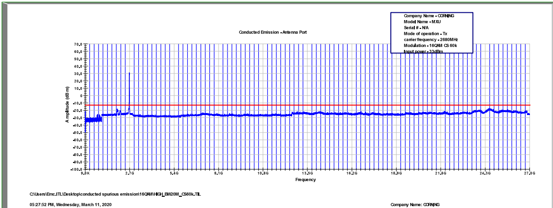
Figure 472: Spurious Emissions at Antenna Terminal 16QAM, 2680.0MHz, B.W. 20MHz, Sub Carrier 60kHz
