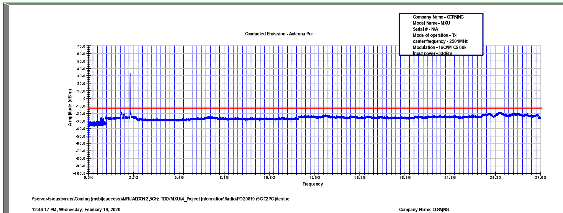
Figure 452: Spurious Emissions at Antenna Terminal 16QAM, 2501.0MHz, B.W. 10MHz, Sub Carrier 60kHz
