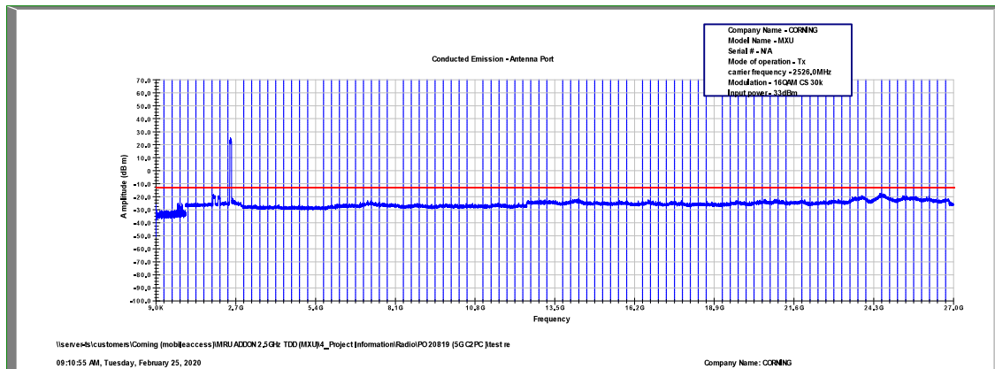
Figure 482: Spurious Emissions at Antenna Terminal 16QAM, 2526.0MHz, B.W. 60MHz, Sub Carrier 30kHz
