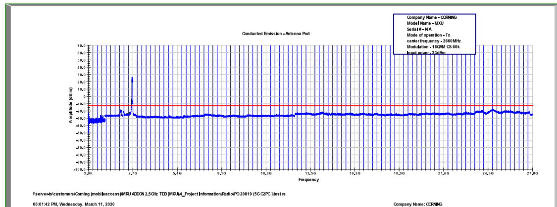
Figure 487: Spurious Emissions at Antenna Terminal 16QAM, 2660.0MHz, B.W. 60MHz, Sub Carrier 60kHz
