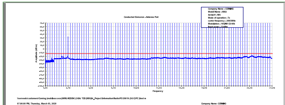
Figure 454: Spurious Emissions at Antenna Terminal 16QAM, 2685.0MHz, B.W. 10MHz, Sub Carrier 60kHz
