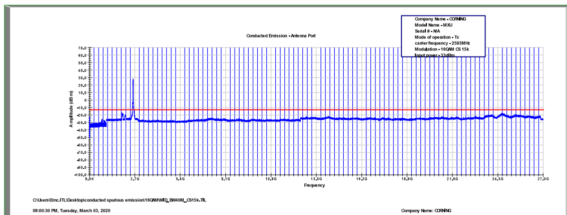
Figure 474: Spurious Emissions at Antenna Terminal 16QAM, 2593.0MHz, B.W. 40MHz, Sub Carrier 15kHz
