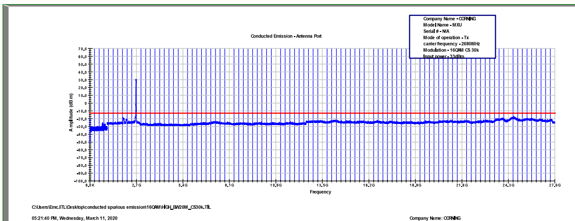
Figure 469: Spurious Emissions at Antenna Terminal 16QAM, 2680.0MHz, B.W. 20MHz, Sub Carrier 30kHz
