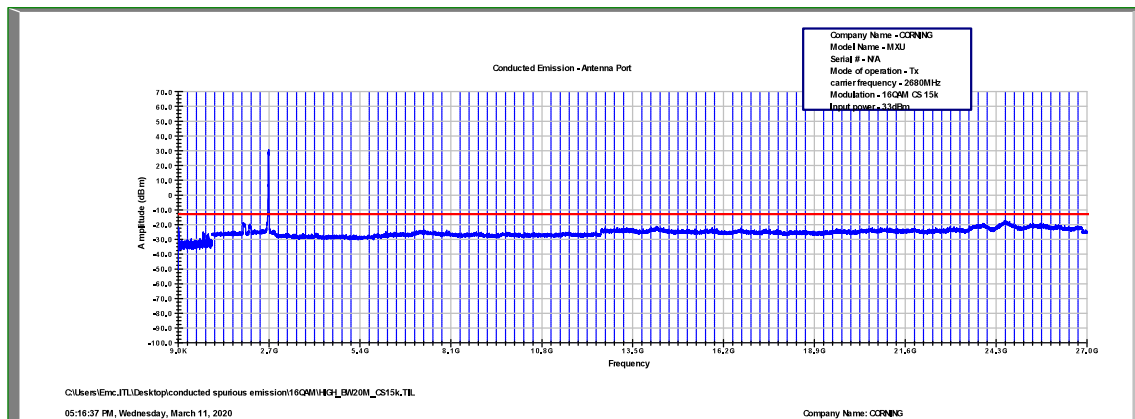
Figure 466: Spurious Emissions at Antenna Terminal 16QAM, 2680.0MHz, B.W. 20MHz, Sub Carrier 15kHz
