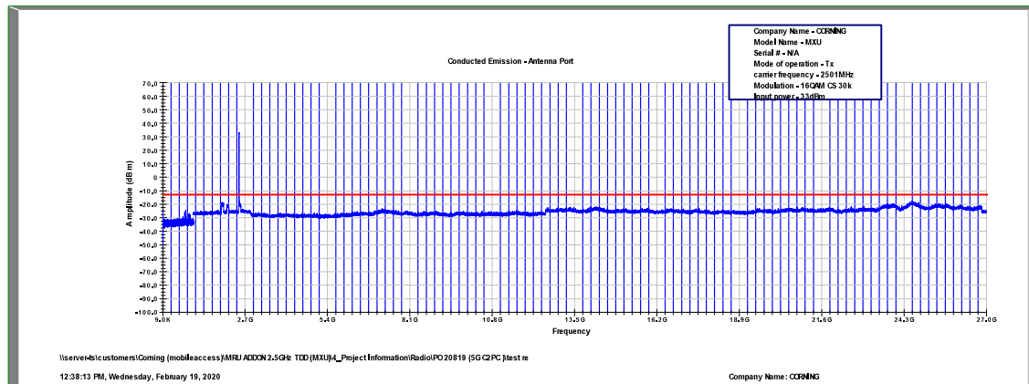
Figure 449: Spurious Emissions at Antenna Terminal 16QAM, 2501.0MHz, B.W. 10MHz, Sub Carrier 30kHz
