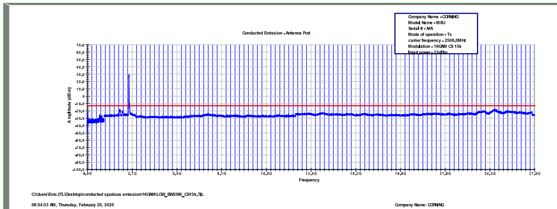
Figure 464: Spurious Emissions at Antenna Terminal 16QAM, 2506.0MHz, B.W. 20MHz, Sub Carrier 15kHz
