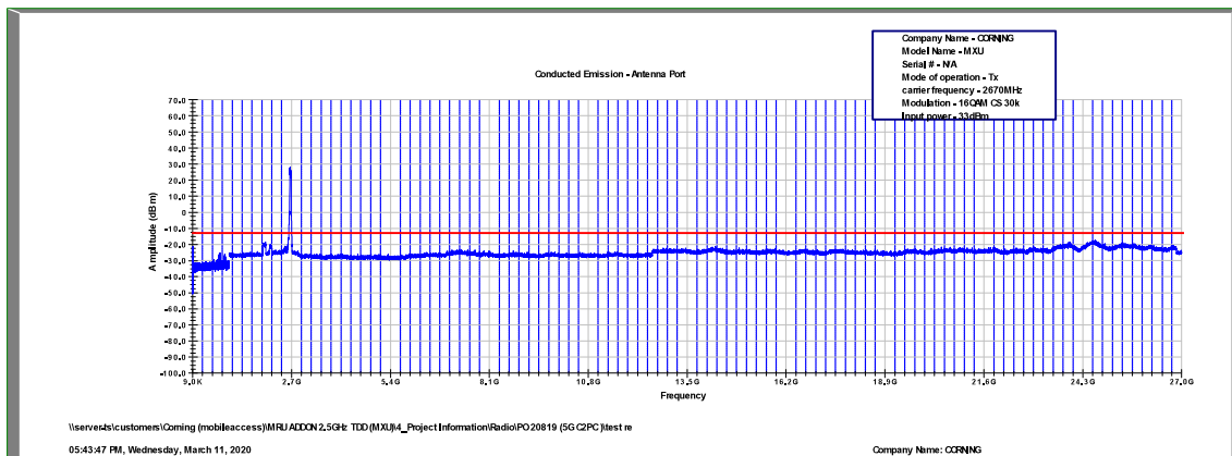
Figure 478: Spurious Emissions at Antenna Terminal 16QAM, 2670.0MHz, B.W. 40MHz, Sub Carrier 30kHz
