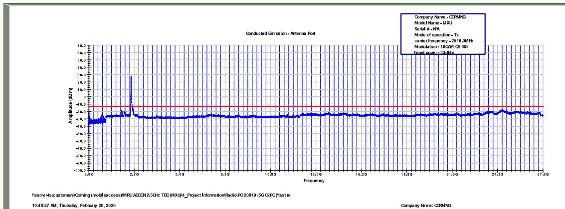
Figure 479: Spurious Emissions at Antenna Terminal 16QAM, 2516.0MHz, B.W. 40MHz, Sub Carrier 60kHz
