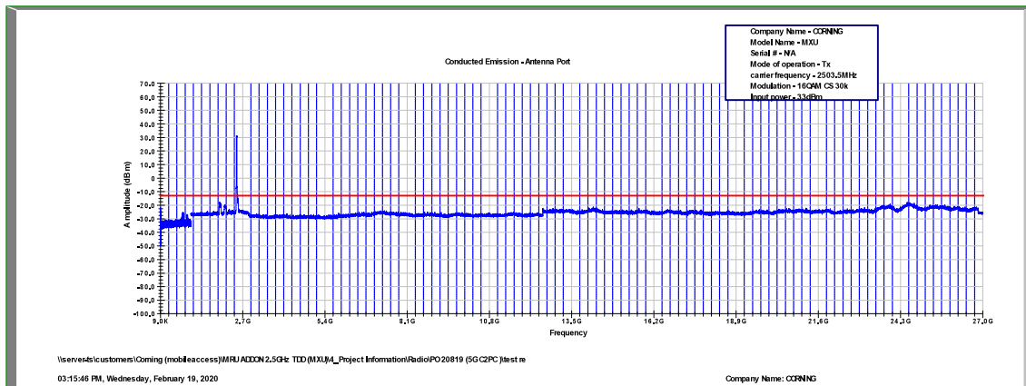
Figure 458: Spurious Emissions at Antenna Terminal 16QAM, 2503.5MHz, B.W. 15MHz, Sub Carrier 30kHz
