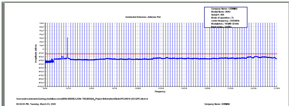
Figure 462: Spurious Emissions at Antenna Terminal 16QAM, 2593.0MHz, B.W. 15MHz, Sub Carrier 60kHz
