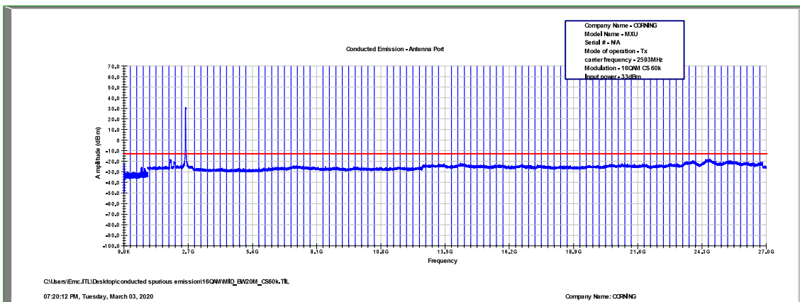
Figure 471: Spurious Emissions at Antenna Terminal 16QAM, 2593.0MHz, B.W. 20MHz, Sub Carrier 60kHz
