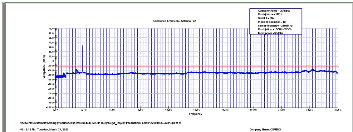
Figure 444: Spurious Emissions at Antenna Terminal 16QAM, 2593.0MHz, B.W. 5MHz, Sub Carrier 30kHz
