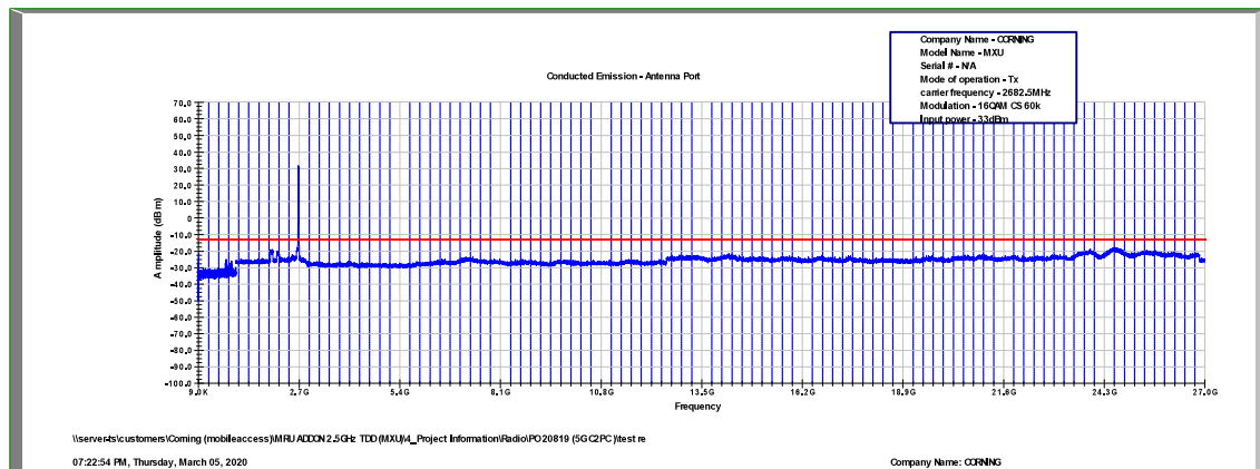
Figure 463: Spurious Emissions at Antenna Terminal 16QAM, 2682.5MHz, B.W. 15MHz, Sub Carrier 60kHz
