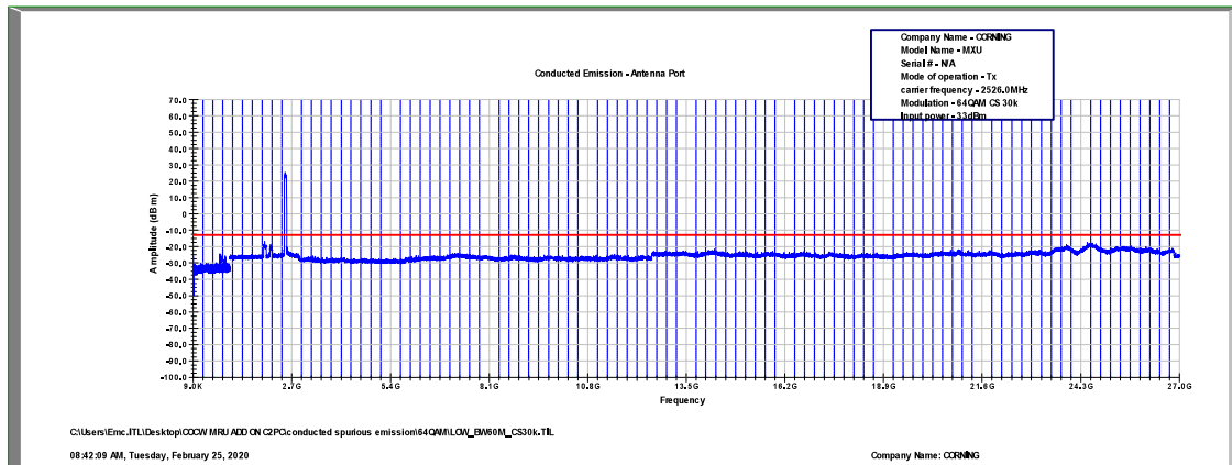
Figure 530: Spurious Emissions at Antenna Terminal 64QAM, 2526.0MHz, B.W. 60MHz, Sub Carrier 30kHz
