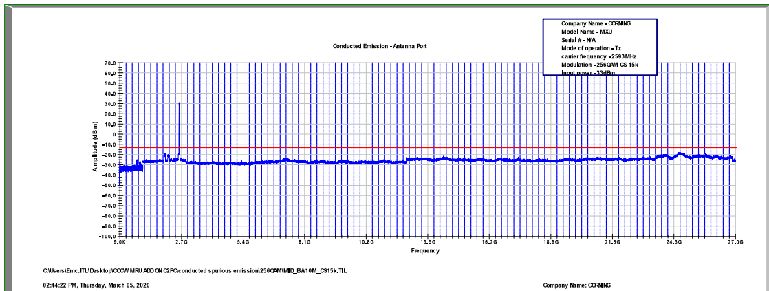
Figure 543: Spurious Emissions at Antenna Terminal 256QAM, 2593.0MHz, B.W. 10MHz, Sub Carrier 15kHz
